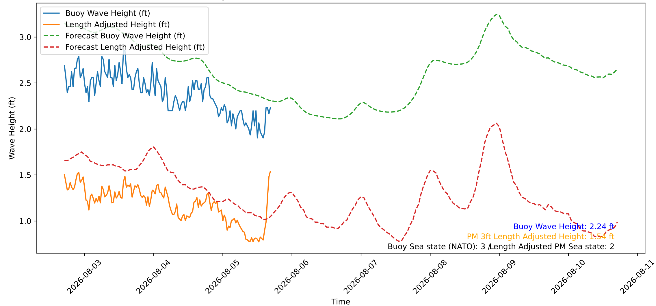
Wave Heights over Time for Oceanside Harbor at 2026-08-05 17:10:26
