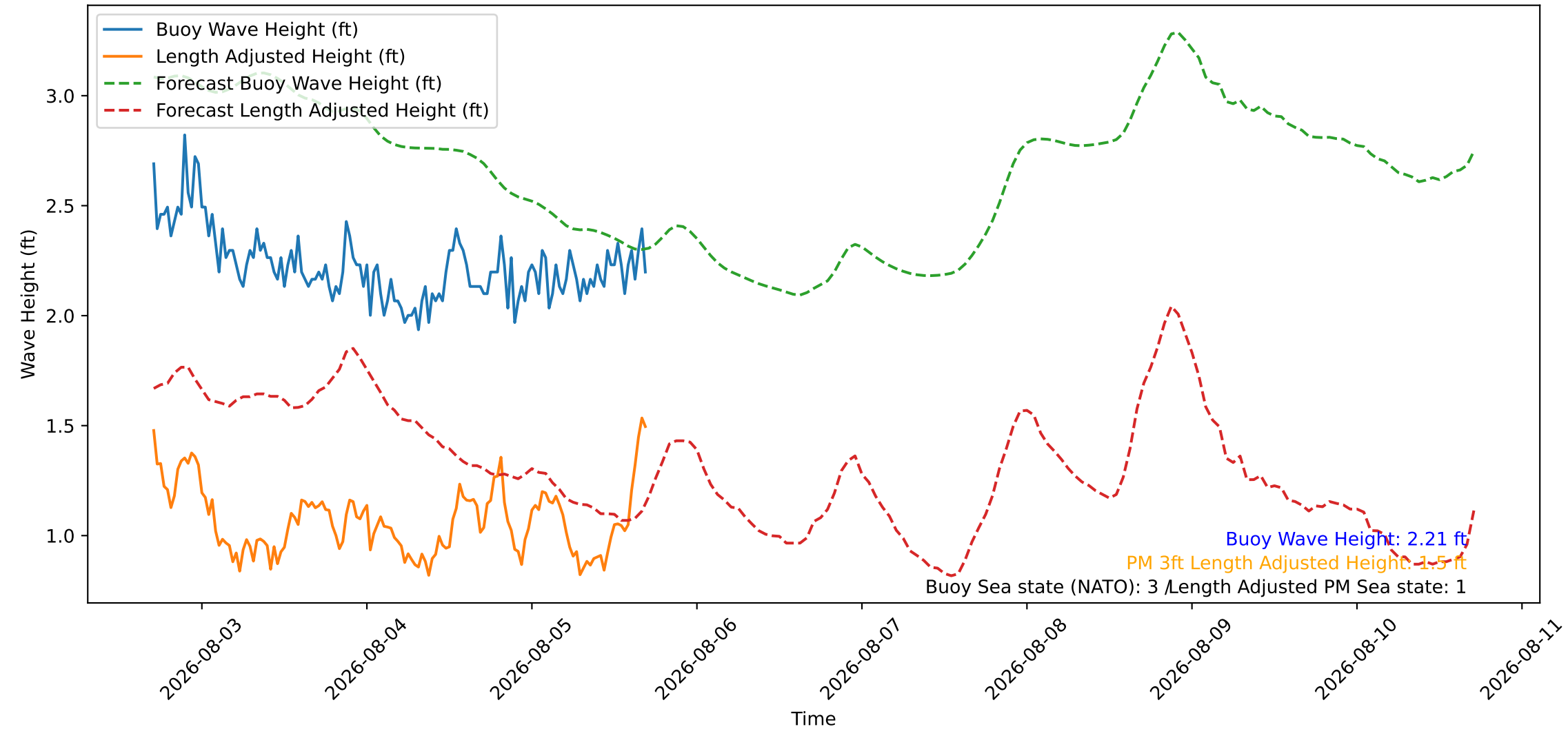
Wave Heights over Time for Green Beach at 2026-08-05 17:11:07
