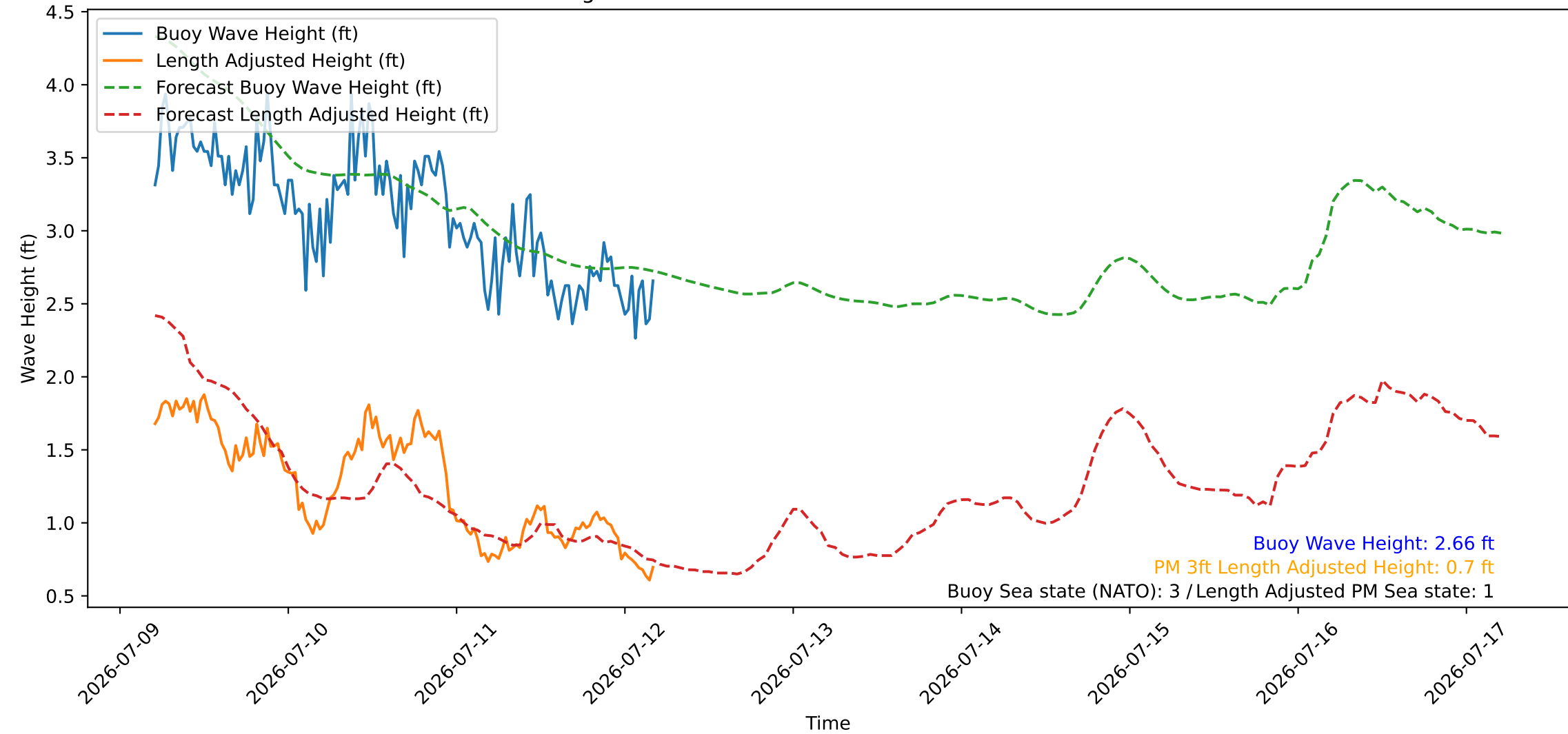
Wave Heights over Time for Red Beach at 2026-07-12 04:50:47
