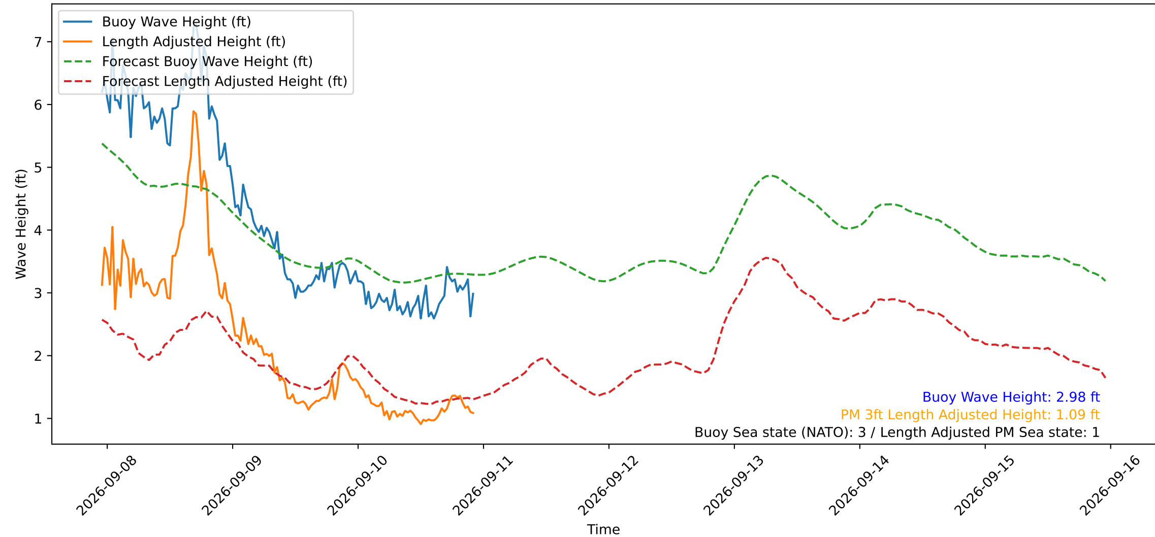
Wave Heights over Time for Green Beach at 2026-09-10 22:51:14
