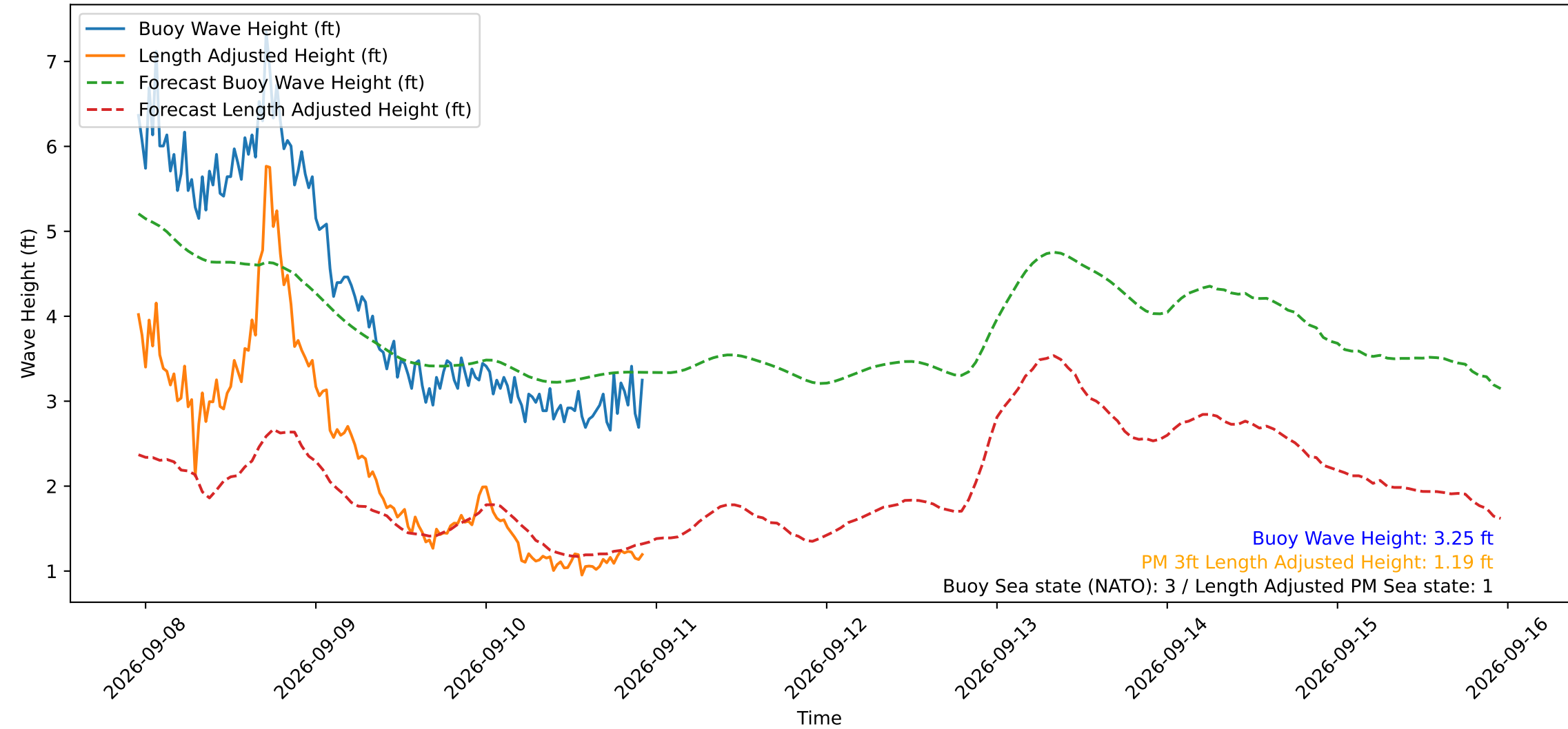
Wave Heights over Time for Oceanside Harbor at 2026-09-10 22:50:29
