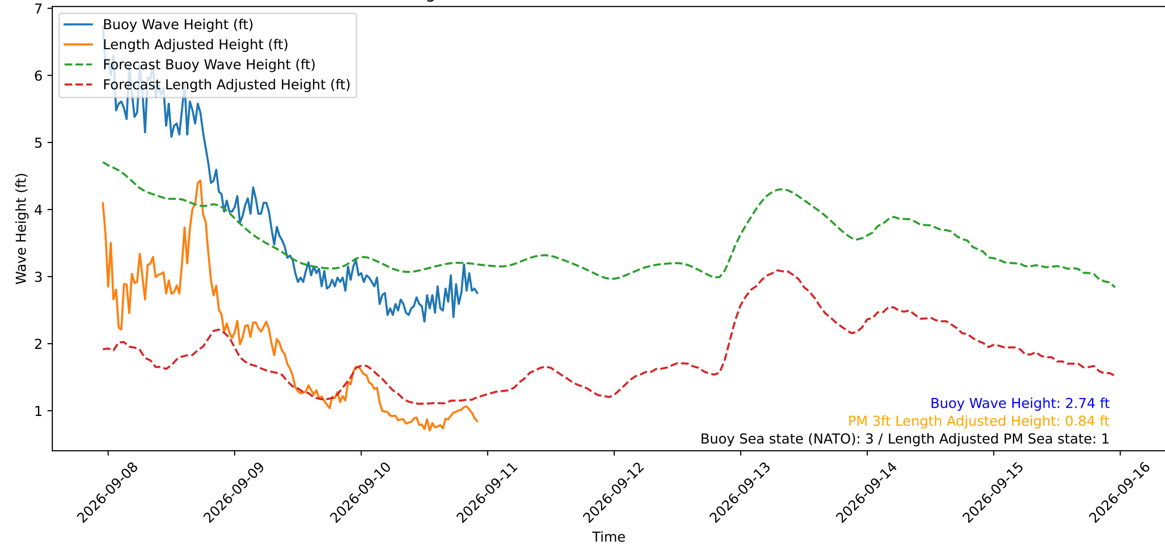
Wave Heights over Time for Red Beach at 2026-09-10 22:50:51
