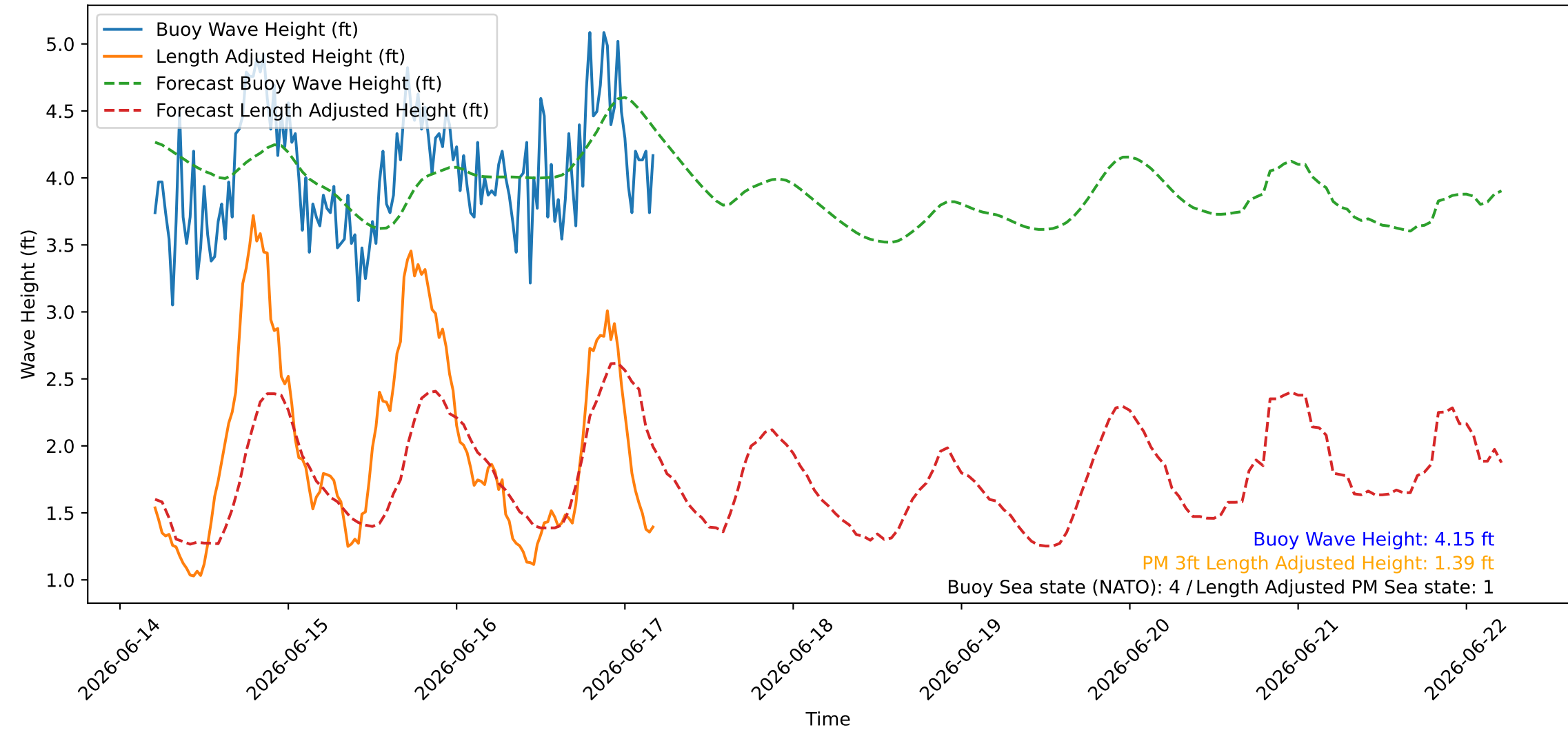
Wave Heights over Time for Green Beach at 2026-06-17 04:51:10
