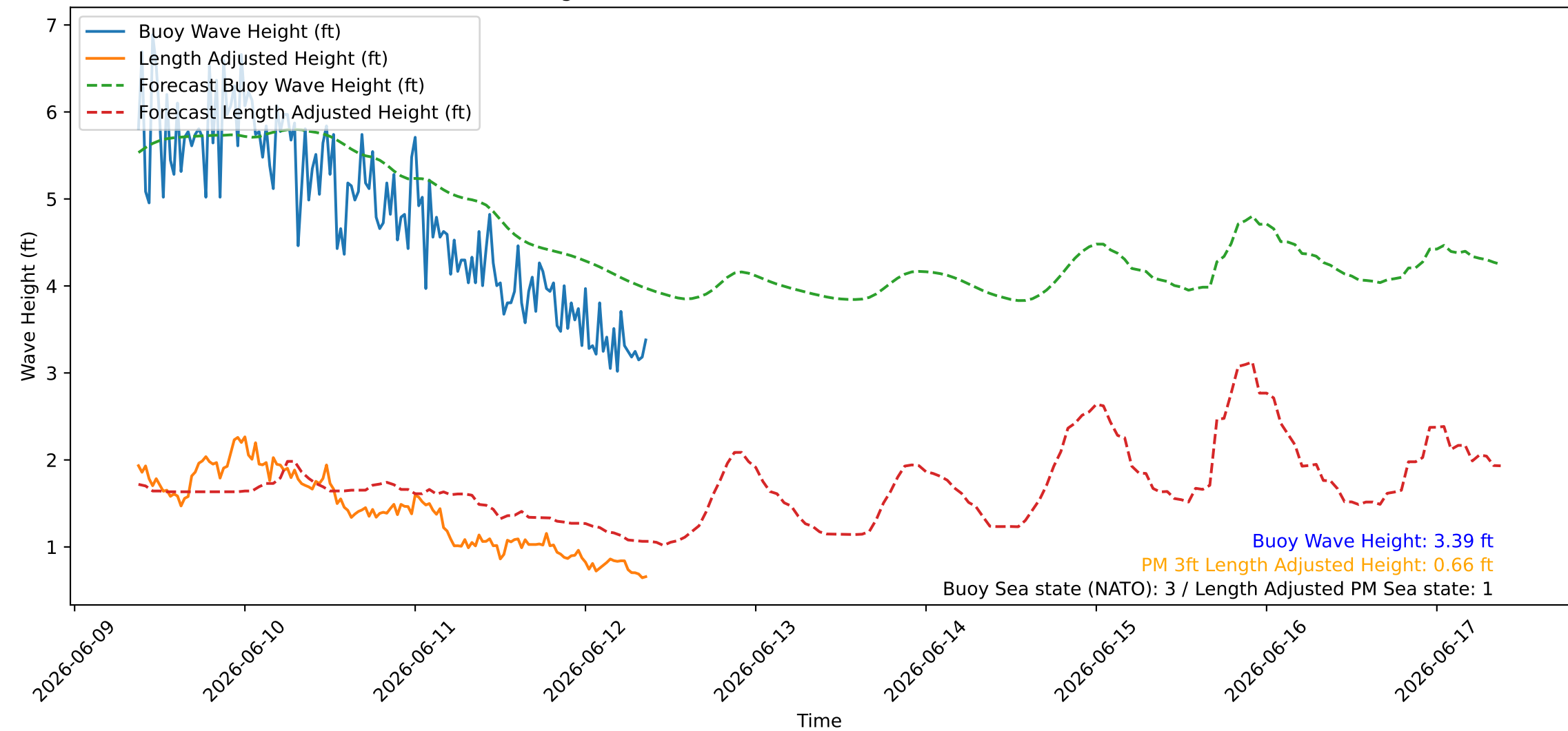
Wave Heights over Time for Green Beach at 2026-06-12 09:11:09
