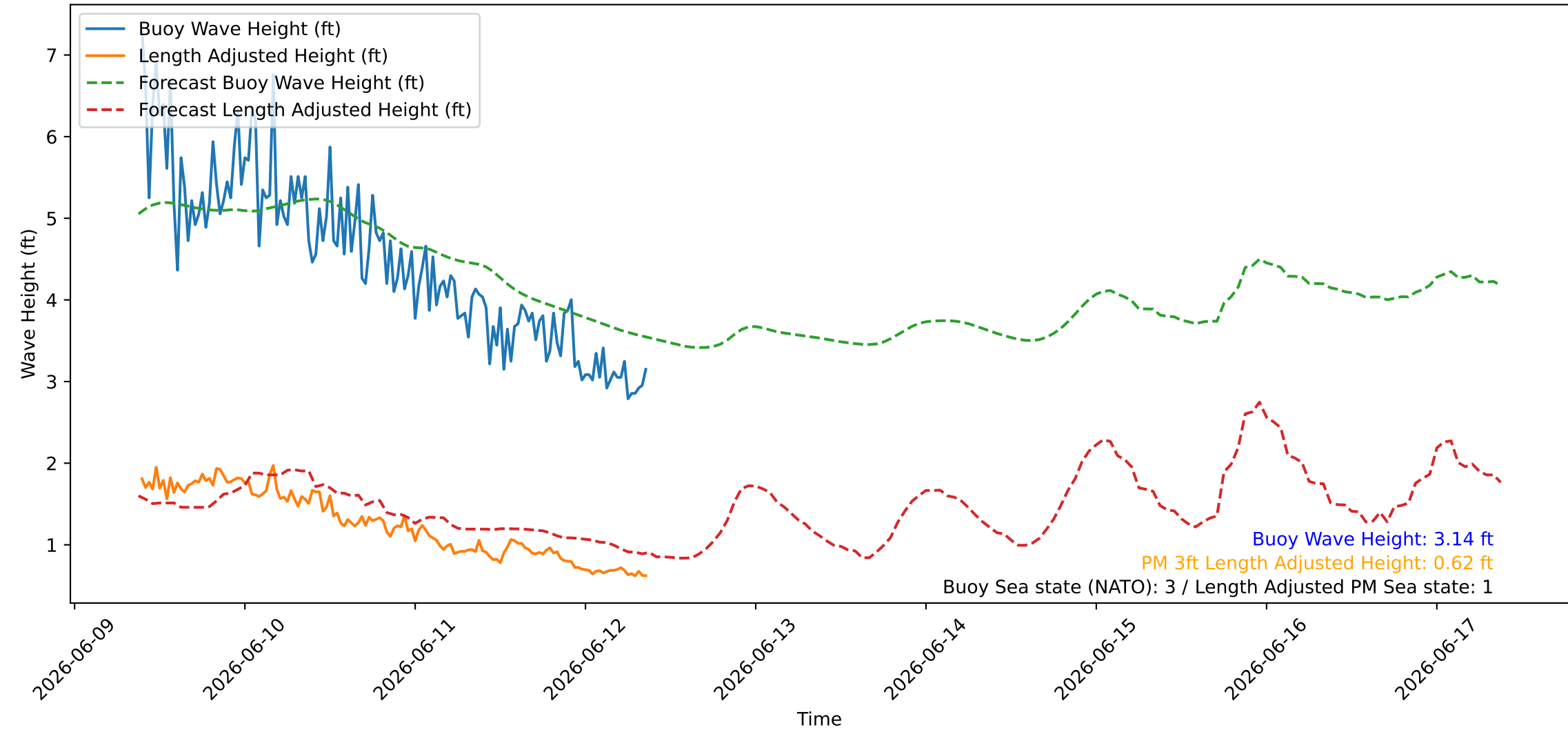
Wave Heights over Time for Red Beach at 2026-06-12 09:10:46
