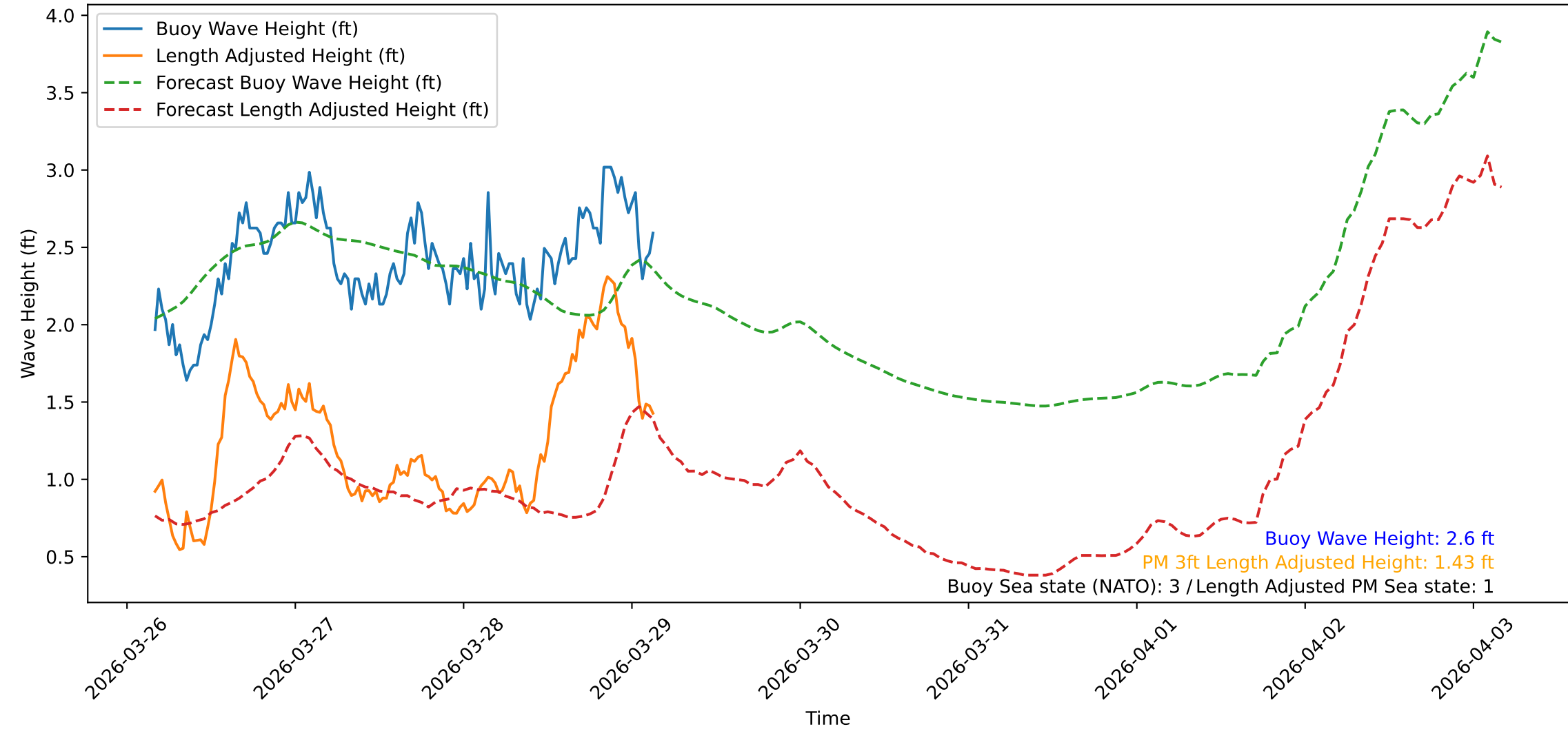
Wave Heights over Time for Red Beach at 2026-03-29 03:50:47
