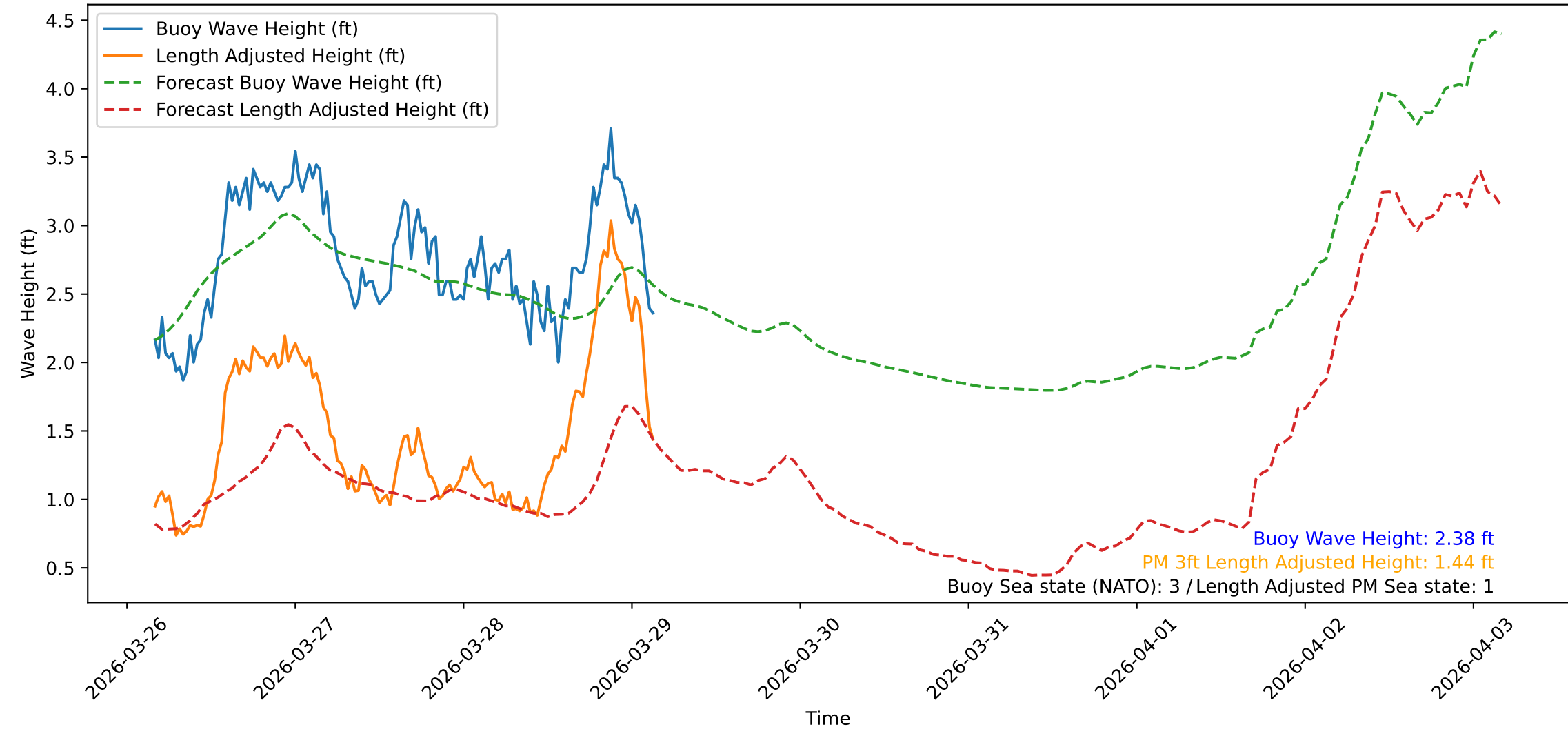
Wave Heights over Time for Green Beach at 2026-03-29 03:51:09
