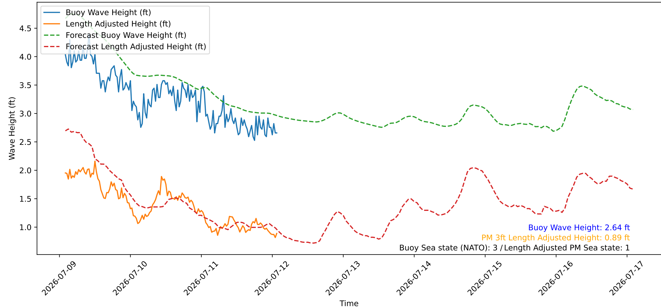
Wave Heights over Time for Green Beach at 2026-07-12 02:11:08
