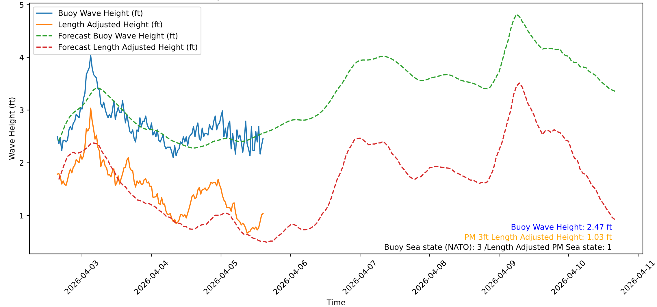
Wave Heights over Time for Oceanside Harbor at 2026-04-05 15:40:32
