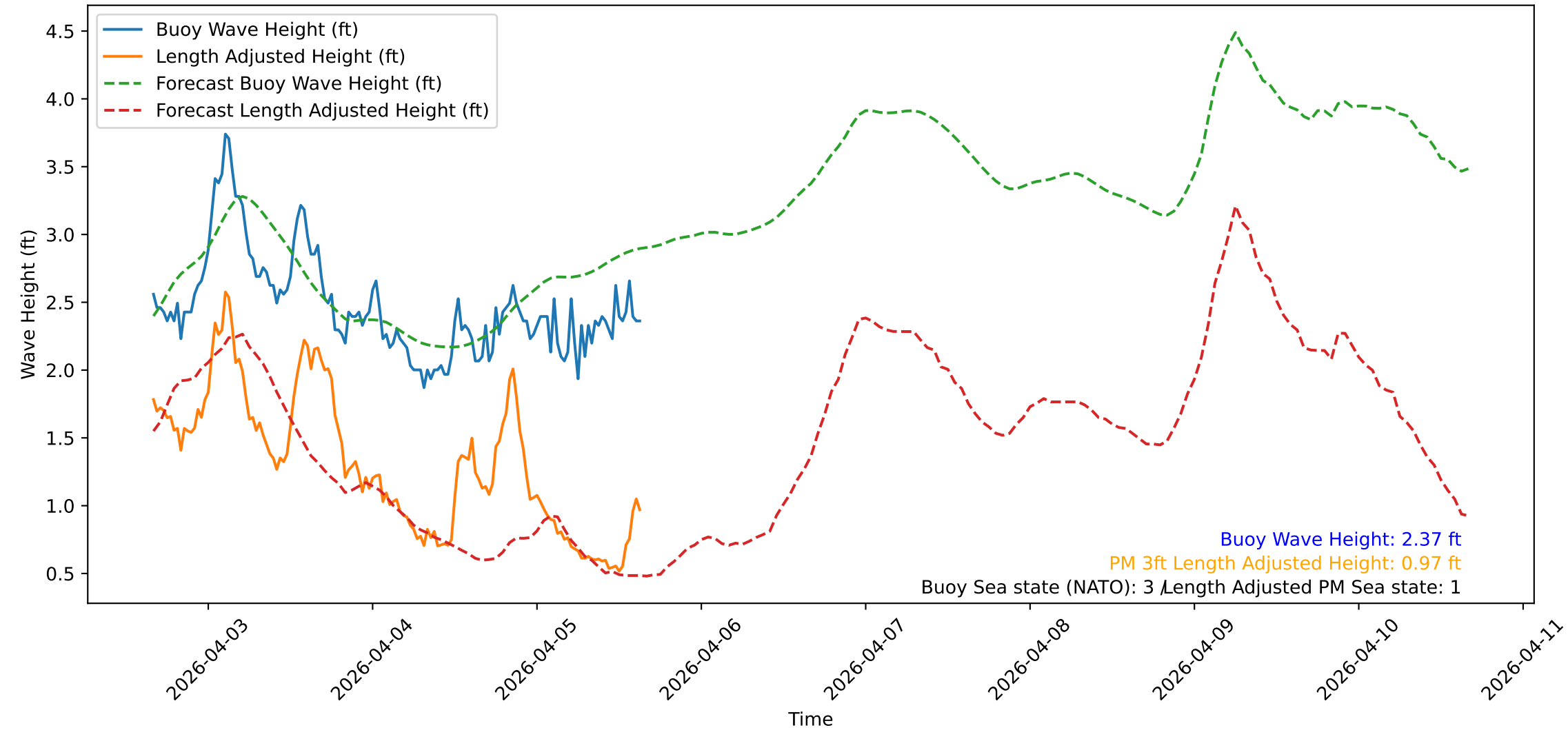
Wave Heights over Time for Red Beach at 2026-04-05 15:40:49
