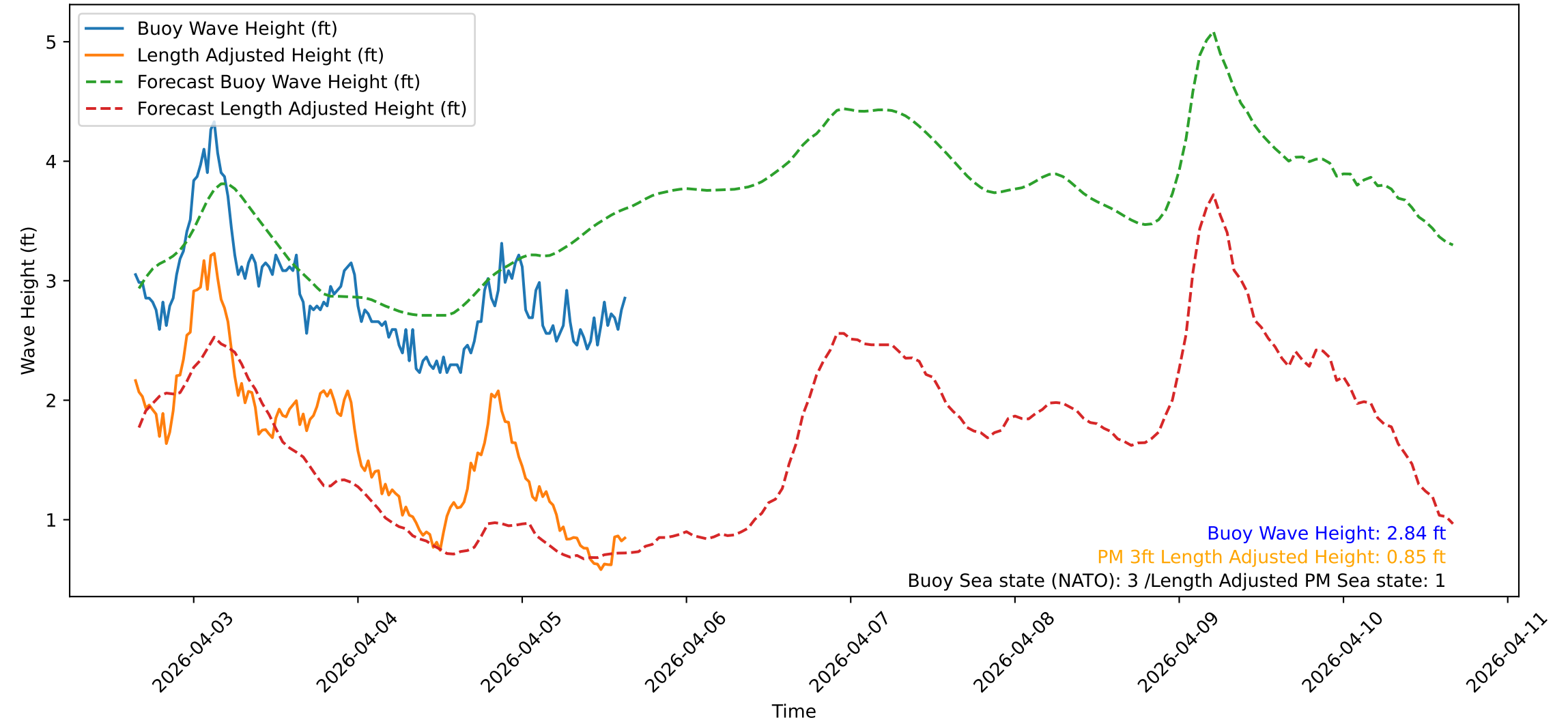
Wave Heights over Time for Green Beach at 2026-04-05 15:41:12
