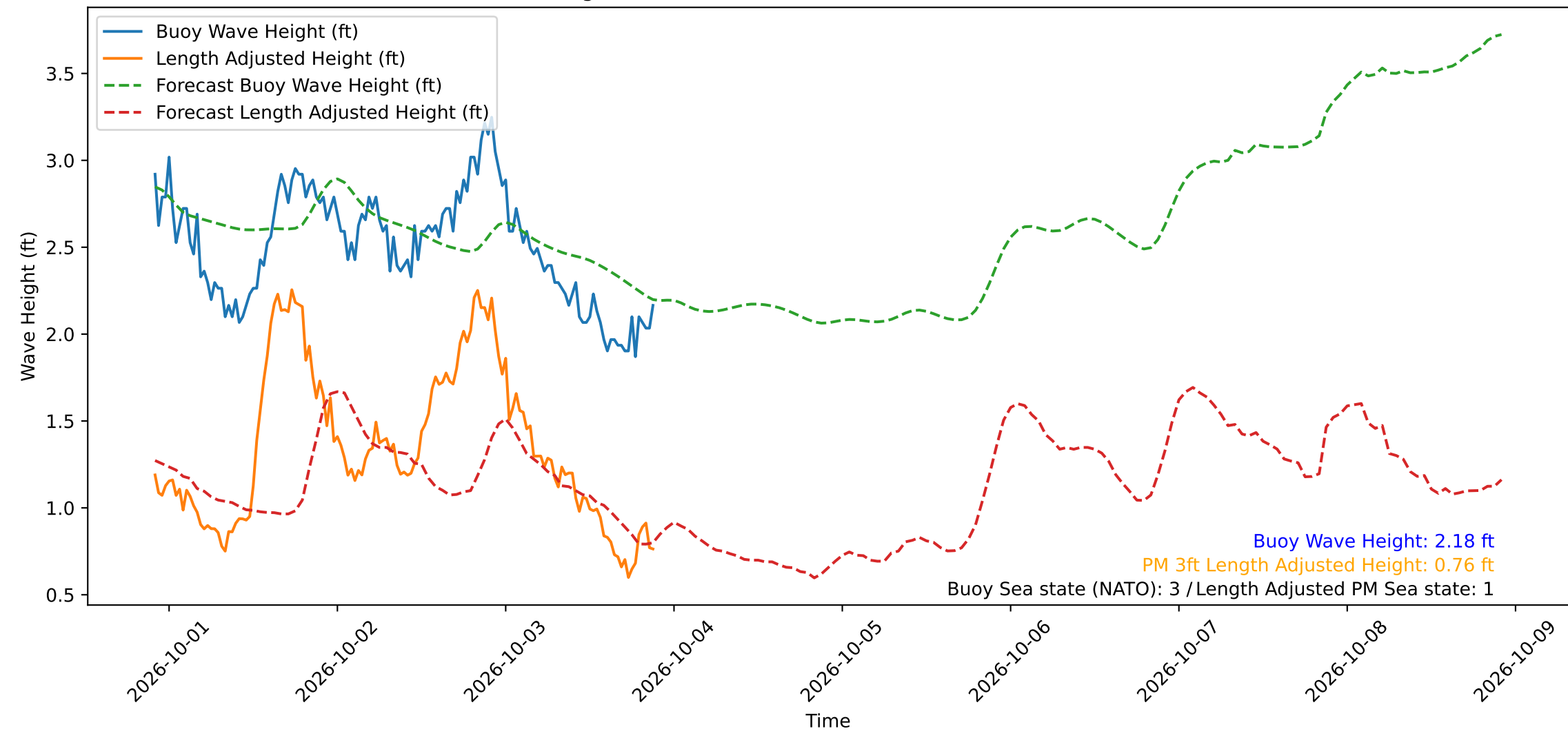
Wave Heights over Time for Red Beach at 2026-10-03 21:50:51
