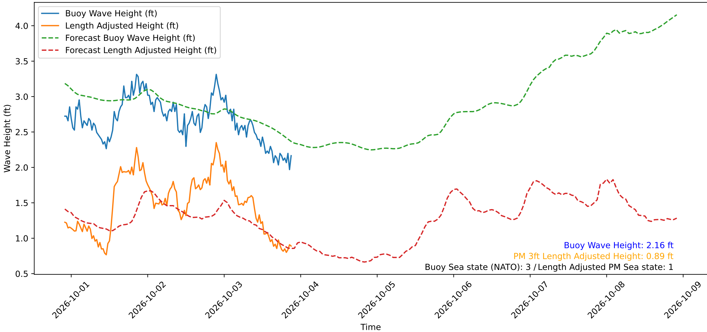
Wave Heights over Time for Oceanside Harbor at 2026-10-03 21:50:30
