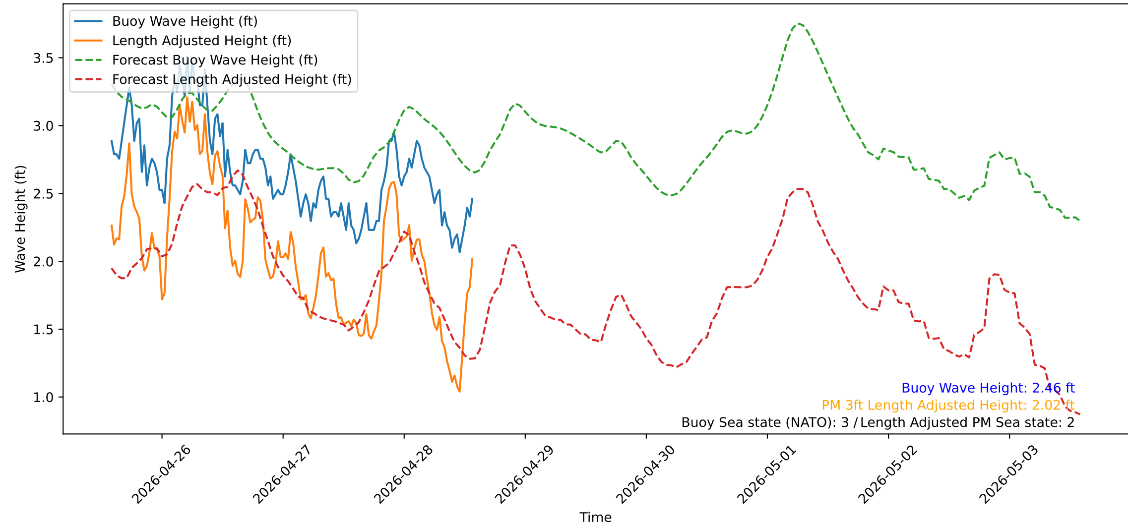
Wave Heights over Time for Green Beach at 2026-04-28 14:11:14
