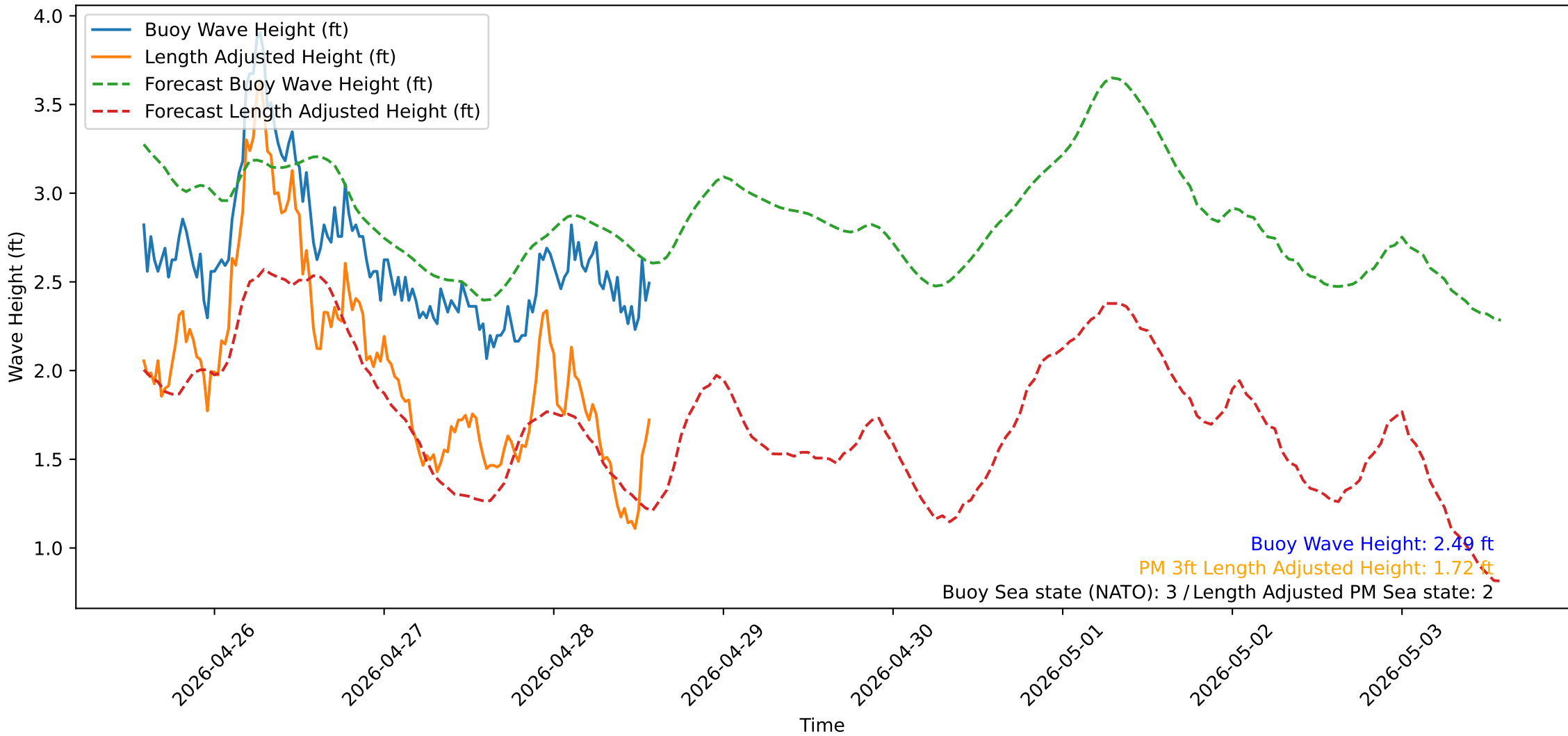
Wave Heights over Time for Oceanside Harbor at 2026-04-28 14:10:31
