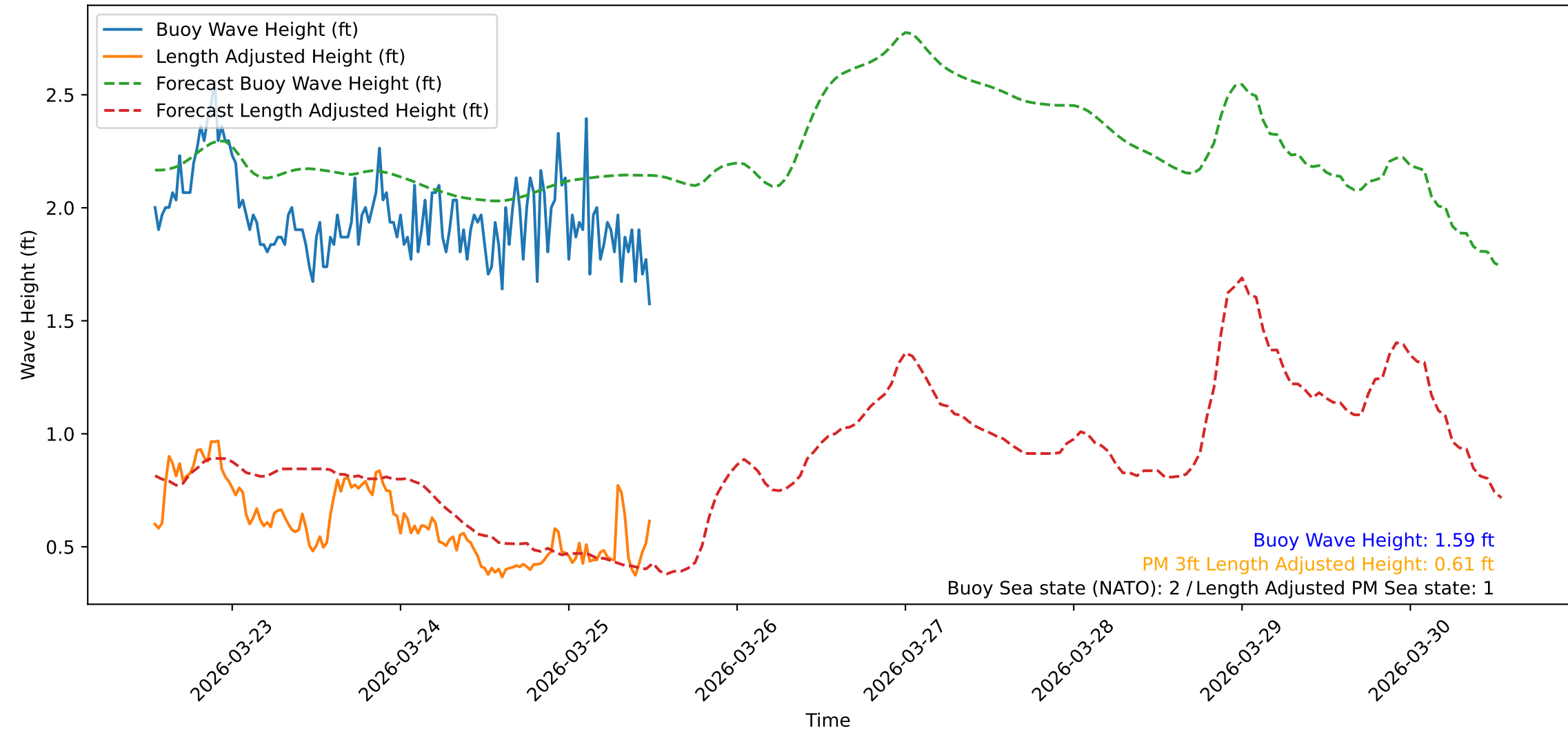
Wave Heights over Time for Red Beach at 2026-03-25 12:30:48
