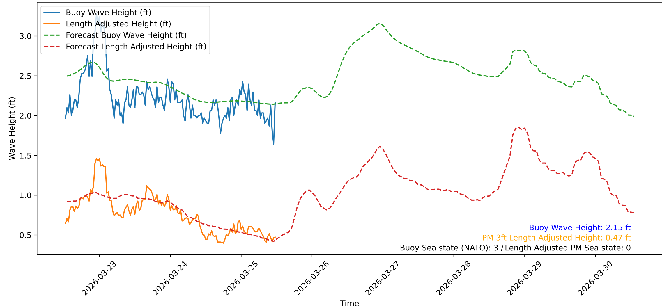
Wave Heights over Time for Green Beach at 2026-03-25 12:31:10
