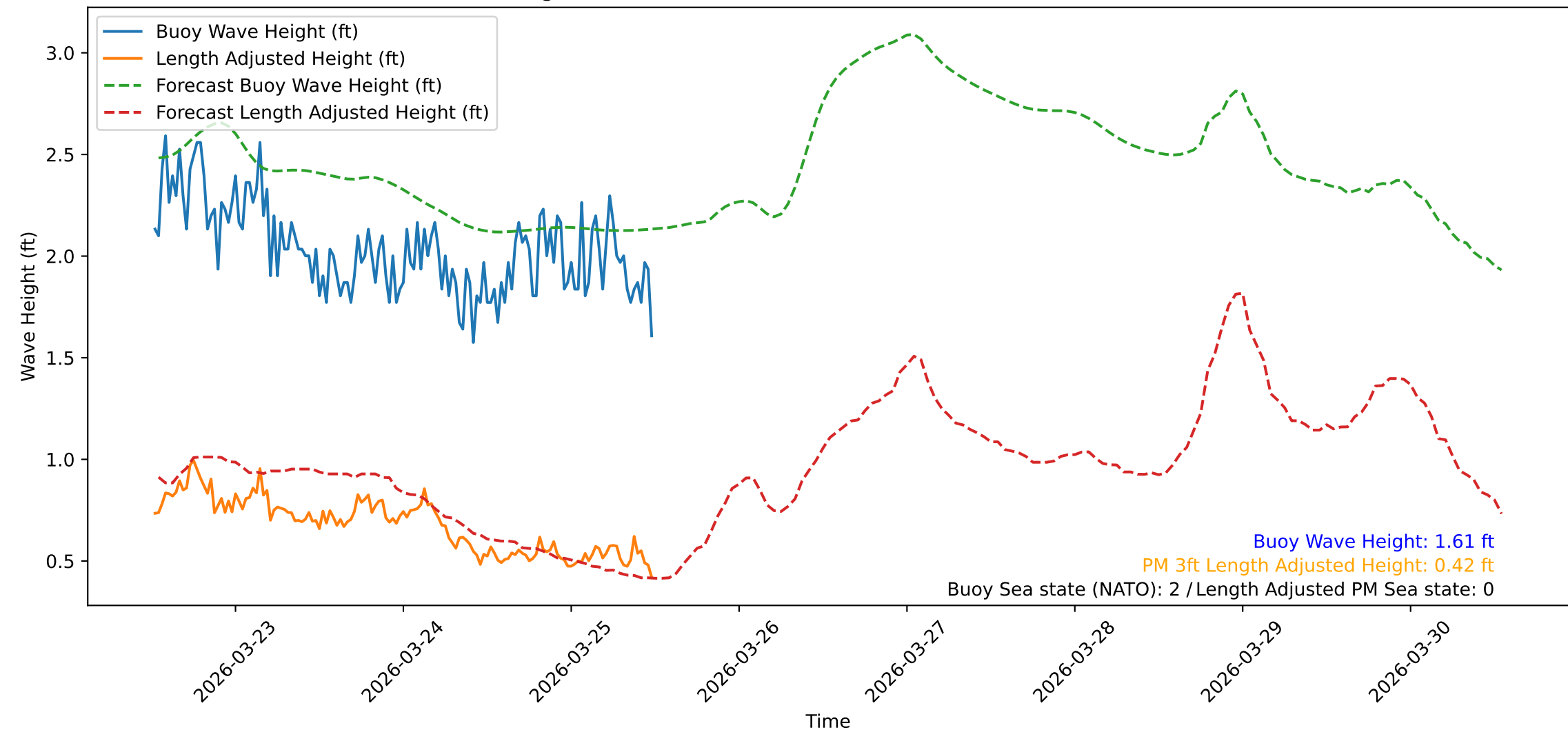
Wave Heights over Time for Oceanside Harbor at 2026-03-25 12:30:32
