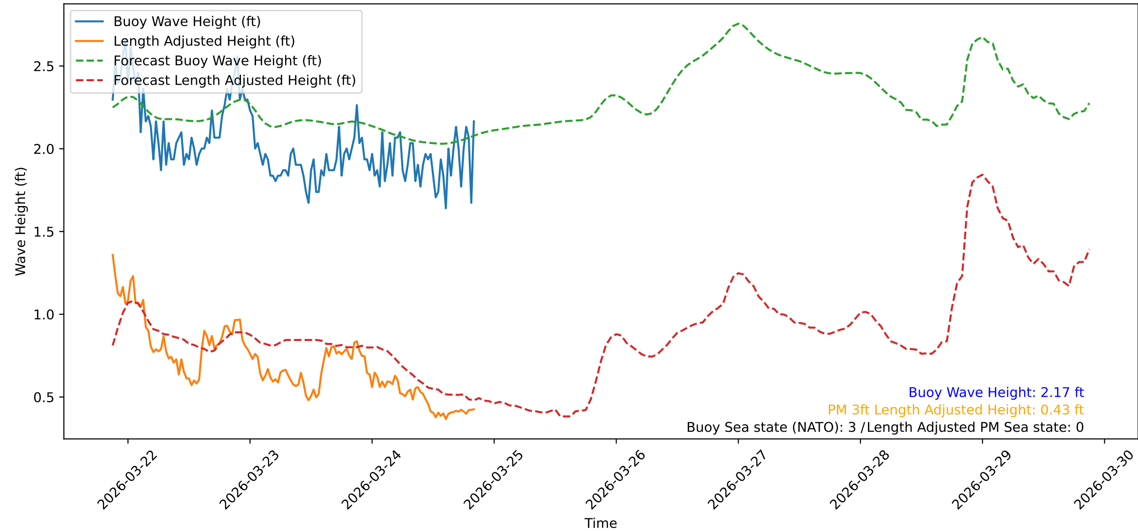
Wave Heights over Time for Red Beach at 2026-03-24 20:40:47
