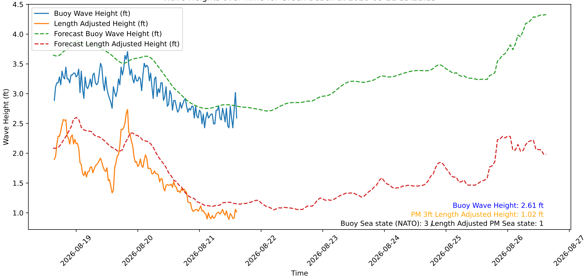
Wave Heights over Time for Green Beach at 2026-08-21 15:21:13
