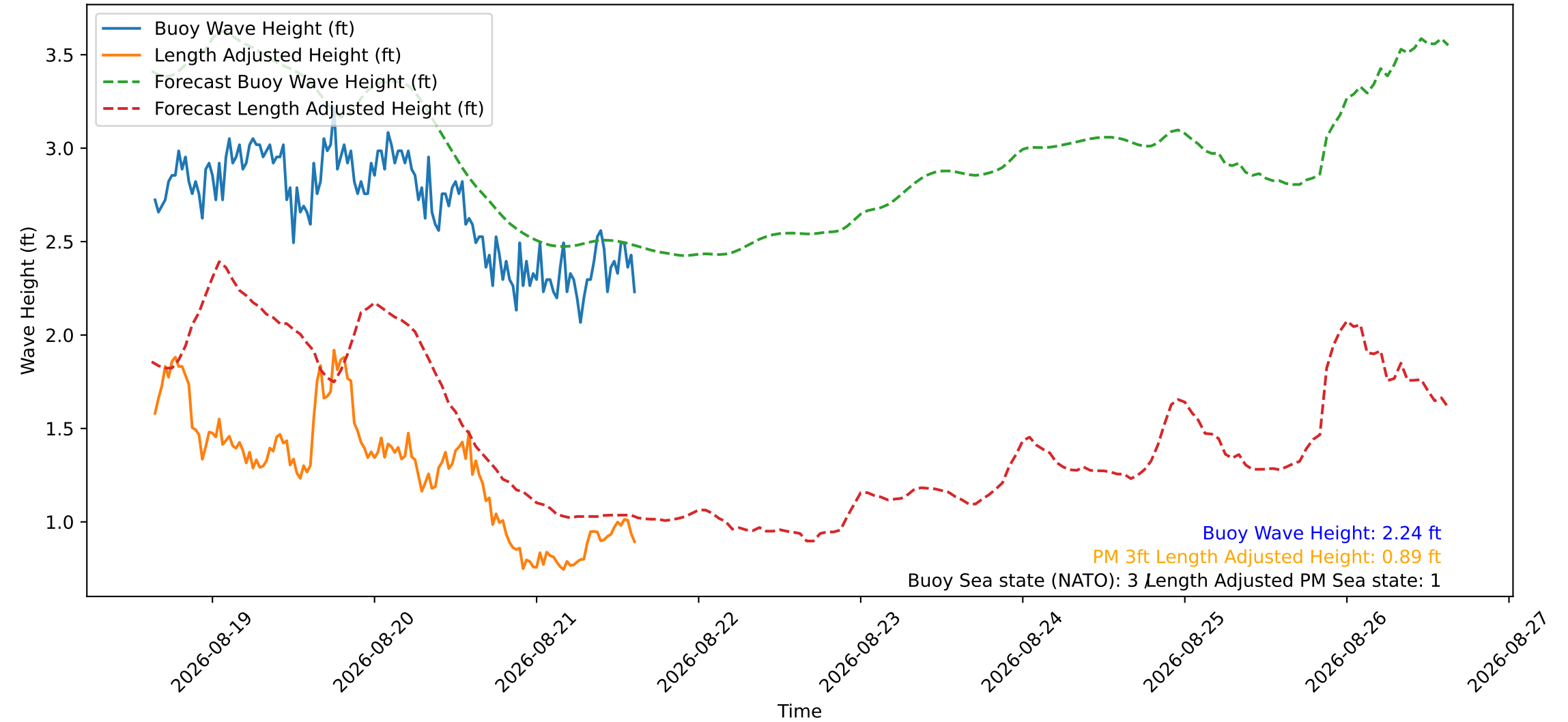
Wave Heights over Time for Red Beach at 2026-08-21 15:20:48
