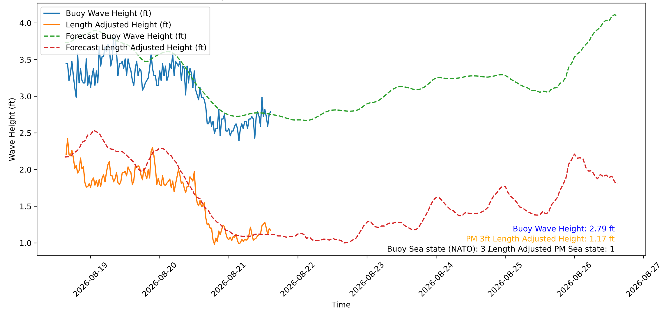
Wave Heights over Time for Oceanside Harbor at 2026-08-21 15:20:26
