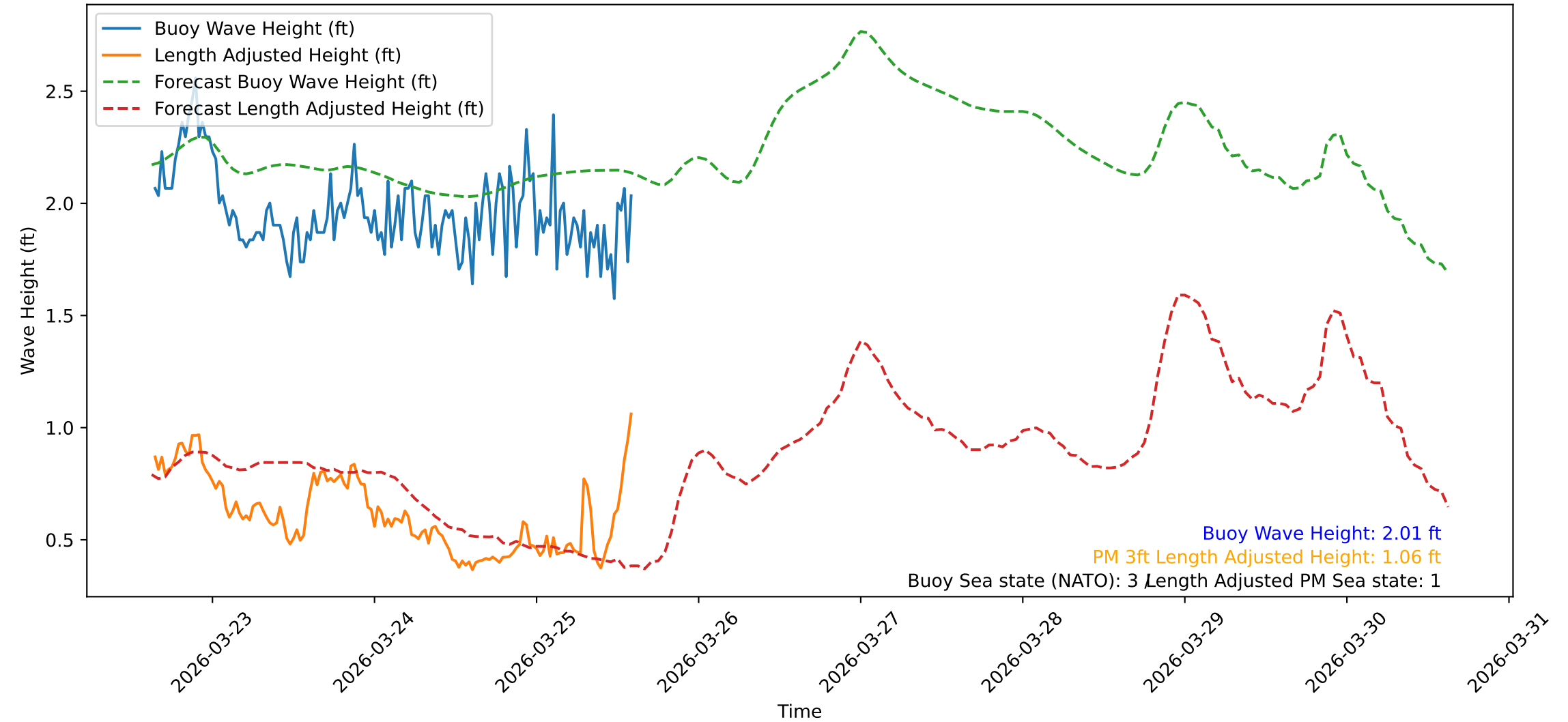
Wave Heights over Time for Red Beach at 2026-03-25 15:00:47
