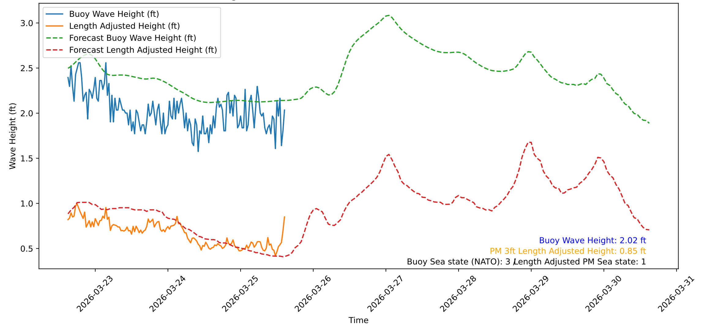
Wave Heights over Time for Oceanside Harbor at 2026-03-25 15:00:31
