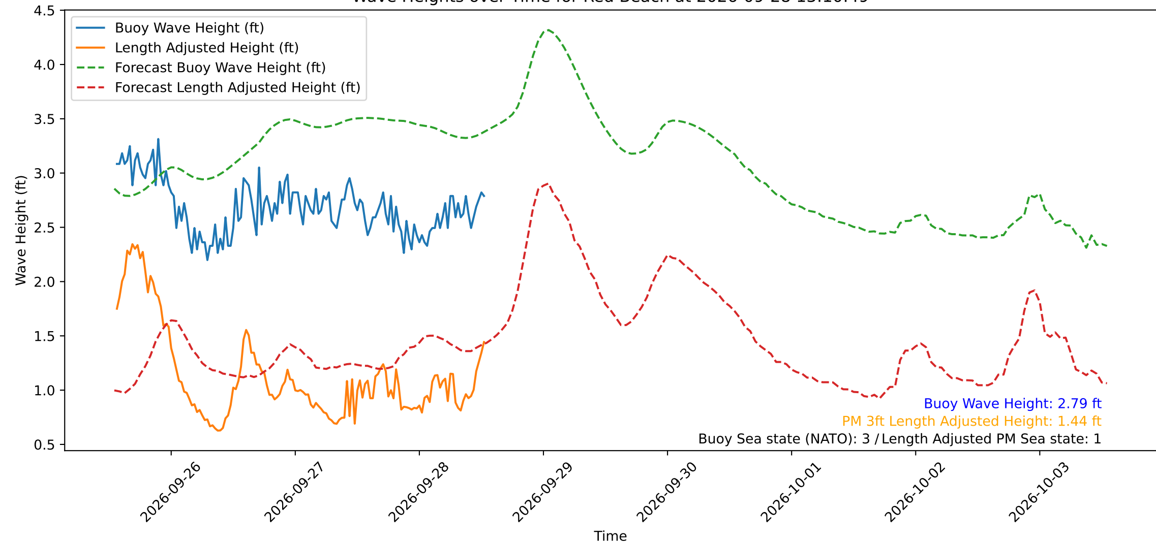
Wave Heights over Time for Red Beach at 2026-09-28 13:10:49
