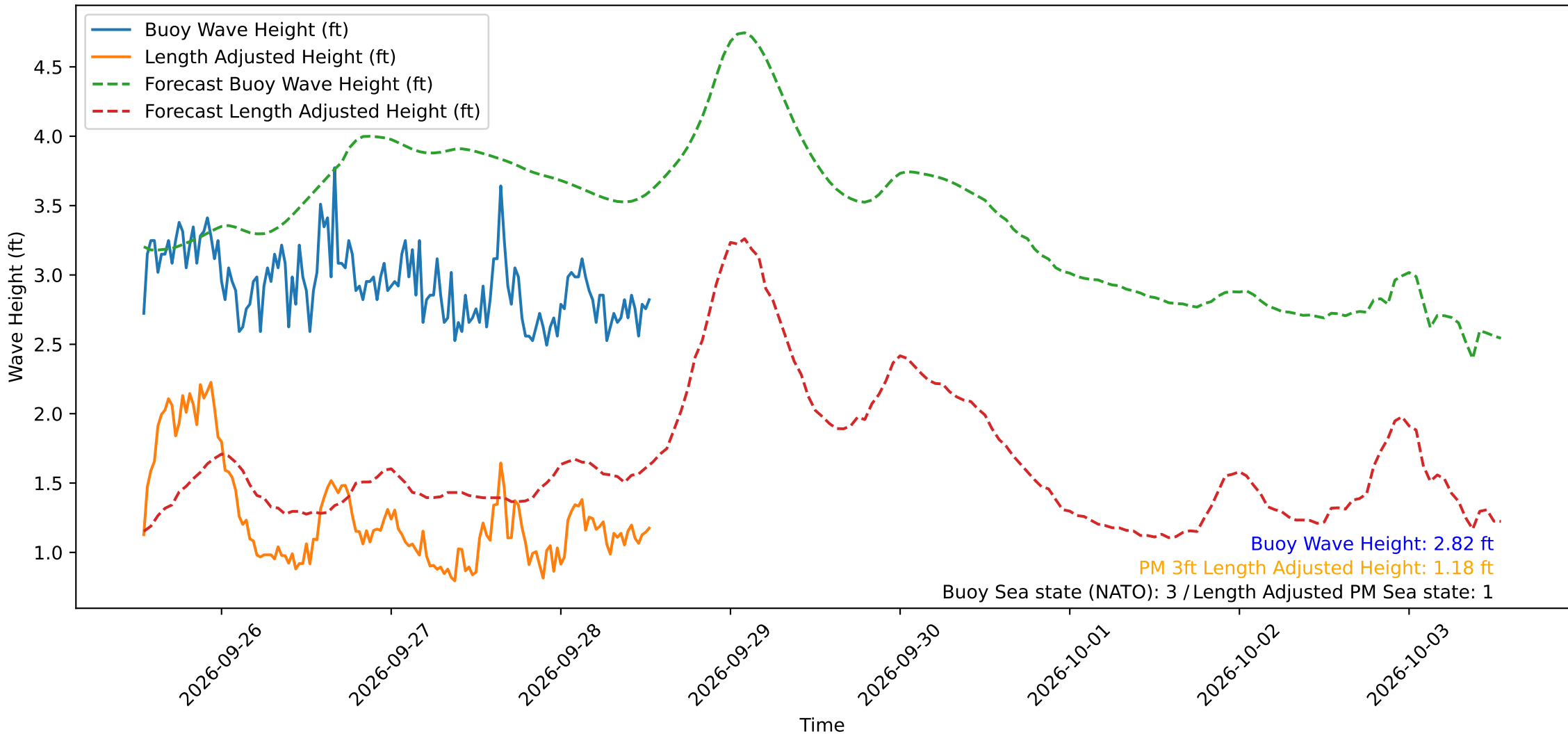
Wave Heights over Time for Oceanside Harbor at 2026-09-28 13:10:29
