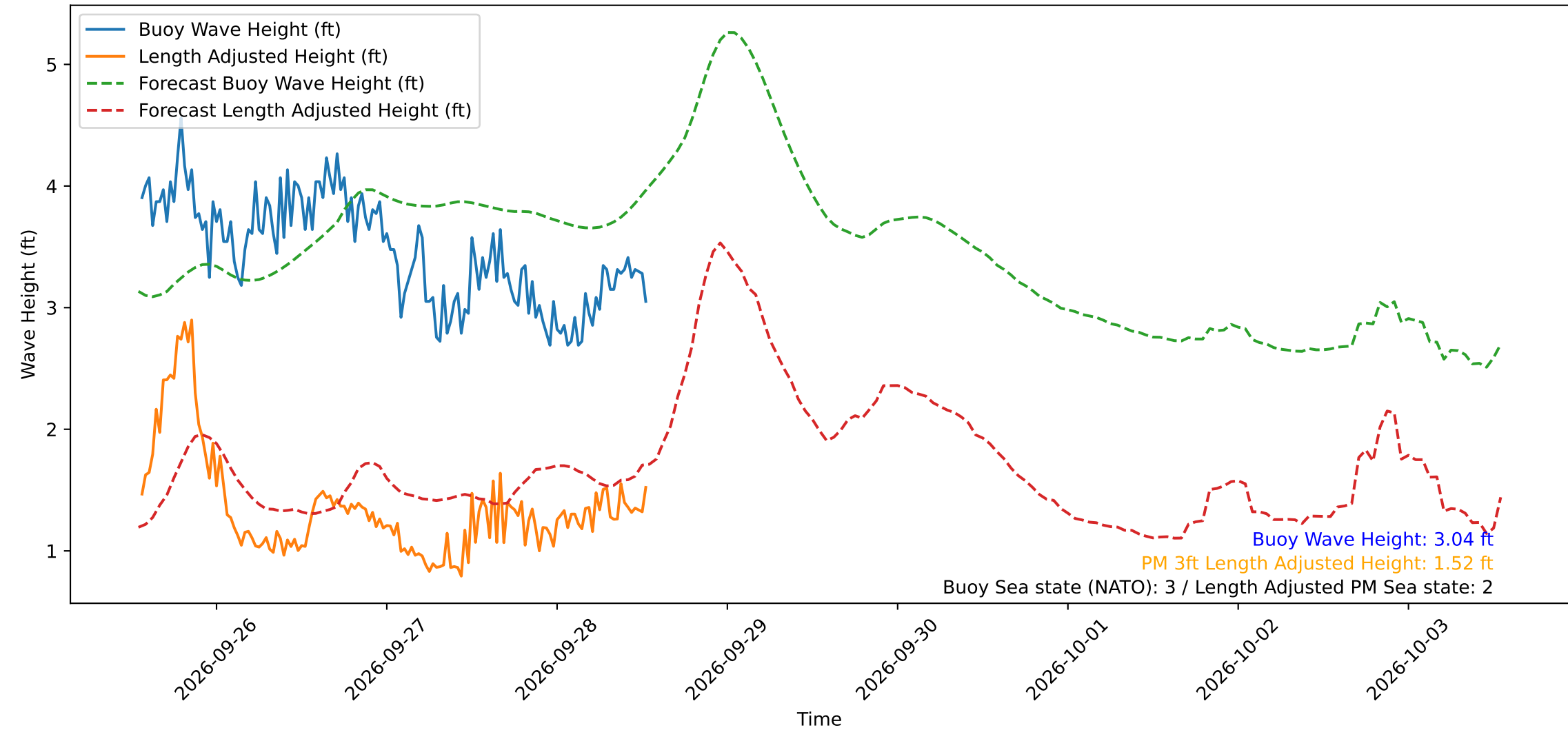
Wave Heights over Time for Green Beach at 2026-09-28 13:11:11
