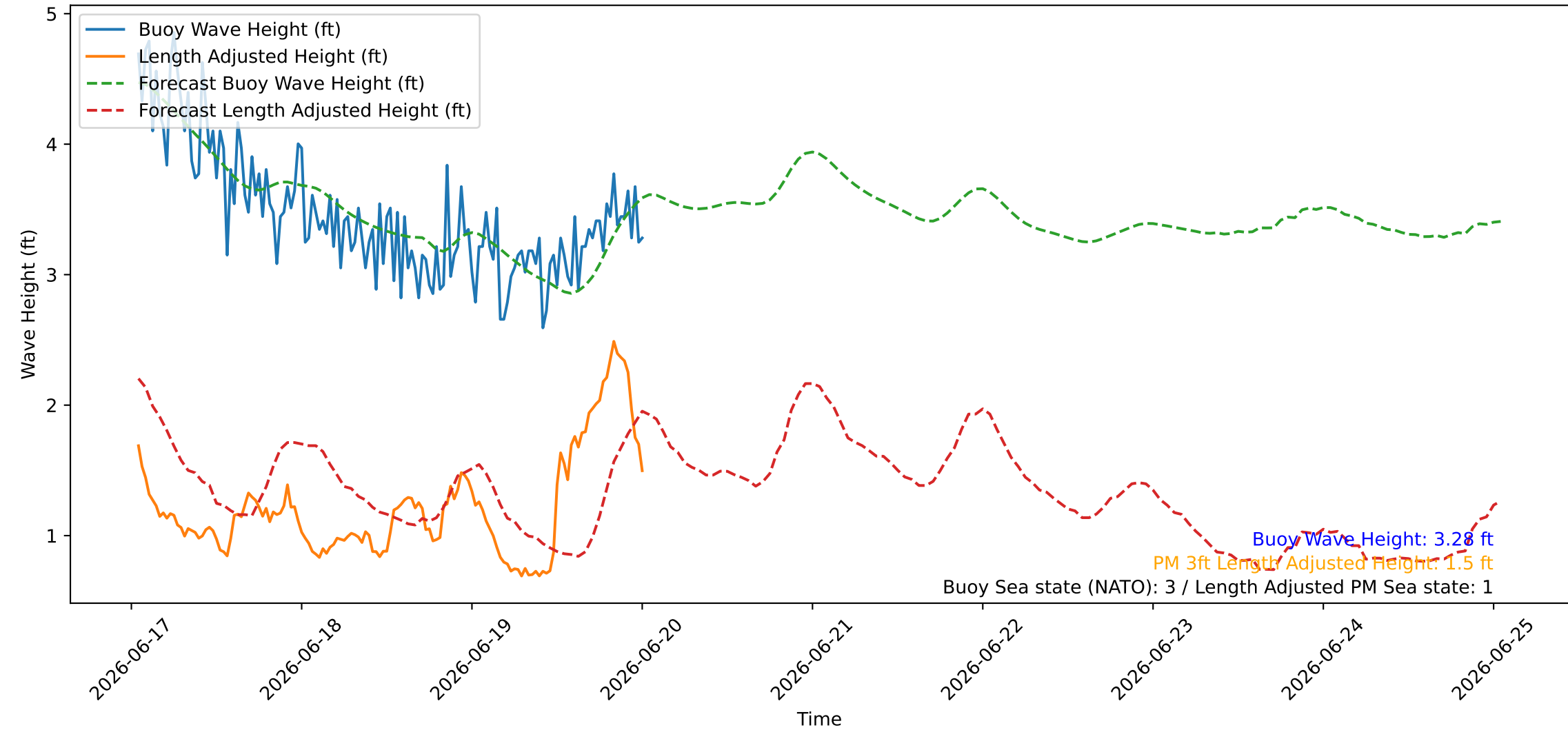
Wave Heights over Time for Red Beach at 2026-06-20 00:40:45
