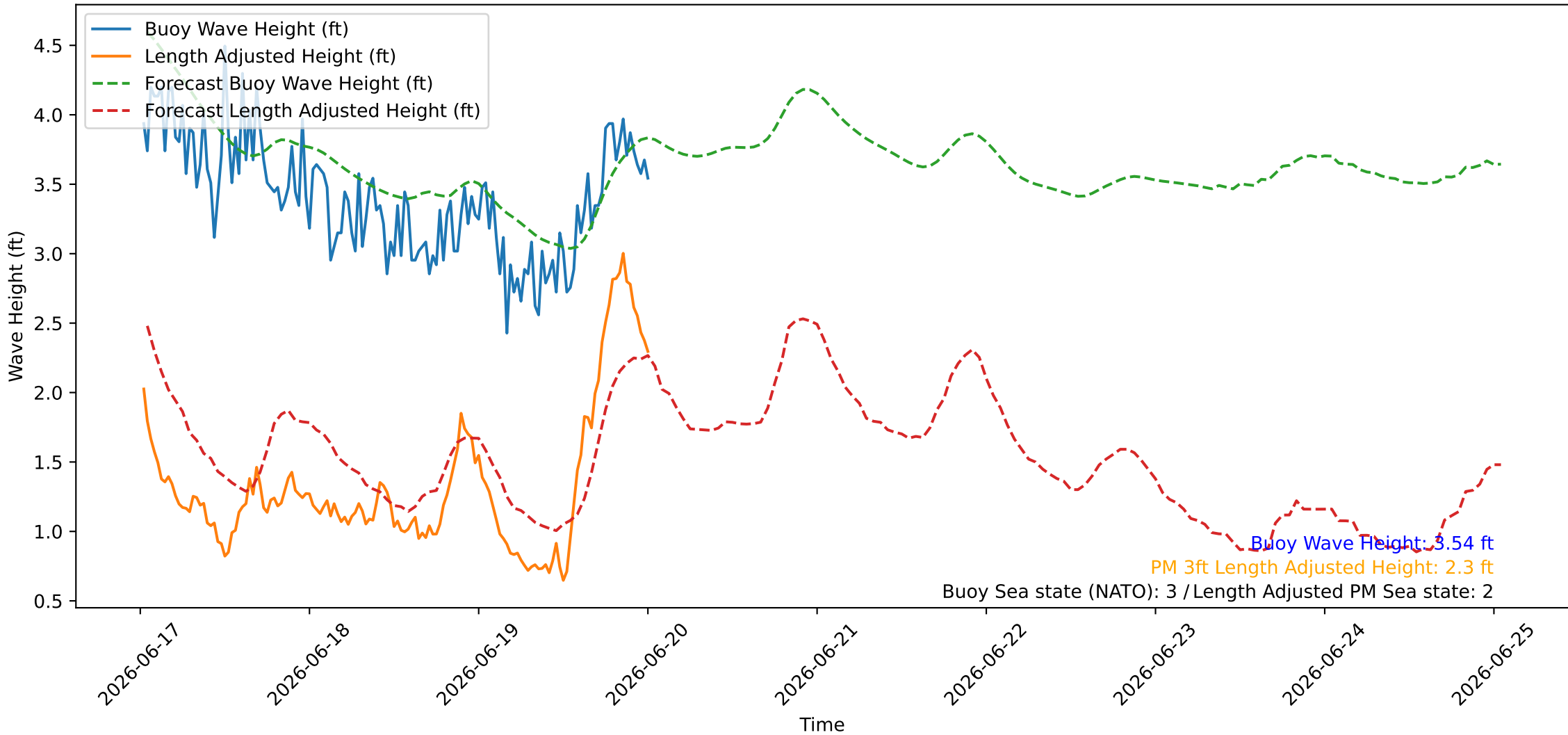
Wave Heights over Time for Green Beach at 2026-06-20 00:41:07
