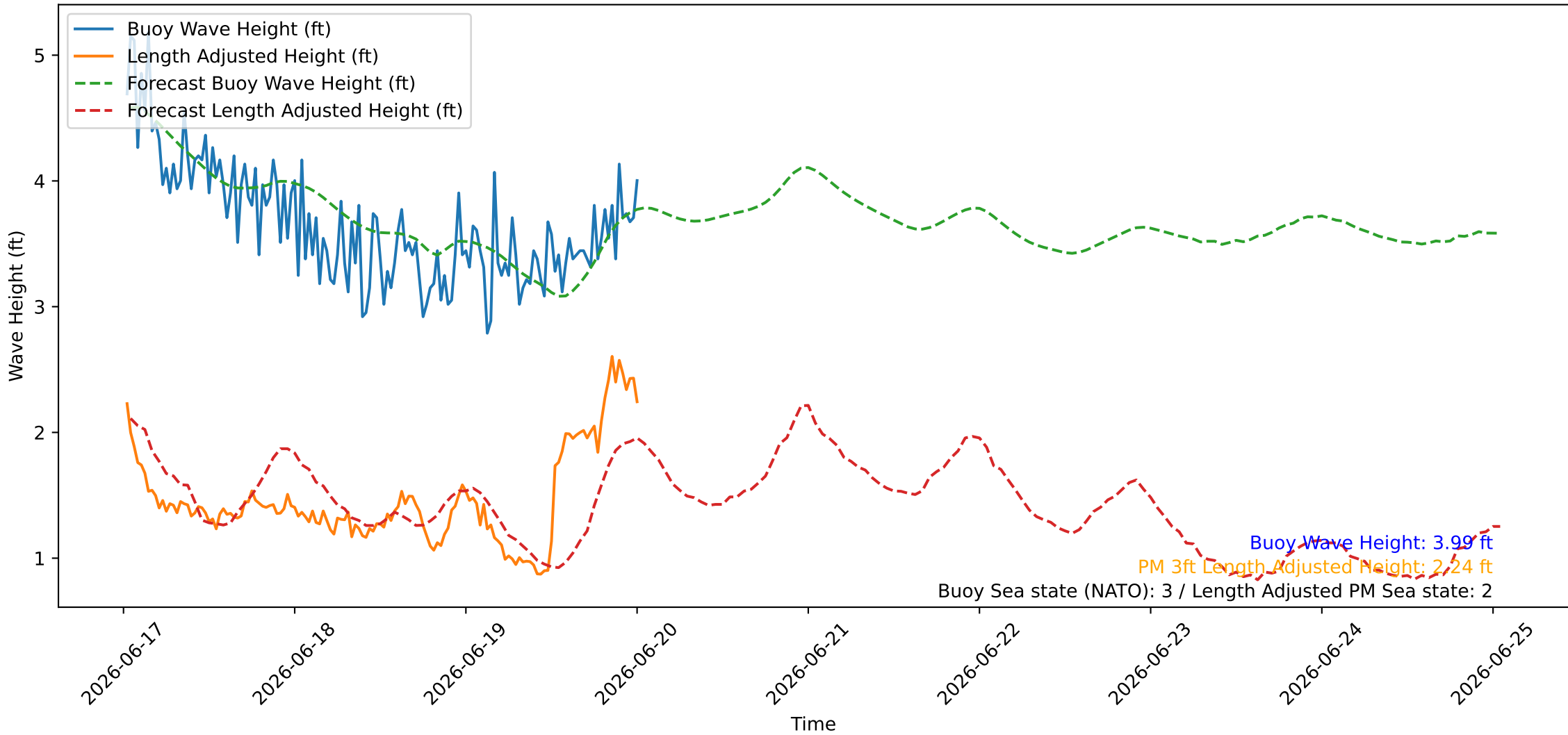
Wave Heights over Time for Oceanside Harbor at 2026-06-20 00:40:25
