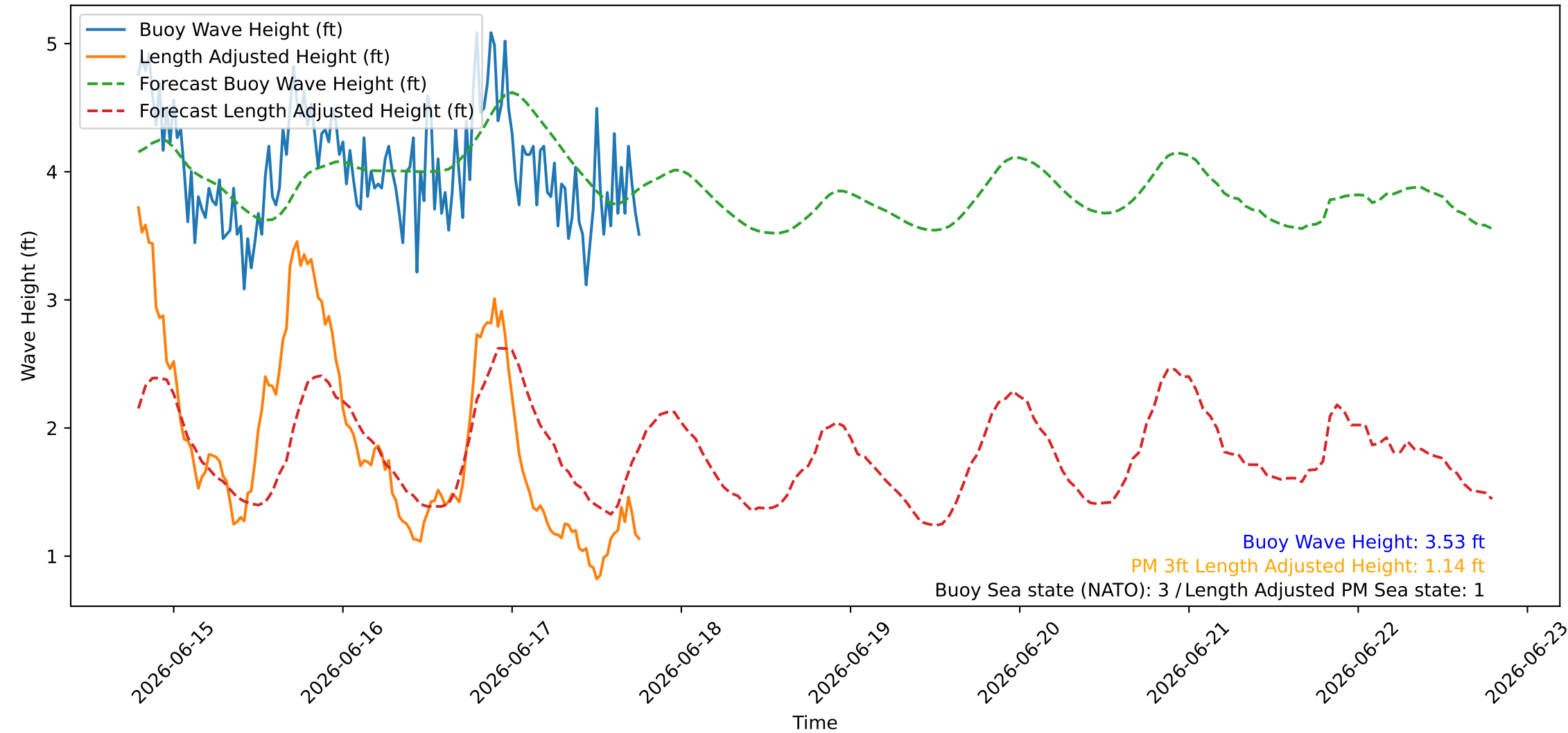
Wave Heights over Time for Green Beach at 2026-06-17 18:51:10
