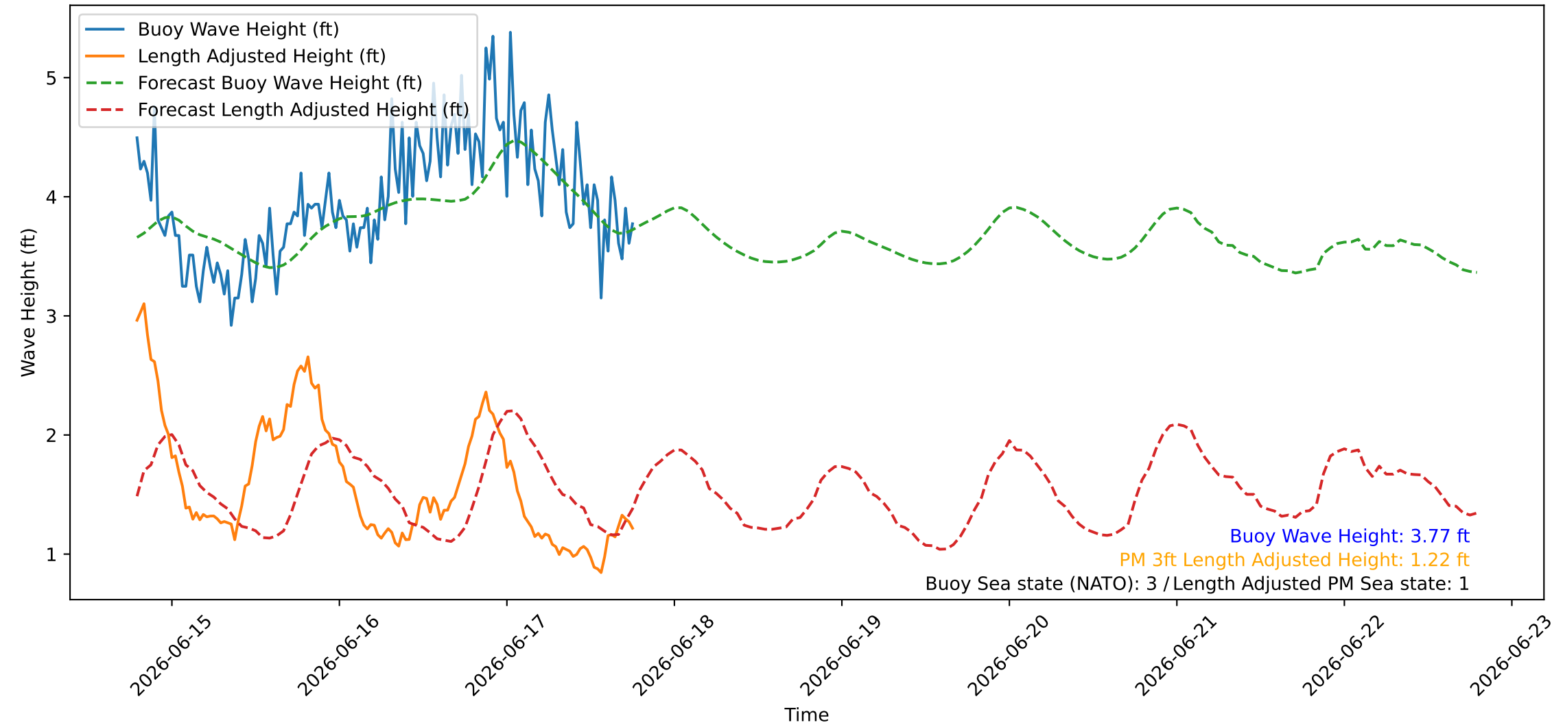
Wave Heights over Time for Red Beach at 2026-06-17 18:50:47
