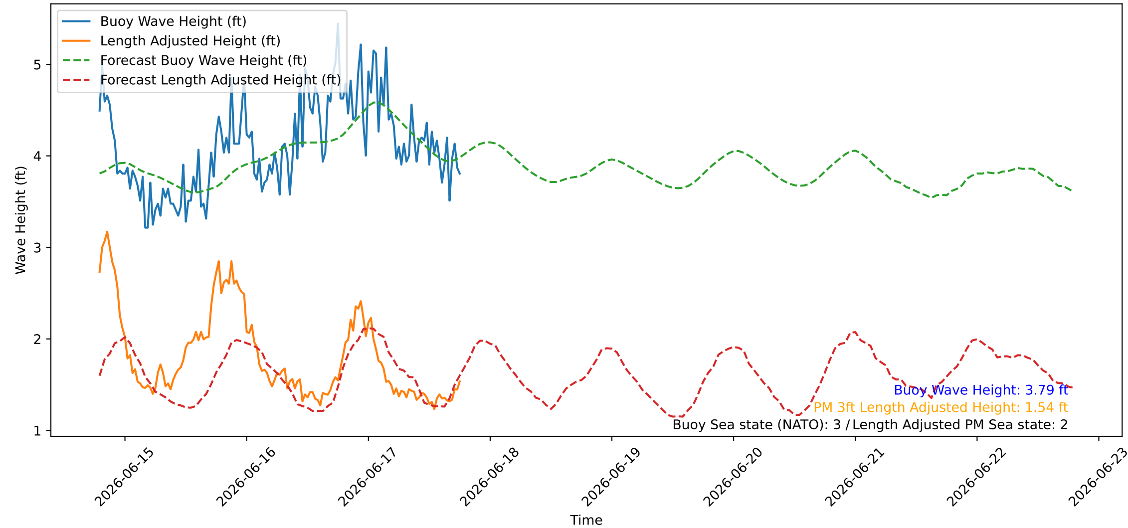
Wave Heights over Time for Oceanside Harbor at 2026-06-17 18:50:26
