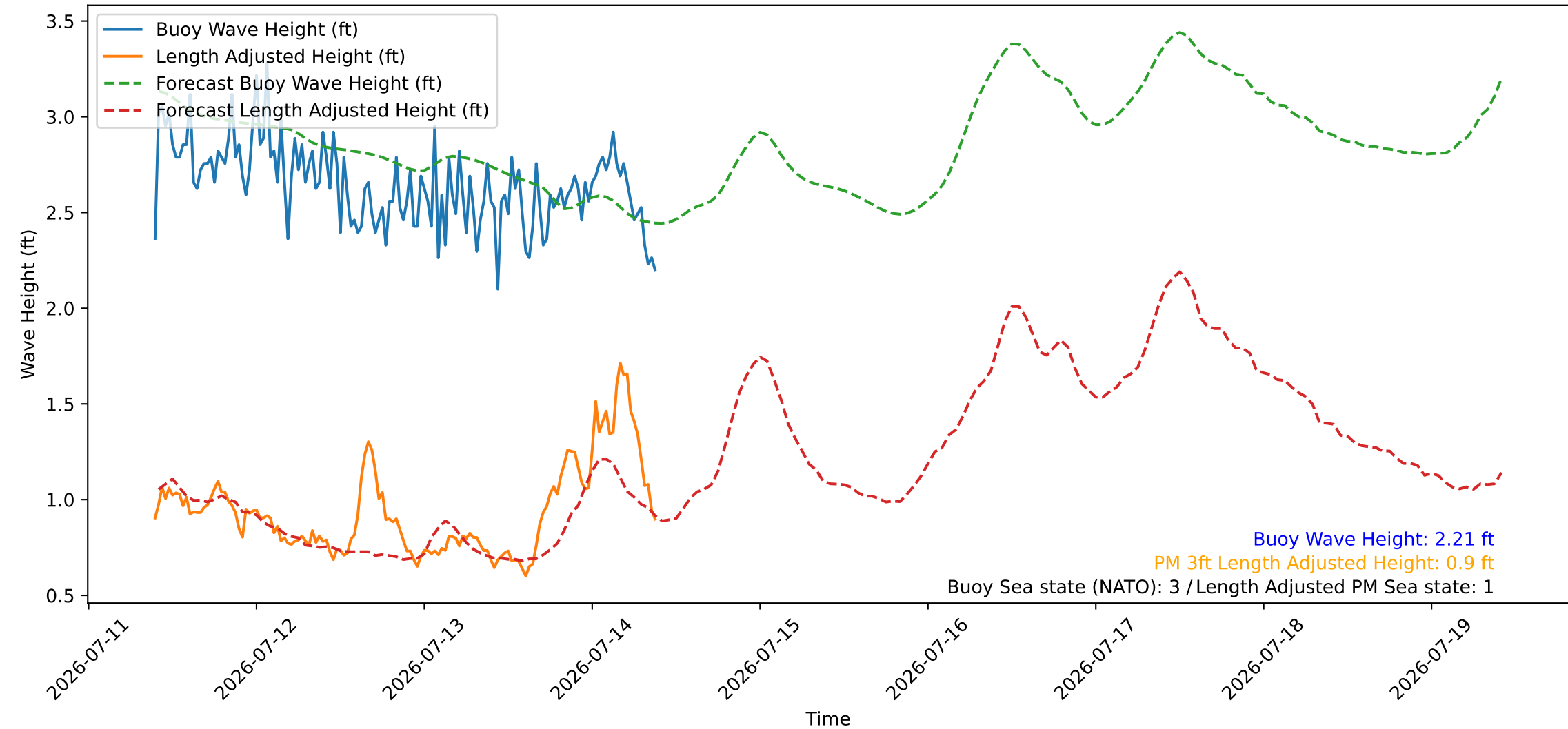
Wave Heights over Time for Oceanside Harbor at 2026-07-14 09:30:27
