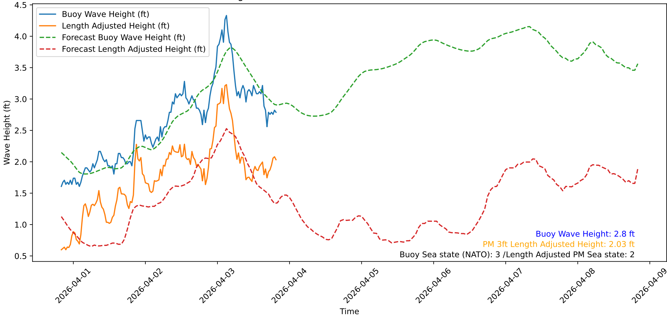
Wave Heights over Time for Green Beach at 2026-04-03 20:11:20
