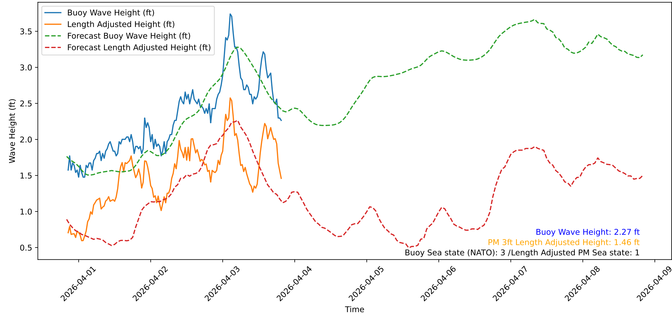
Wave Heights over Time for Red Beach at 2026-04-03 20:10:53
