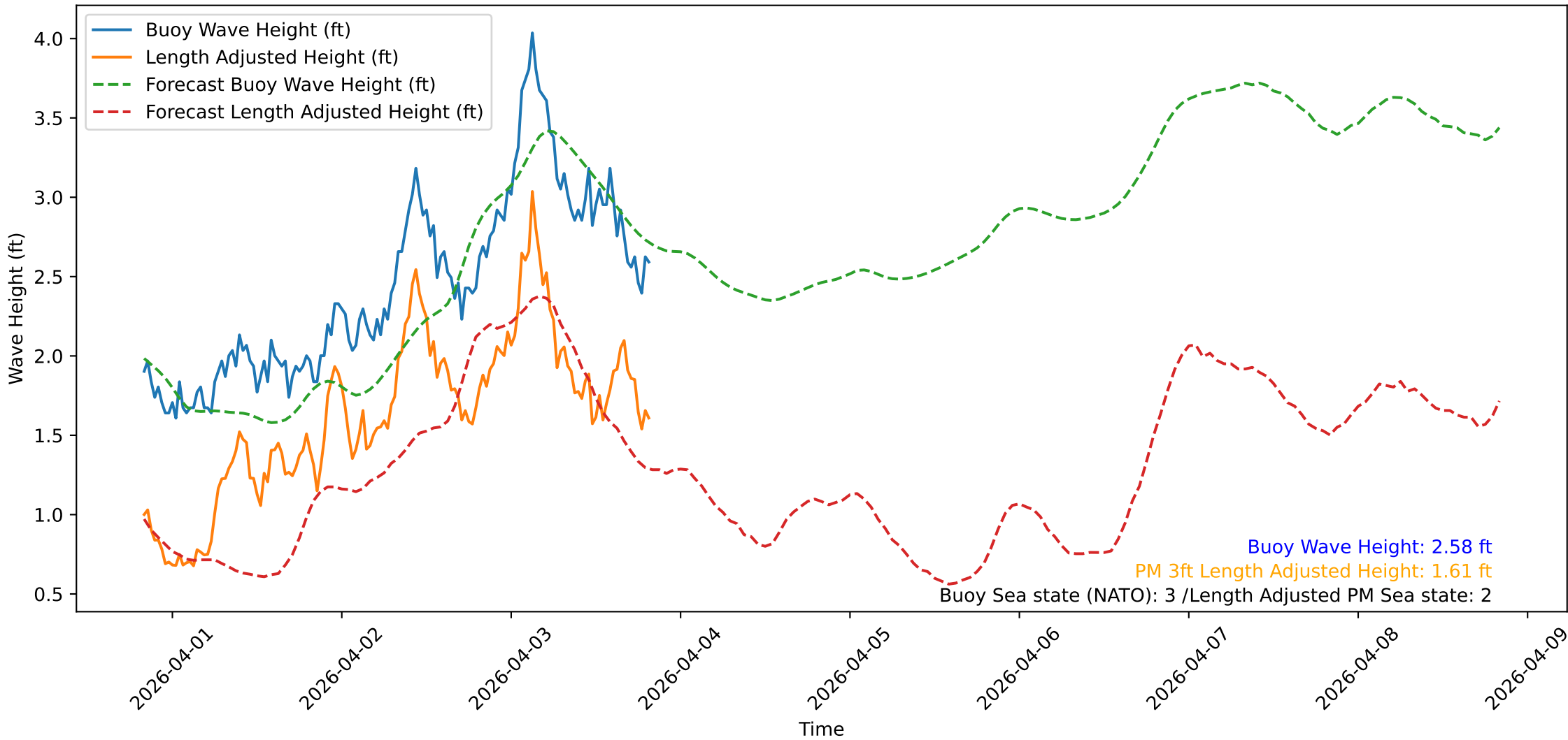
Wave Heights over Time for Oceanside Harbor at 2026-04-03 20:10:35
