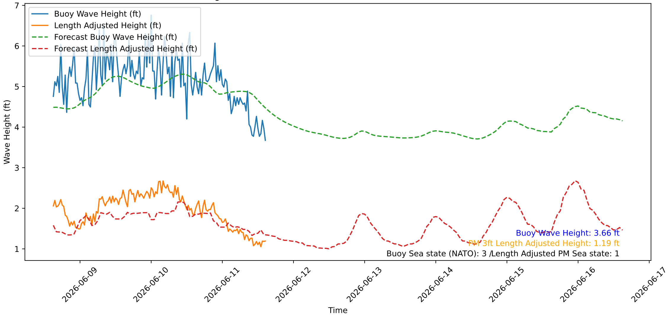
Wave Heights over Time for Oceanside Harbor at 2026-06-11 15:10:26
