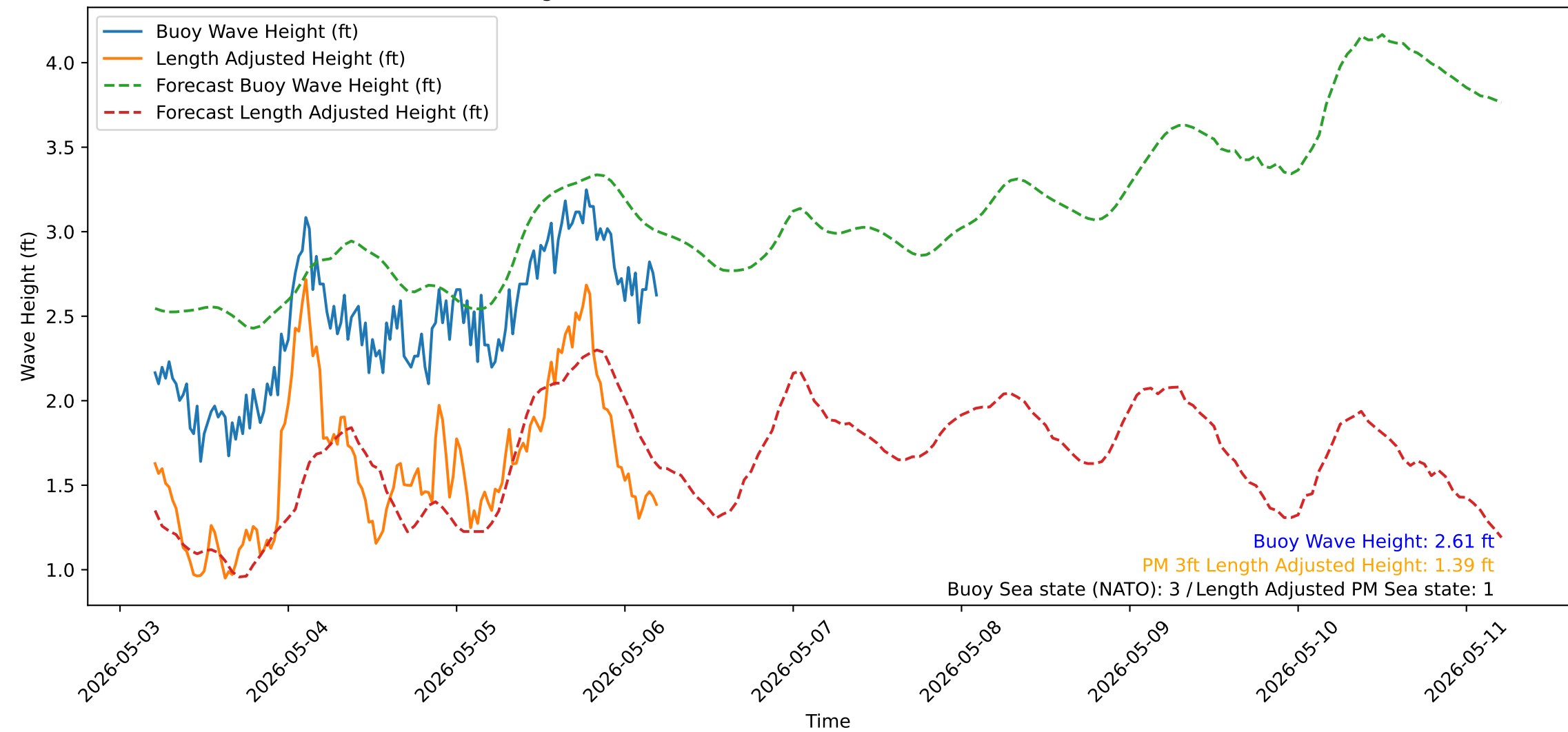
Wave Heights over Time for Oceanside Harbor at 2026-05-06 05:10:31
