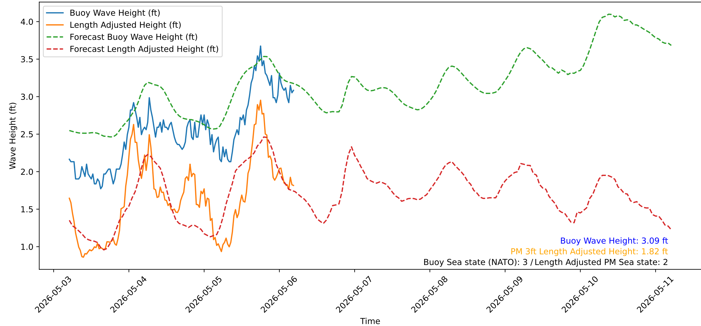
Wave Heights over Time for Green Beach at 2026-05-06 05:11:13
