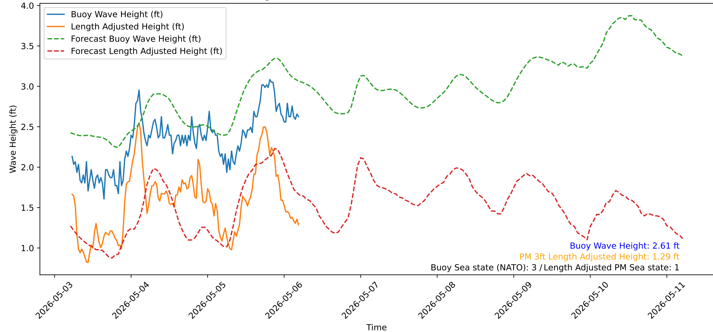
Wave Heights over Time for Red Beach at 2026-05-06 05:10:50
