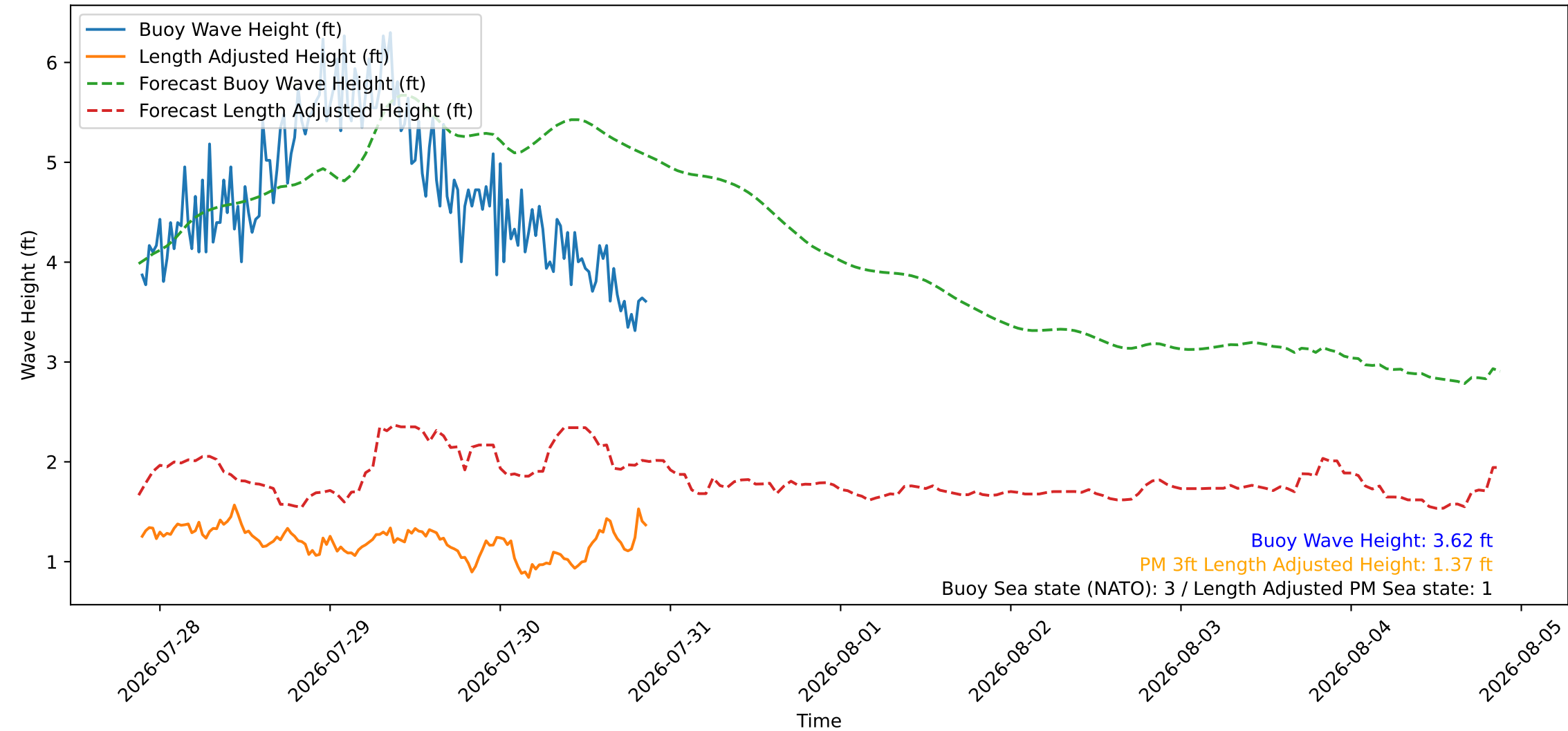
Wave Heights over Time for Green Beach at 2026-07-30 21:21:11
