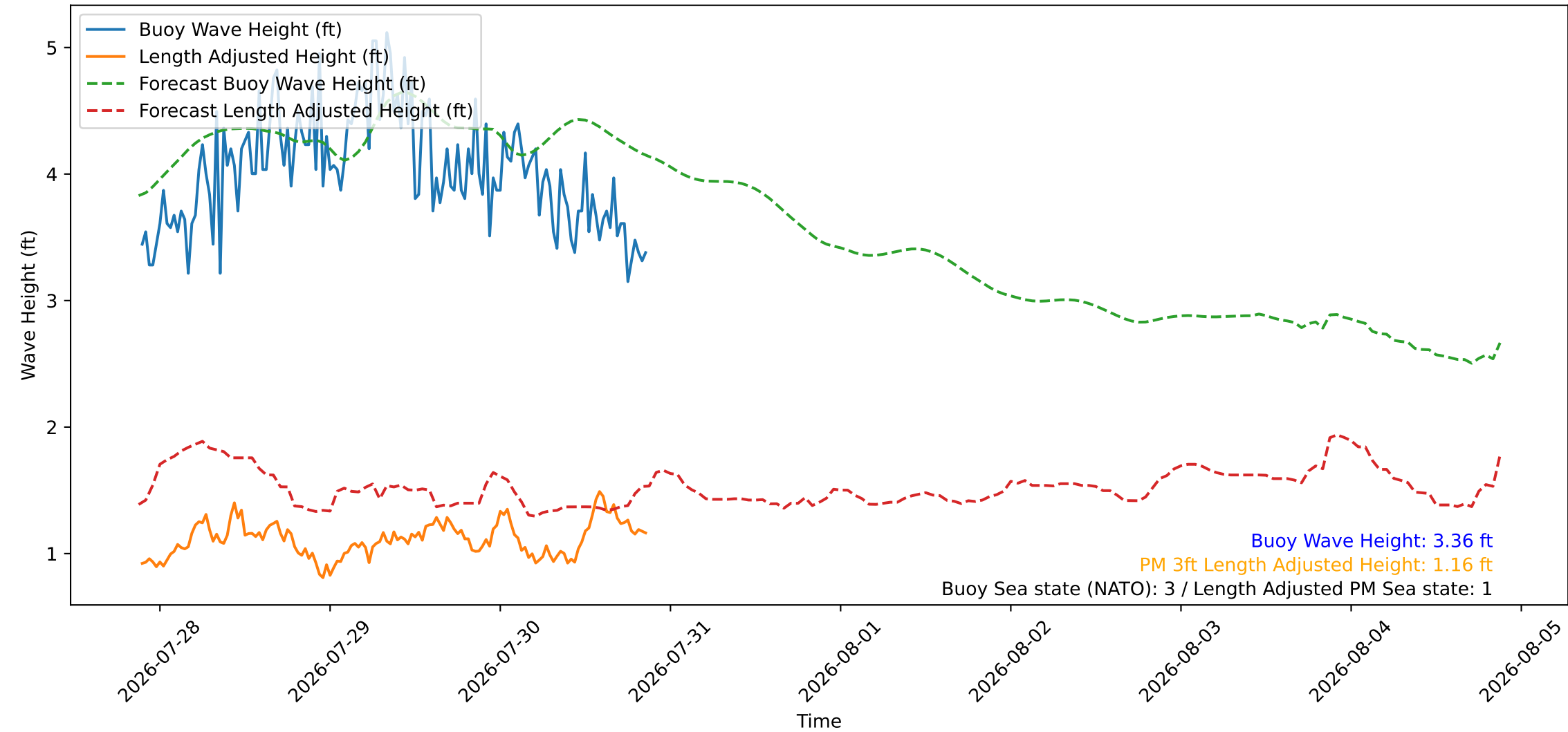
Wave Heights over Time for Red Beach at 2026-07-30 21:20:48
