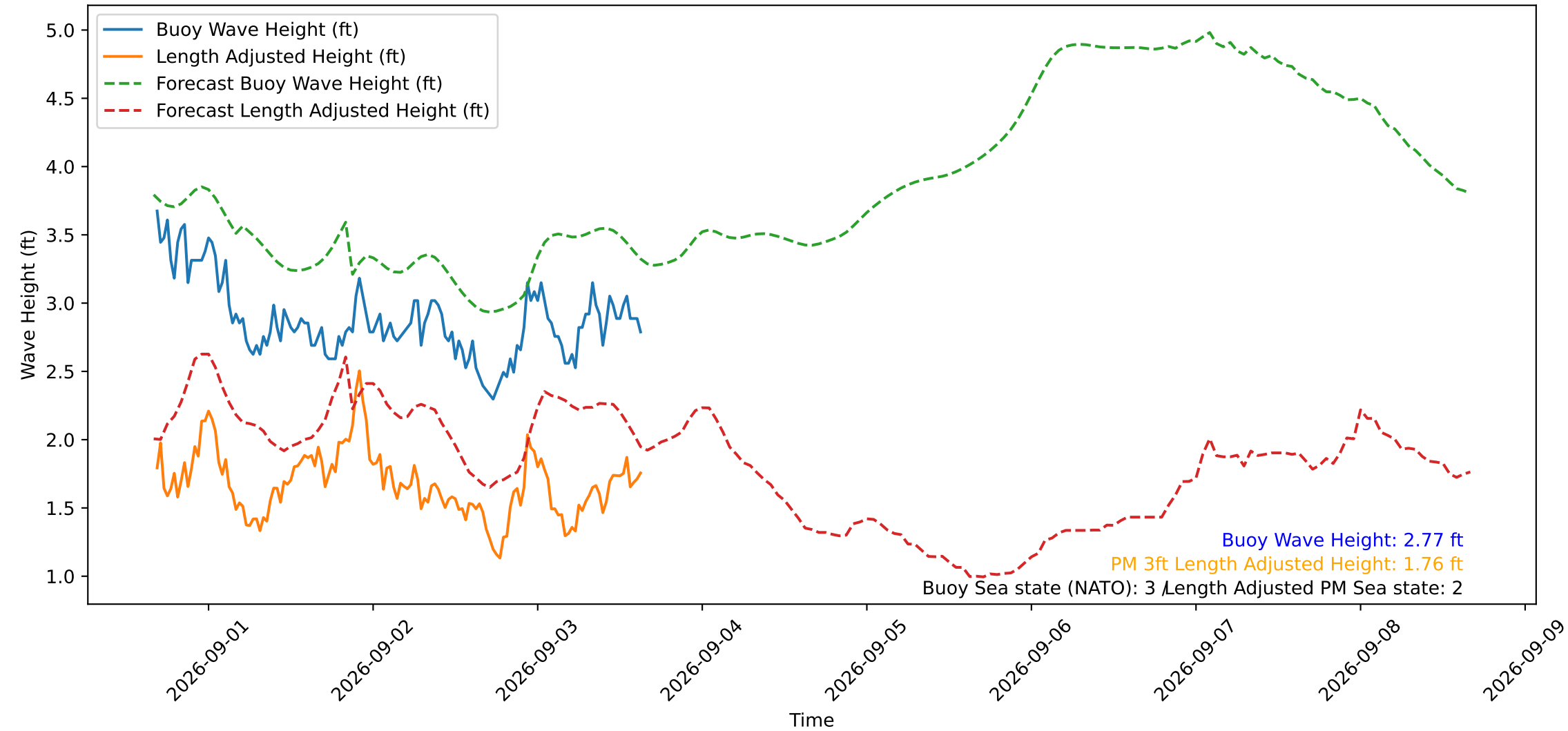
Wave Heights over Time for Red Beach at 2026-09-03 16:00:50
