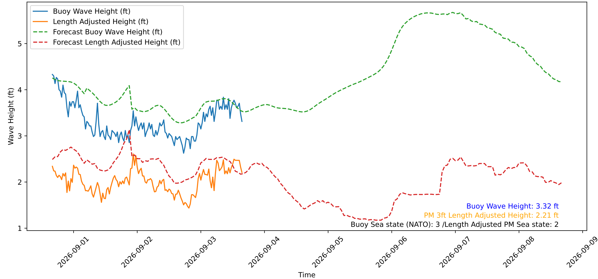
Wave Heights over Time for Oceanside Harbor at 2026-09-03 16:00:30
