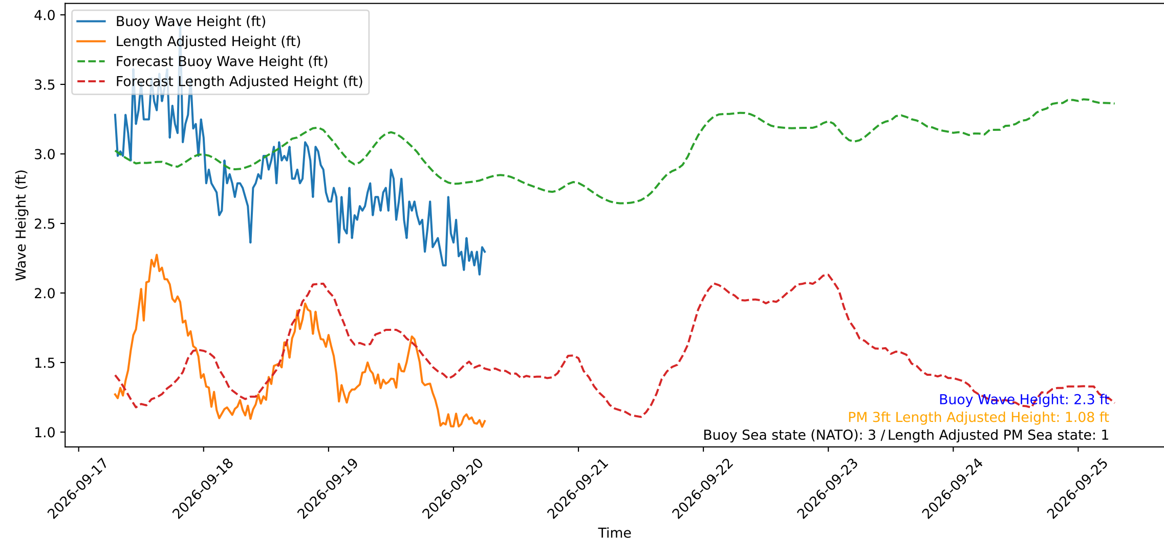
Wave Heights over Time for Oceanside Harbor at 2026-09-20 07:00:29
