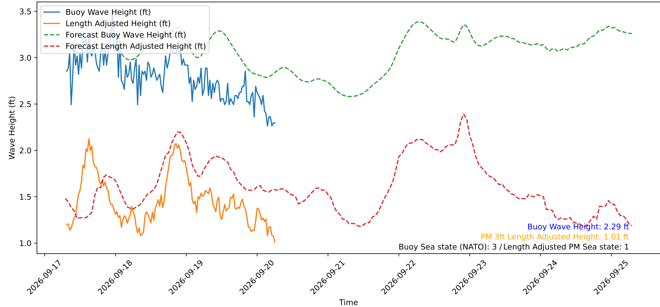
Wave Heights over Time for Green Beach at 2026-09-20 07:01:11
