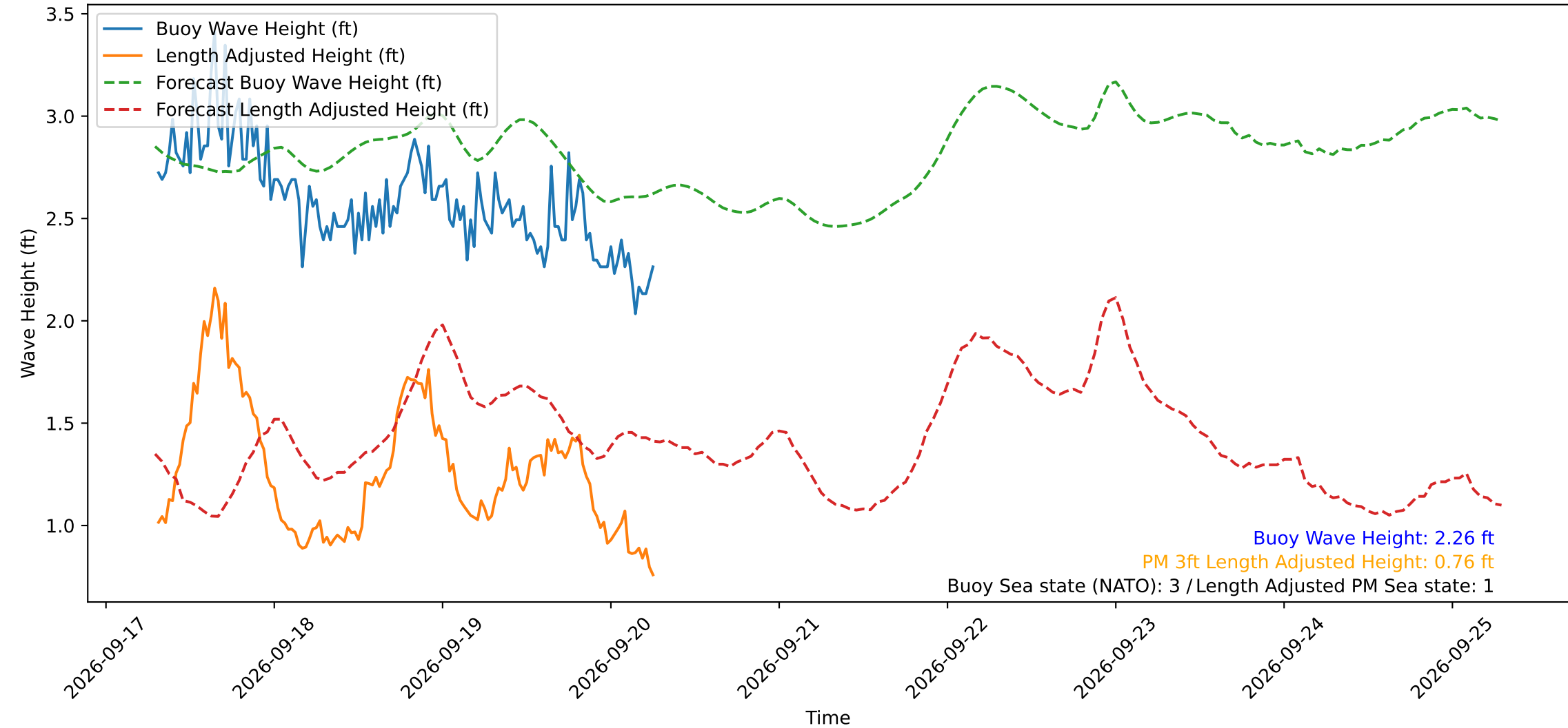
Wave Heights over Time for Red Beach at 2026-09-20 07:00:49
