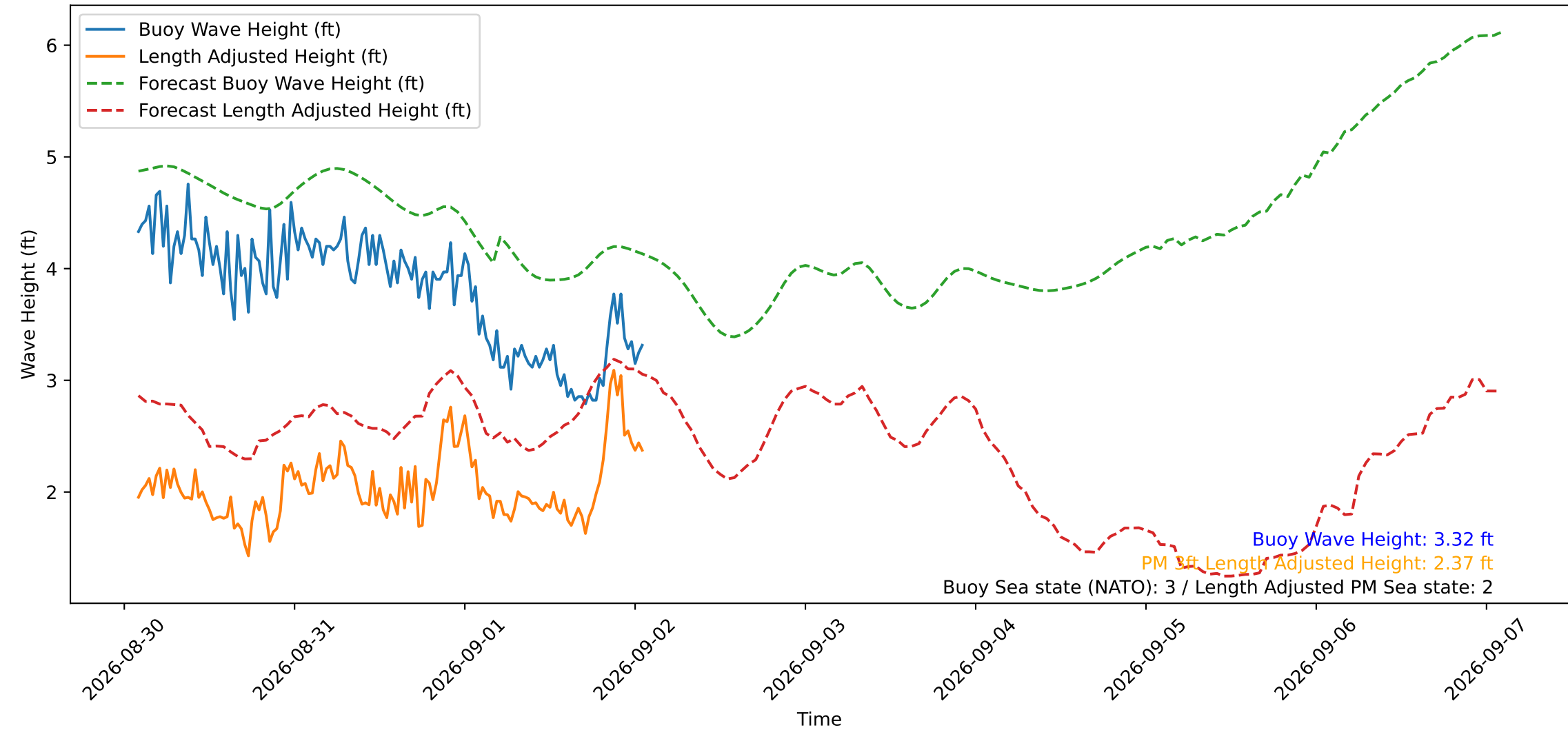
Wave Heights over Time for Green Beach at 2026-09-02 01:51:15
