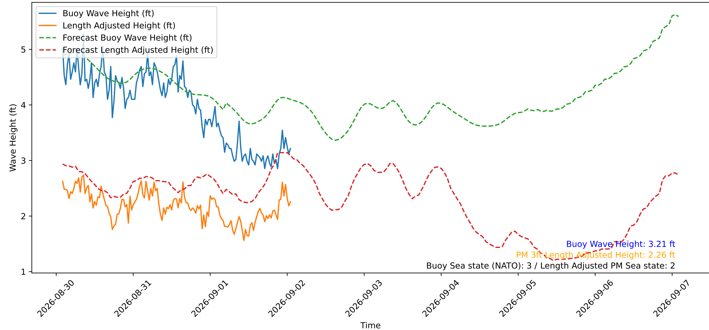
Wave Heights over Time for Oceanside Harbor at 2026-09-02 01:50:30
