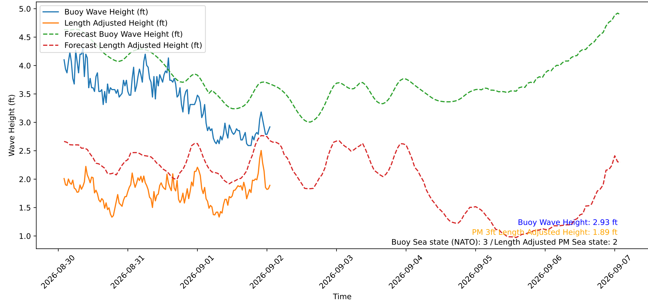
Wave Heights over Time for Red Beach at 2026-09-02 01:50:51
