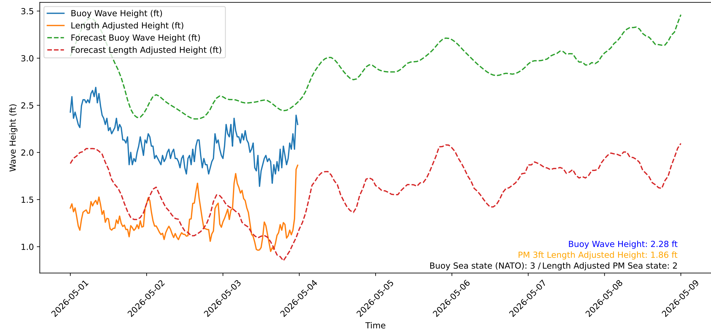
Wave Heights over Time for Oceanside Harbor at 2026-05-04 00:00:31
