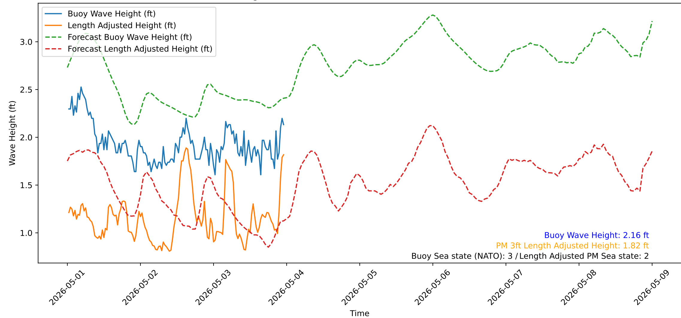
Wave Heights over Time for Red Beach at 2026-05-04 00:00:50
