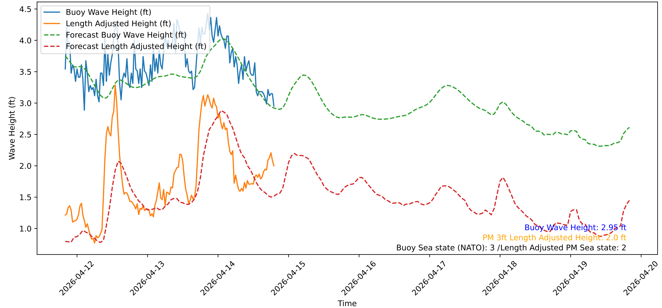
Wave Heights over Time for Red Beach at 2026-04-14 19:40:51
