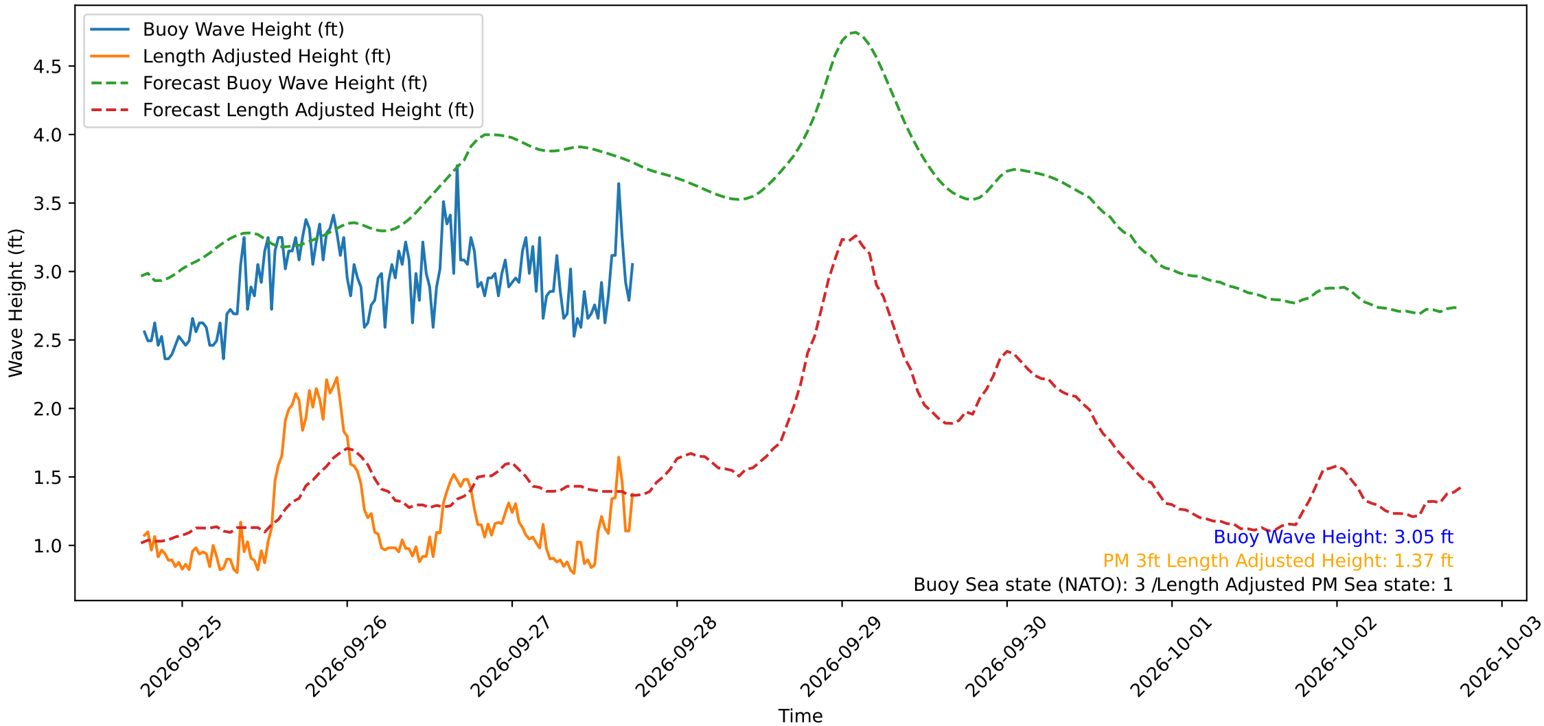
Wave Heights over Time for Oceanside Harbor at 2026-09-27 18:20:30
