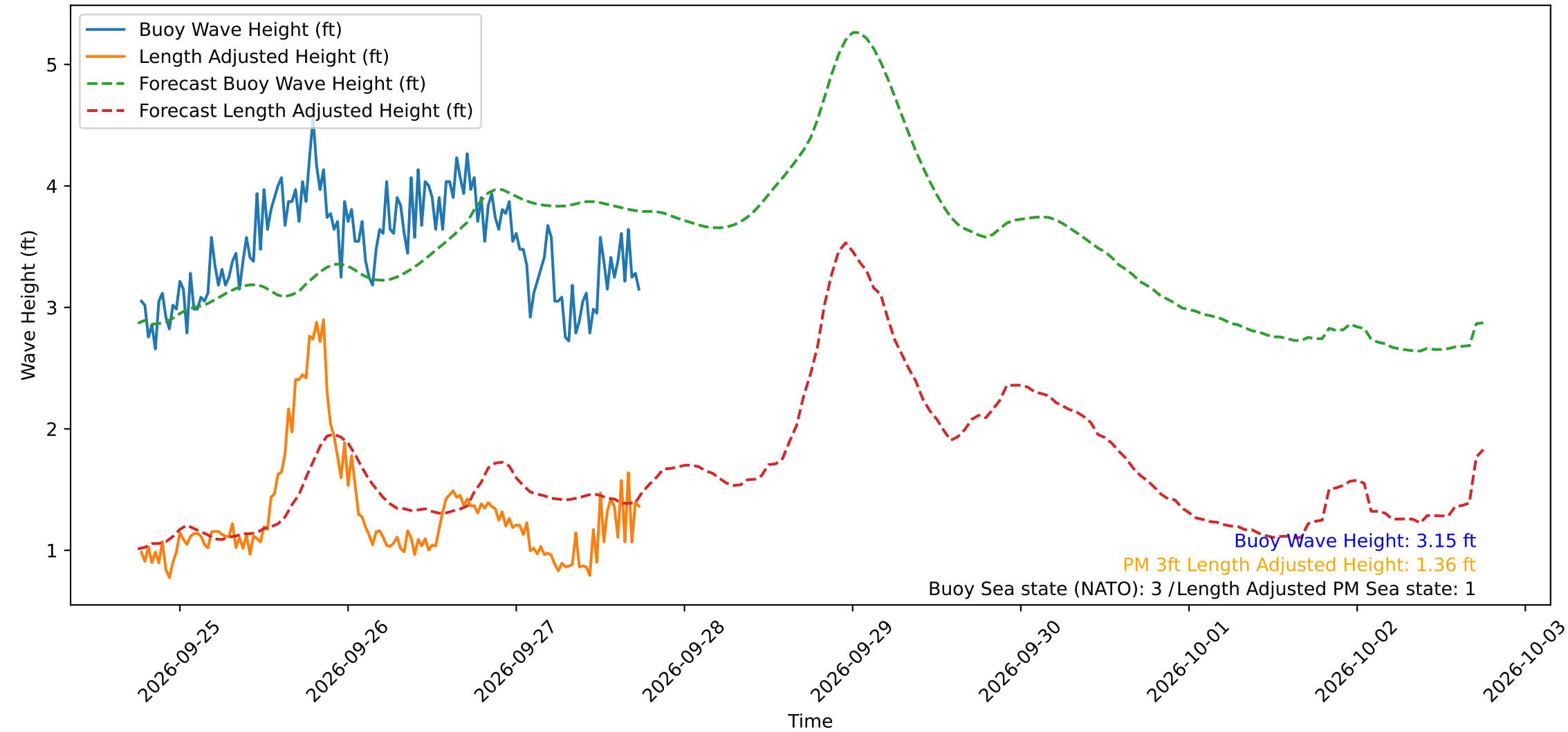
Wave Heights over Time for Green Beach at 2026-09-27 18:21:15
