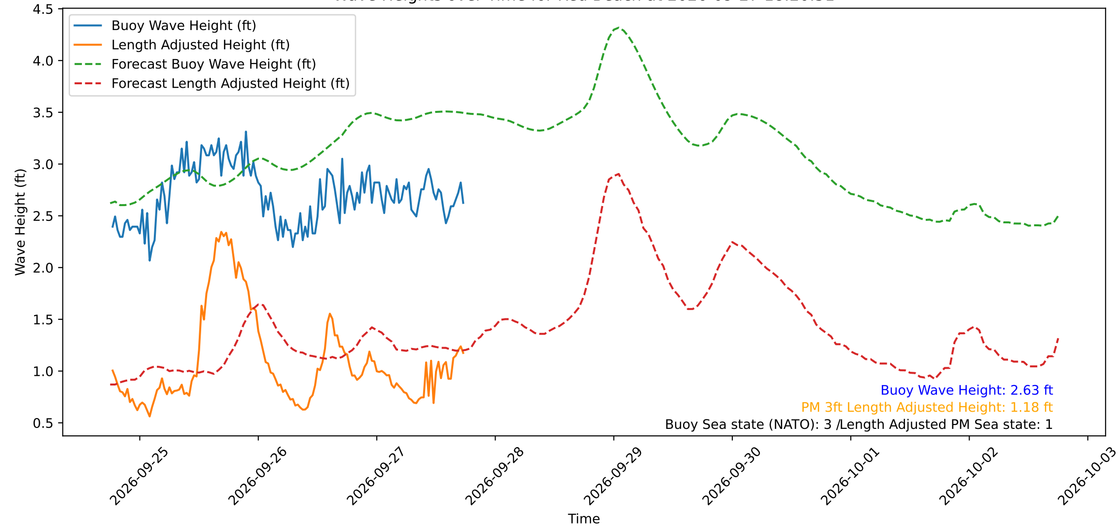
Wave Heights over Time for Red Beach at 2026-09-27 18:20:51
