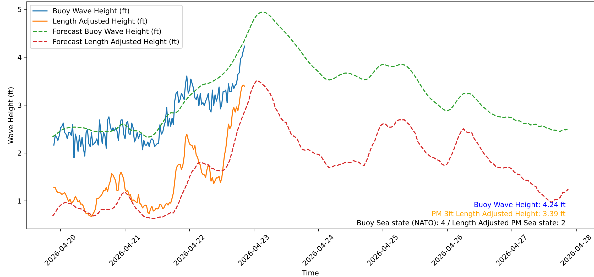
Wave Heights over Time for Oceanside Harbor at 2026-04-22 21:20:31
