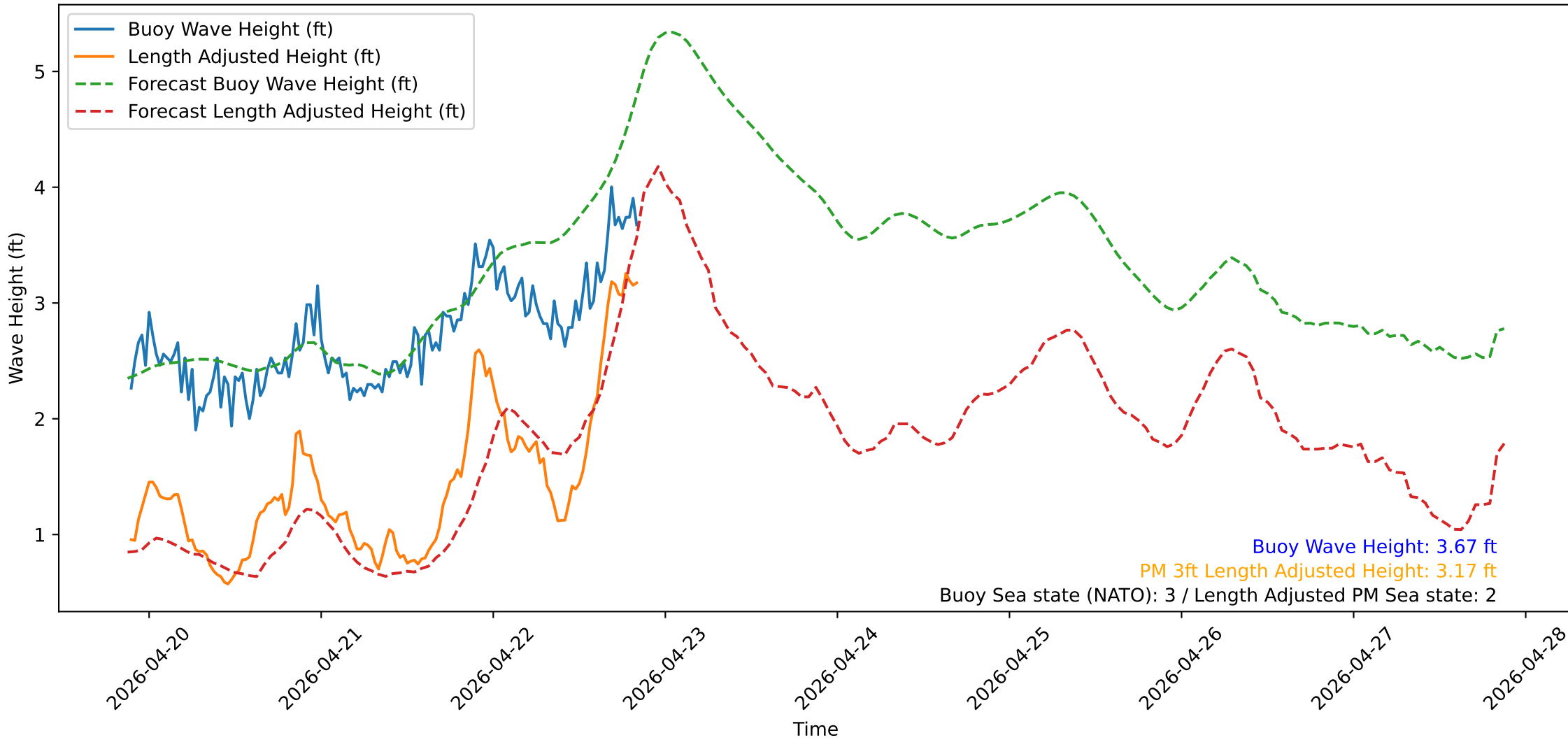
Wave Heights over Time for Green Beach at 2026-04-22 21:21:14
