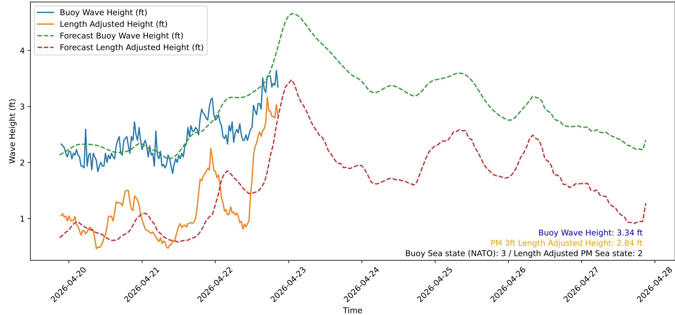
Wave Heights over Time for Red Beach at 2026-04-22 21:20:52
