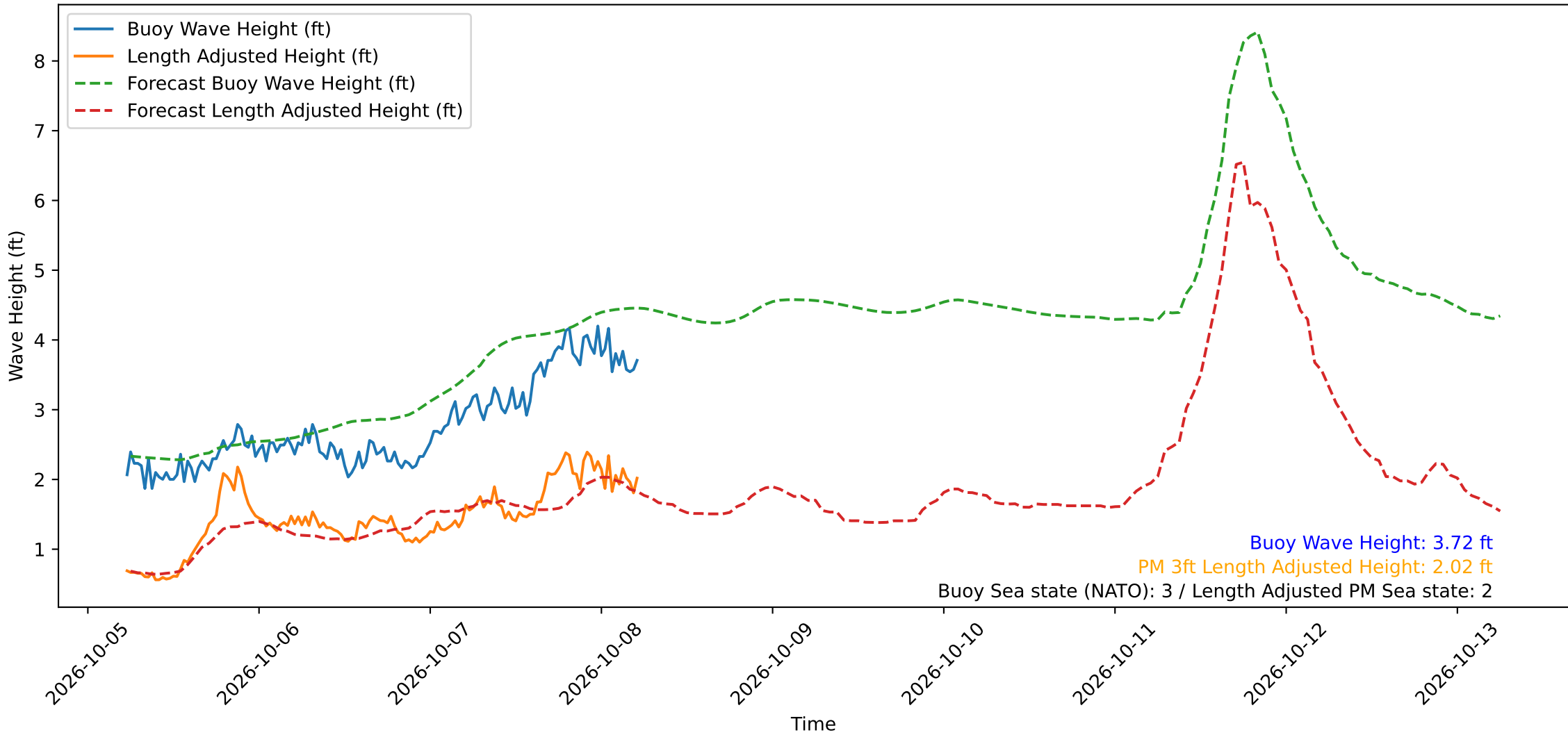
Wave Heights over Time for Oceanside Harbor at 2026-10-08 05:40:30
