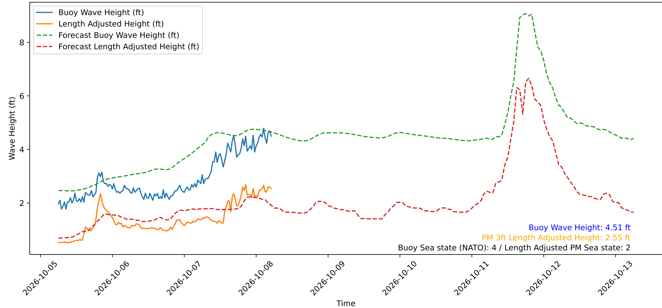
Wave Heights over Time for Green Beach at 2026-10-08 05:41:12
