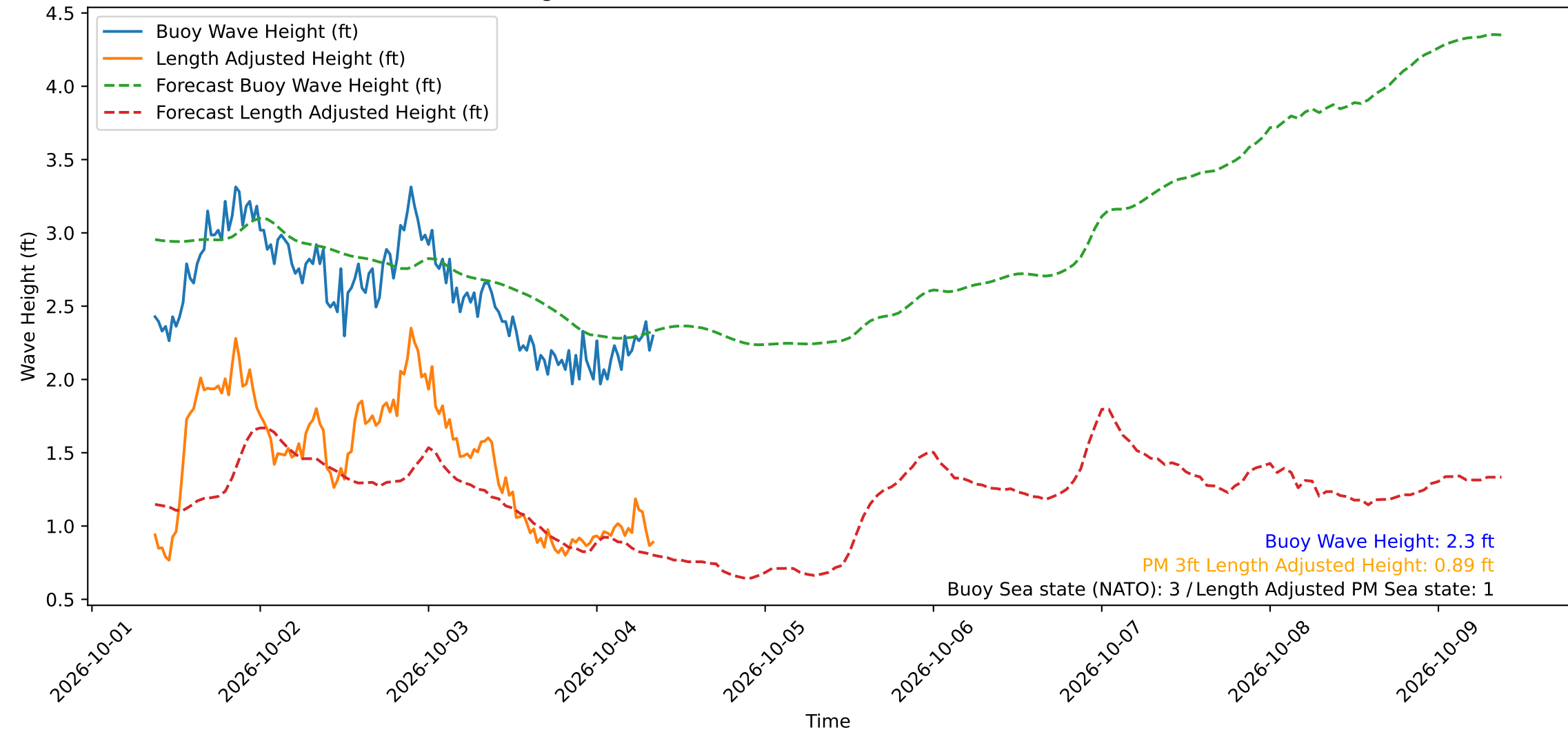
Wave Heights over Time for Oceanside Harbor at 2026-10-04 09:10:30
