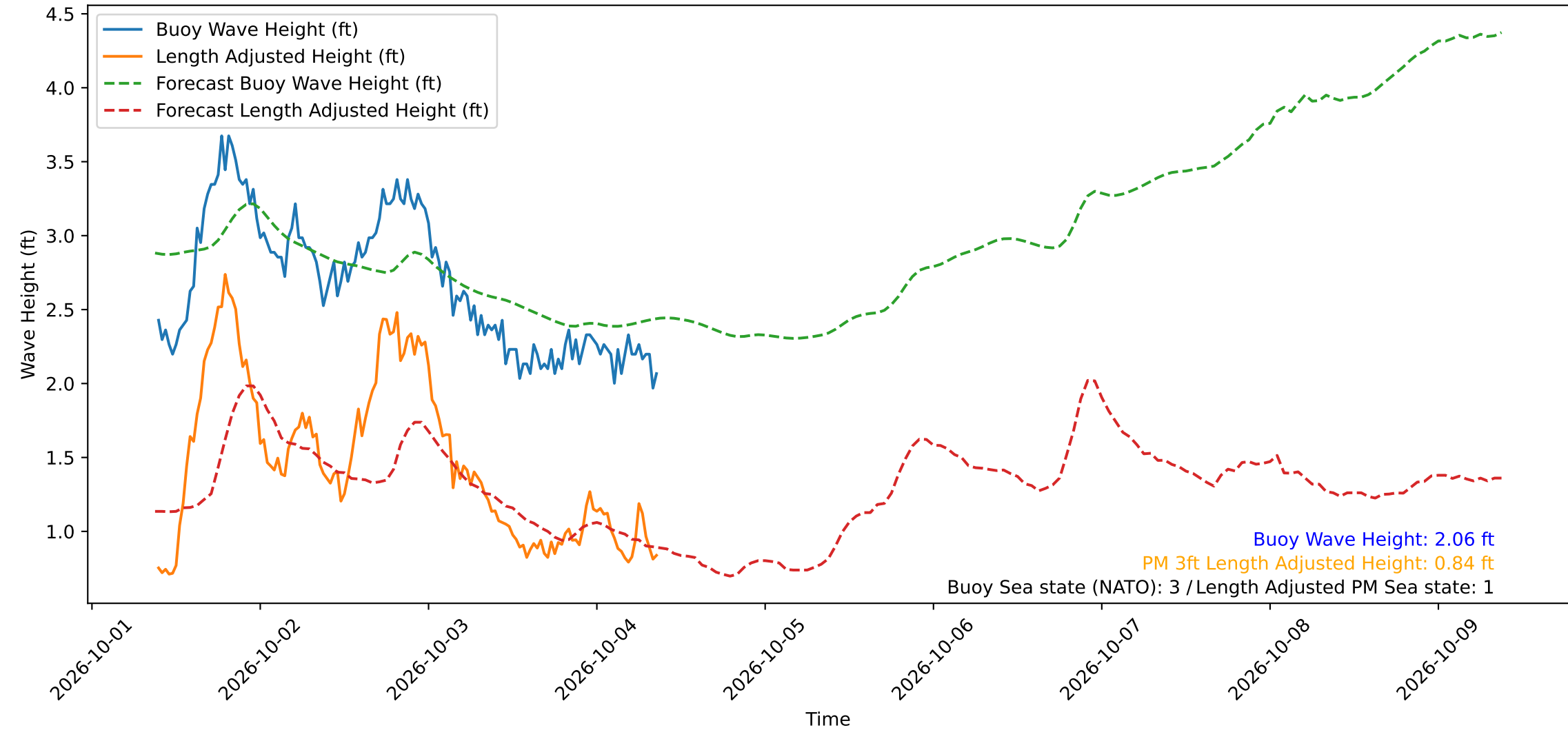
Wave Heights over Time for Green Beach at 2026-10-04 09:11:13
