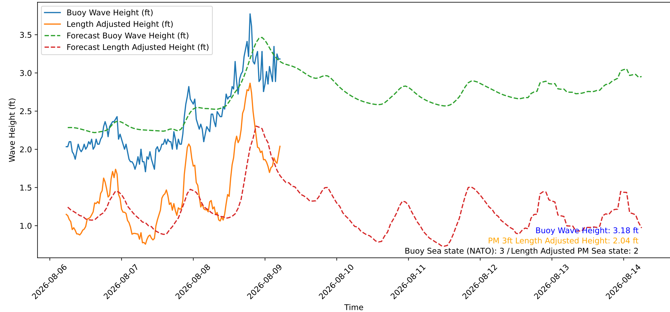
Wave Heights over Time for Green Beach at 2026-08-09 05:41:08
