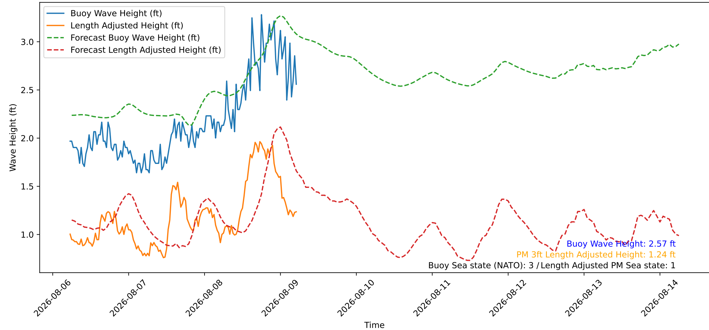
Wave Heights over Time for Oceanside Harbor at 2026-08-09 05:40:27
