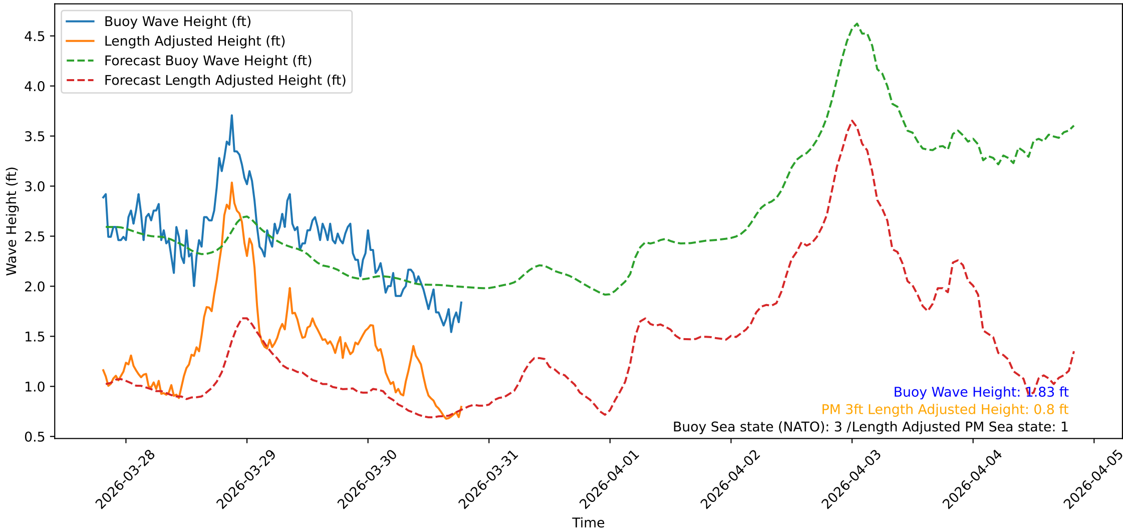
Wave Heights over Time for Green Beach at 2026-03-30 19:31:10
