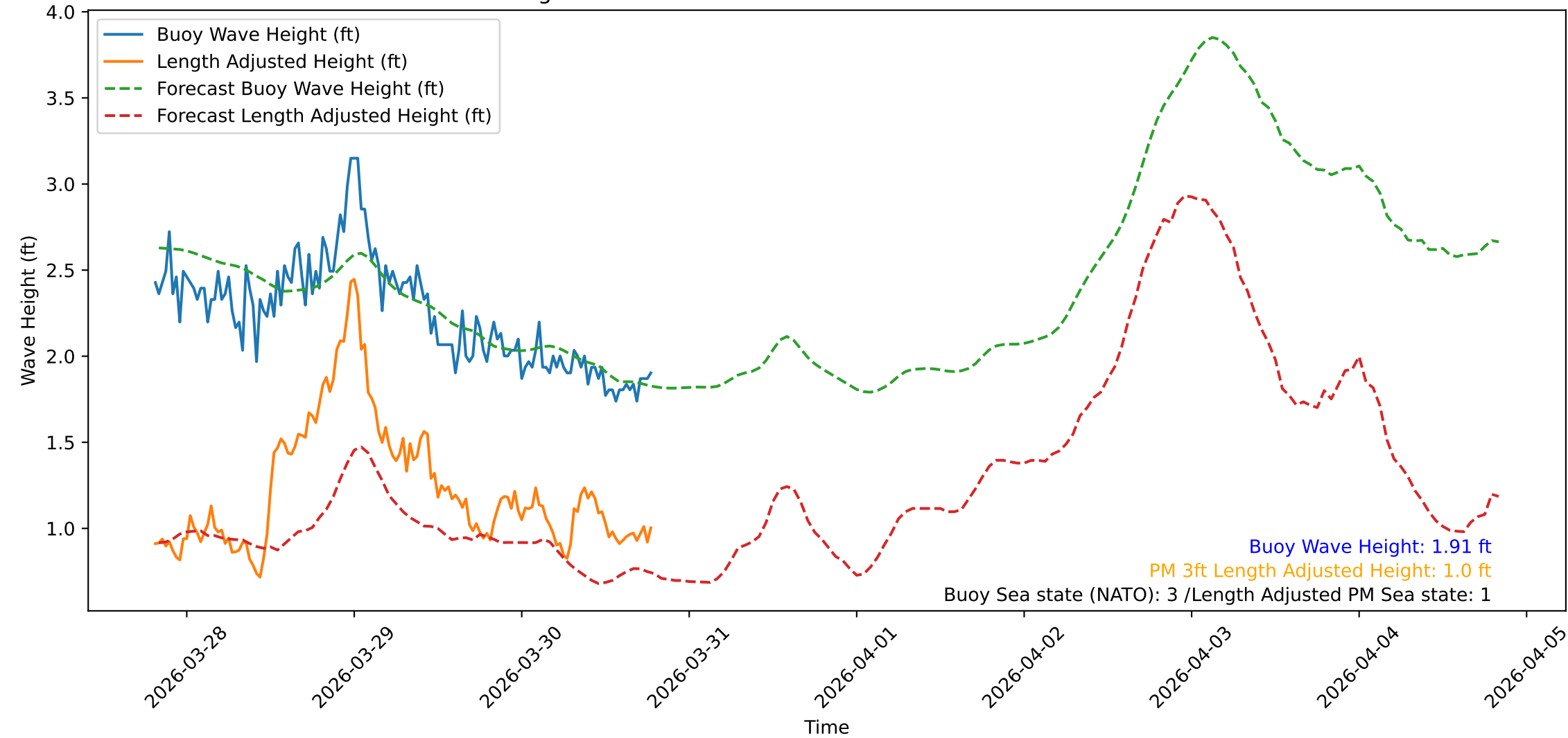
Wave Heights over Time for Oceanside Harbor at 2026-03-30 19:30:31
