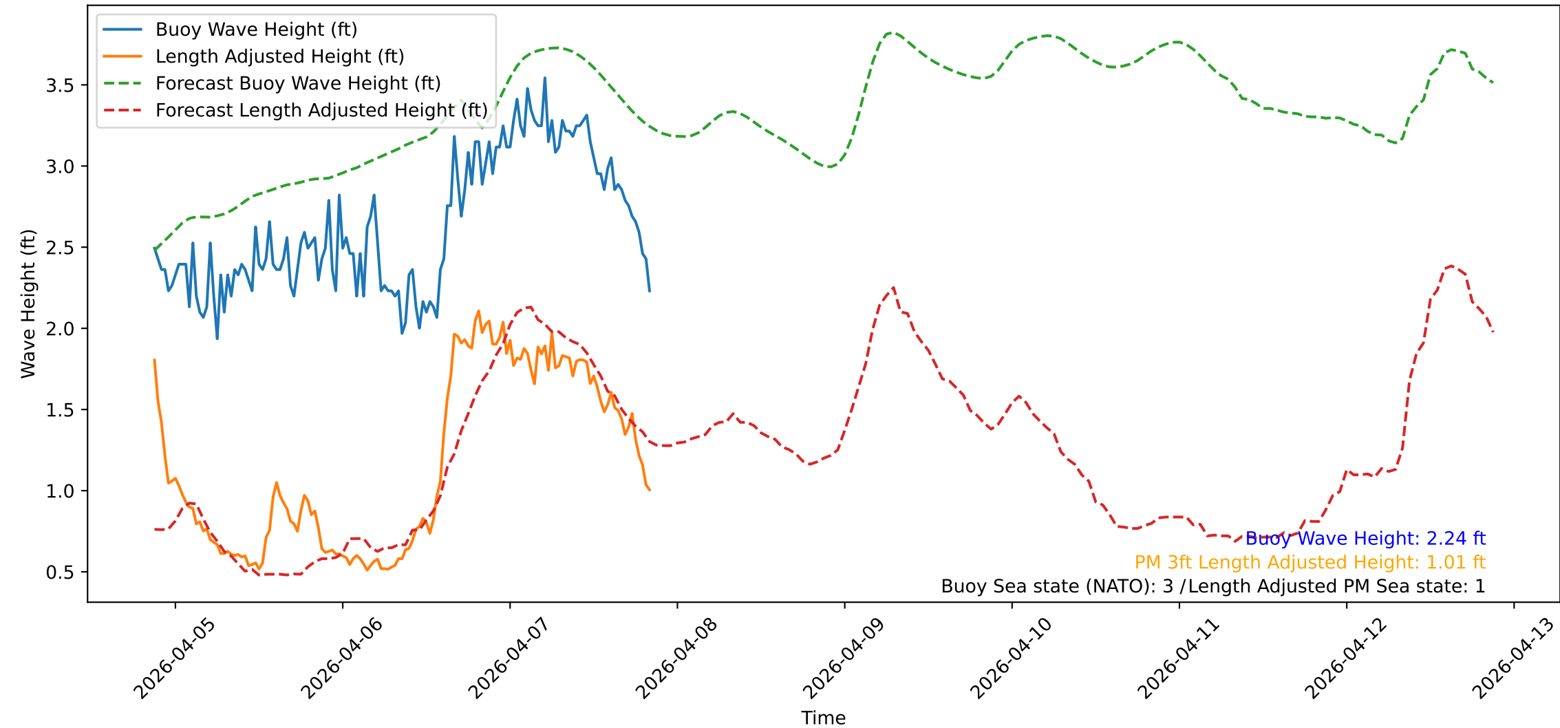
Wave Heights over Time for Red Beach at 2026-04-07 20:50:48
