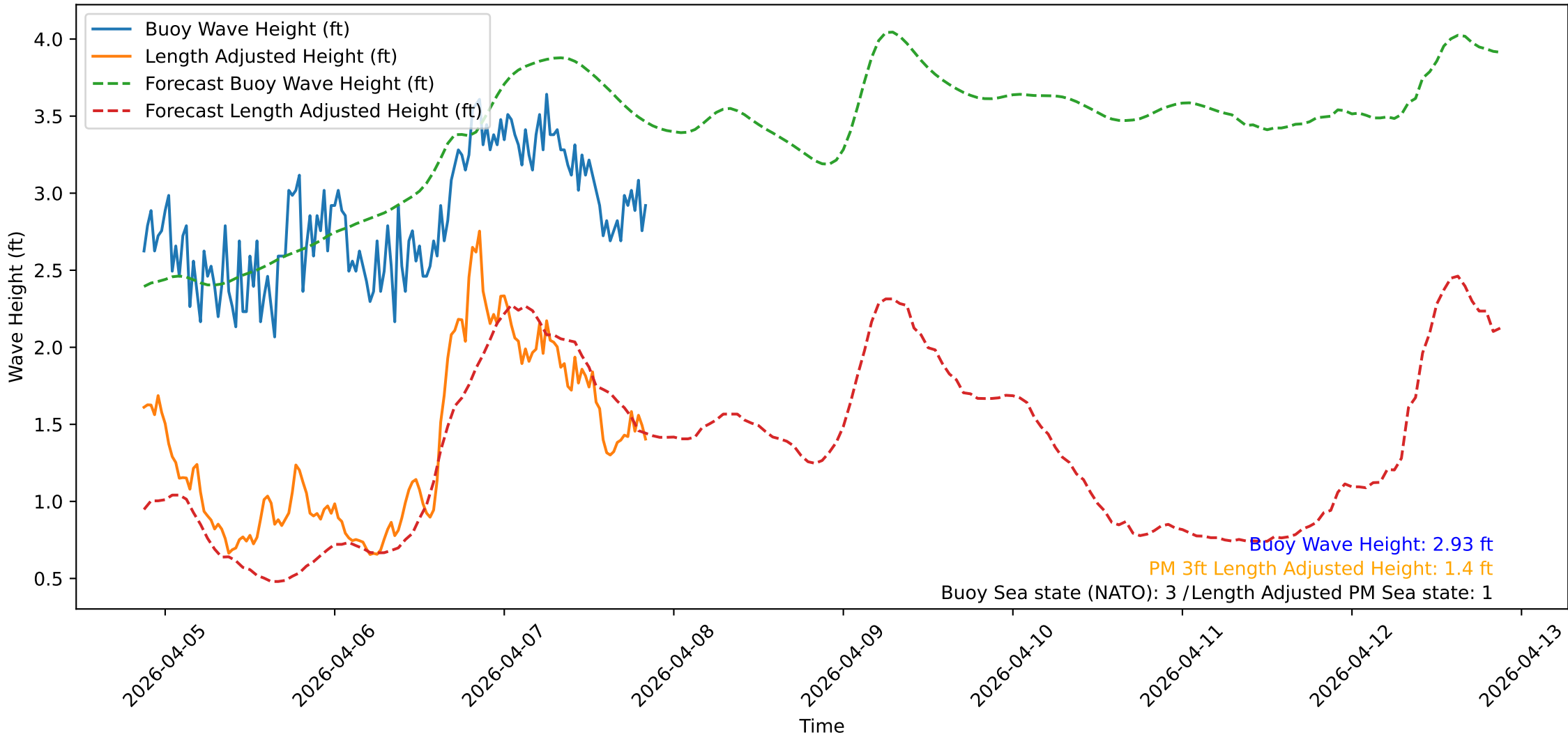
Wave Heights over Time for Oceanside Harbor at 2026-04-07 20:50:32
