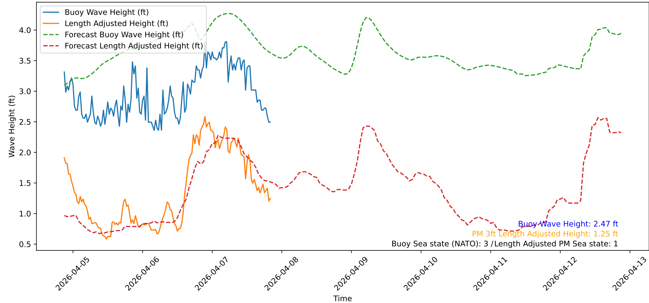
Wave Heights over Time for Green Beach at 2026-04-07 20:51:11
