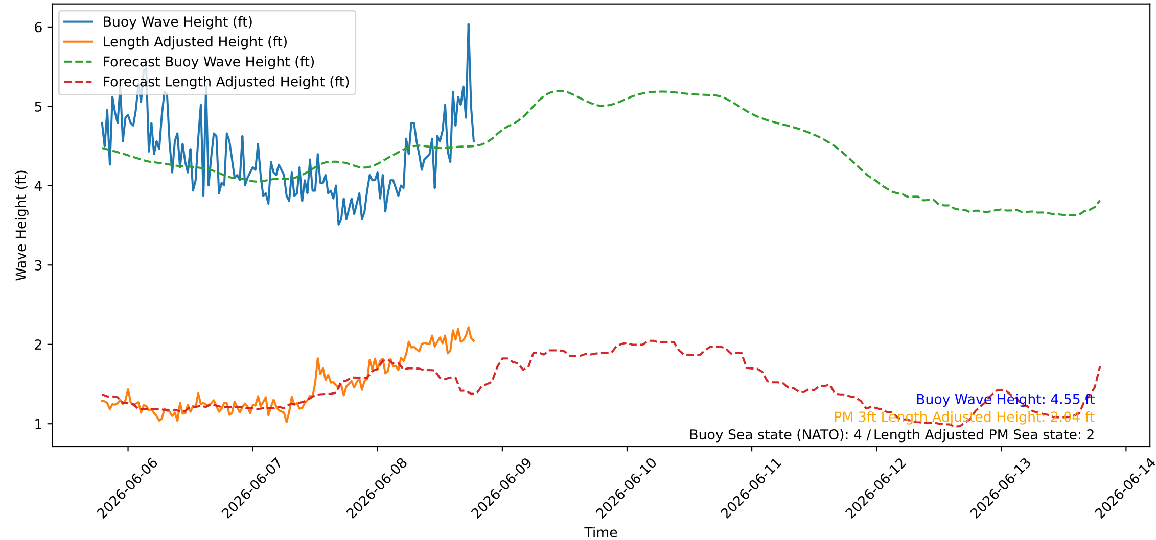
Wave Heights over Time for Oceanside Harbor at 2026-06-08 19:10:27
