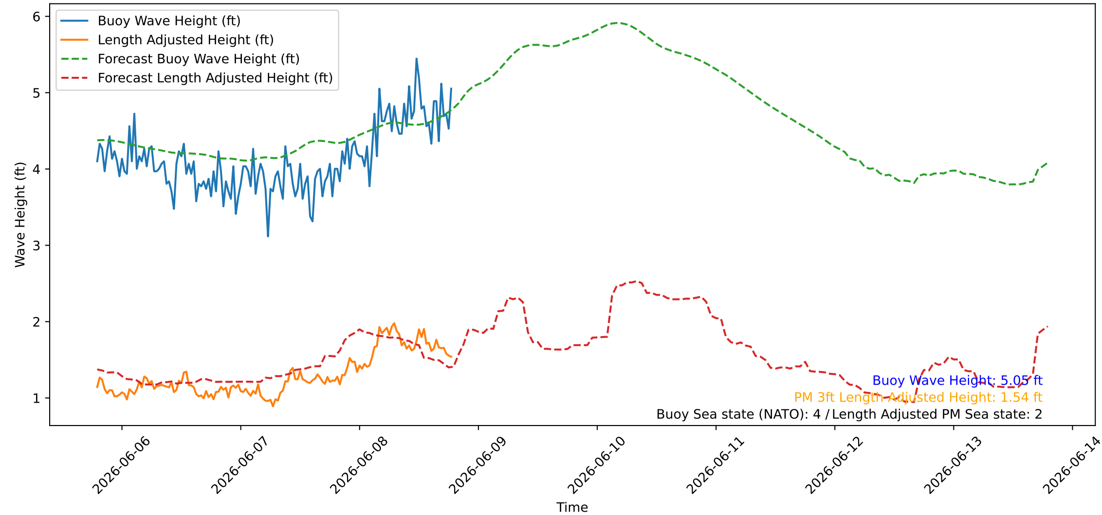
Wave Heights over Time for Green Beach at 2026-06-08 19:11:09
