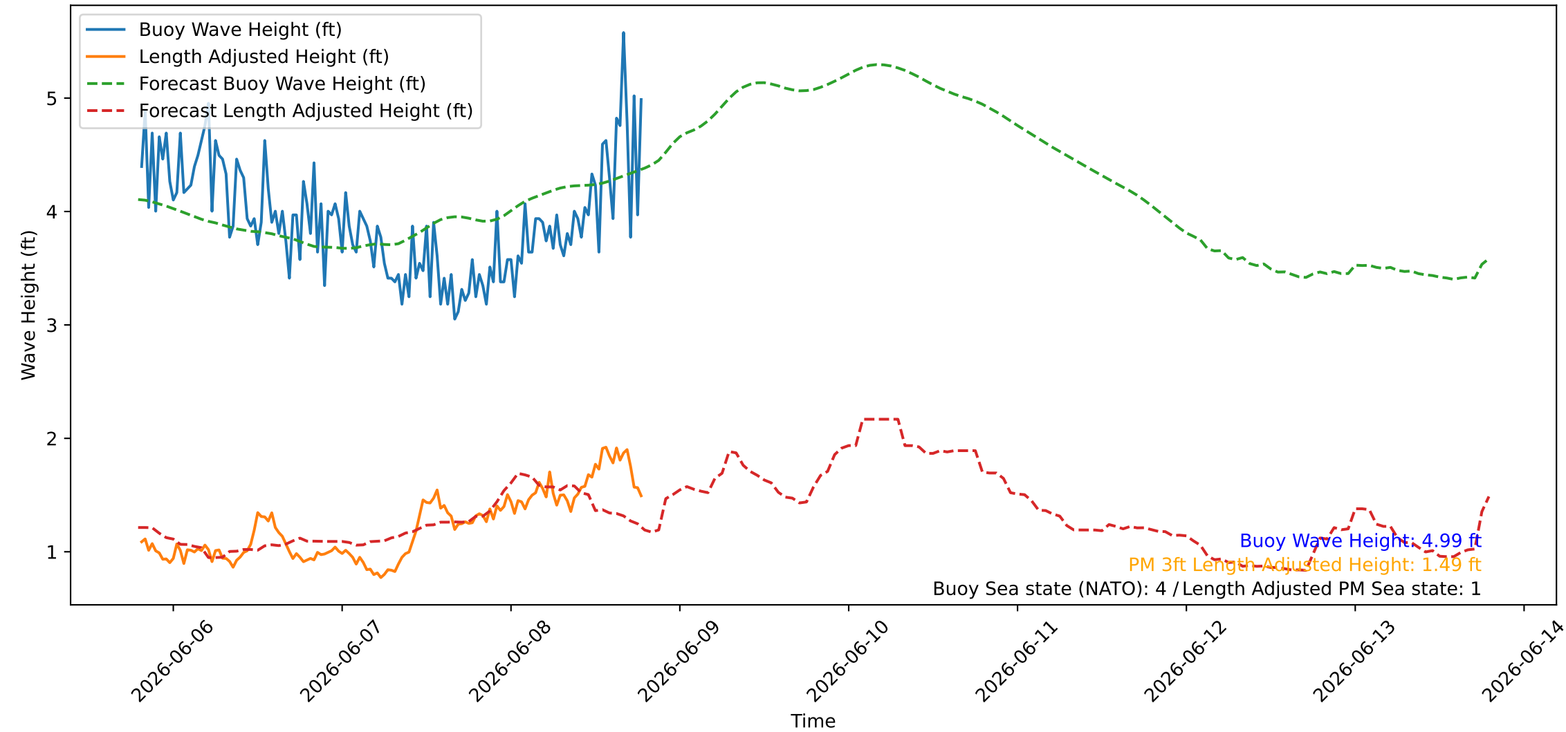
Wave Heights over Time for Red Beach at 2026-06-08 19:10:46
