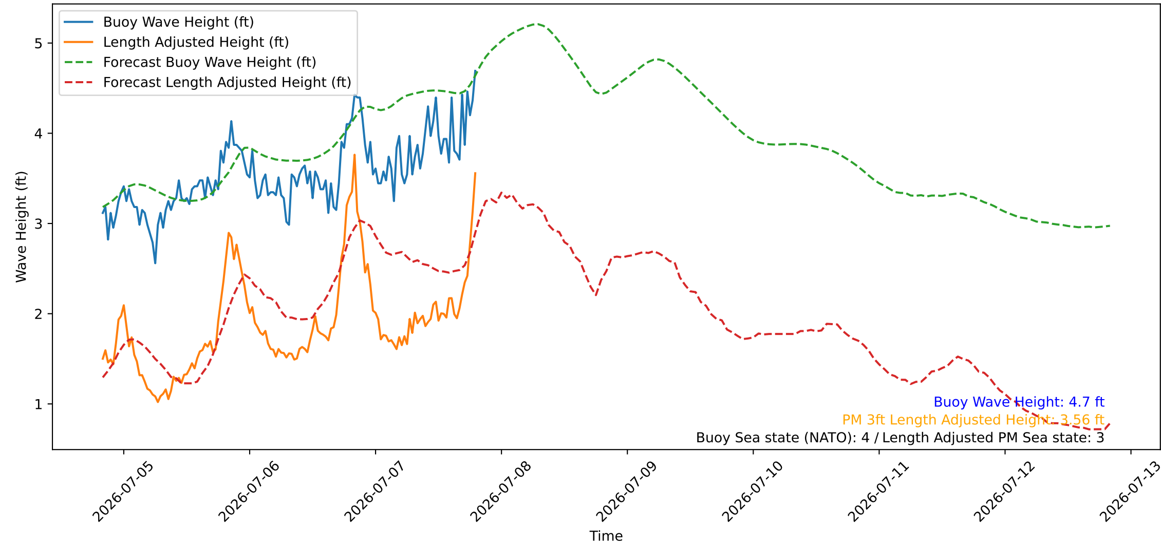
Wave Heights over Time for Green Beach at 2026-07-07 20:01:09
