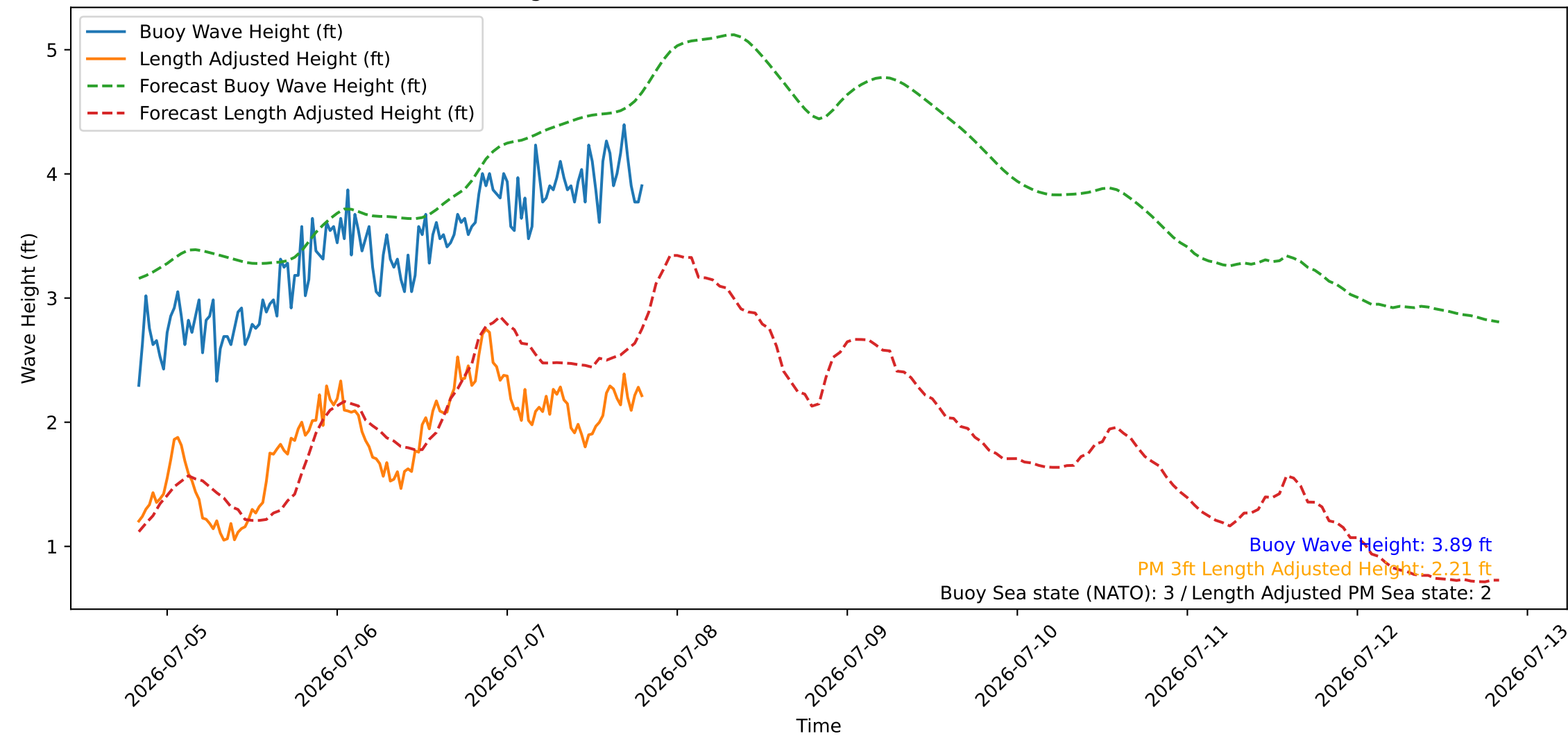
Wave Heights over Time for Oceanside Harbor at 2026-07-07 20:00:27
