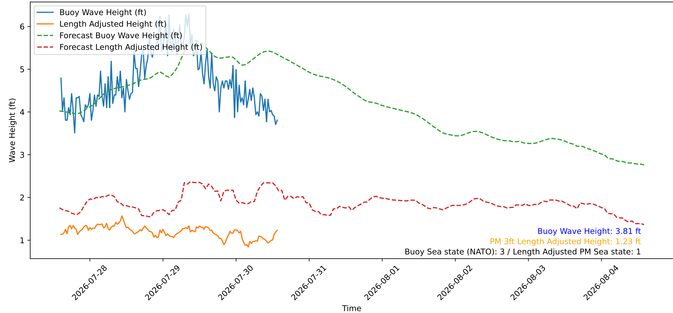
Wave Heights over Time for Green Beach at 2026-07-30 14:21:09
