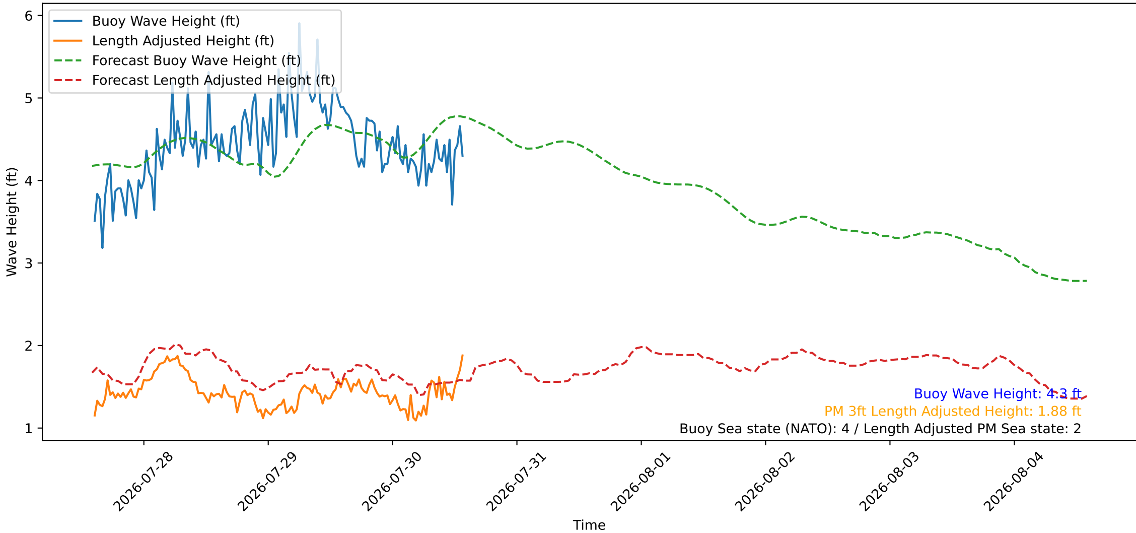
Wave Heights over Time for Oceanside Harbor at 2026-07-30 14:20:26
