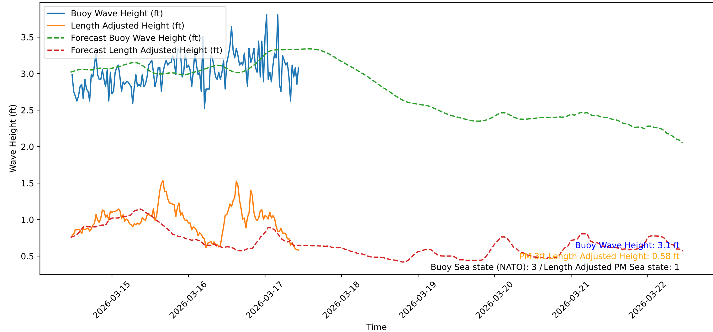
Wave Heights over Time for Red Beach at 2026-03-17 11:21:03
