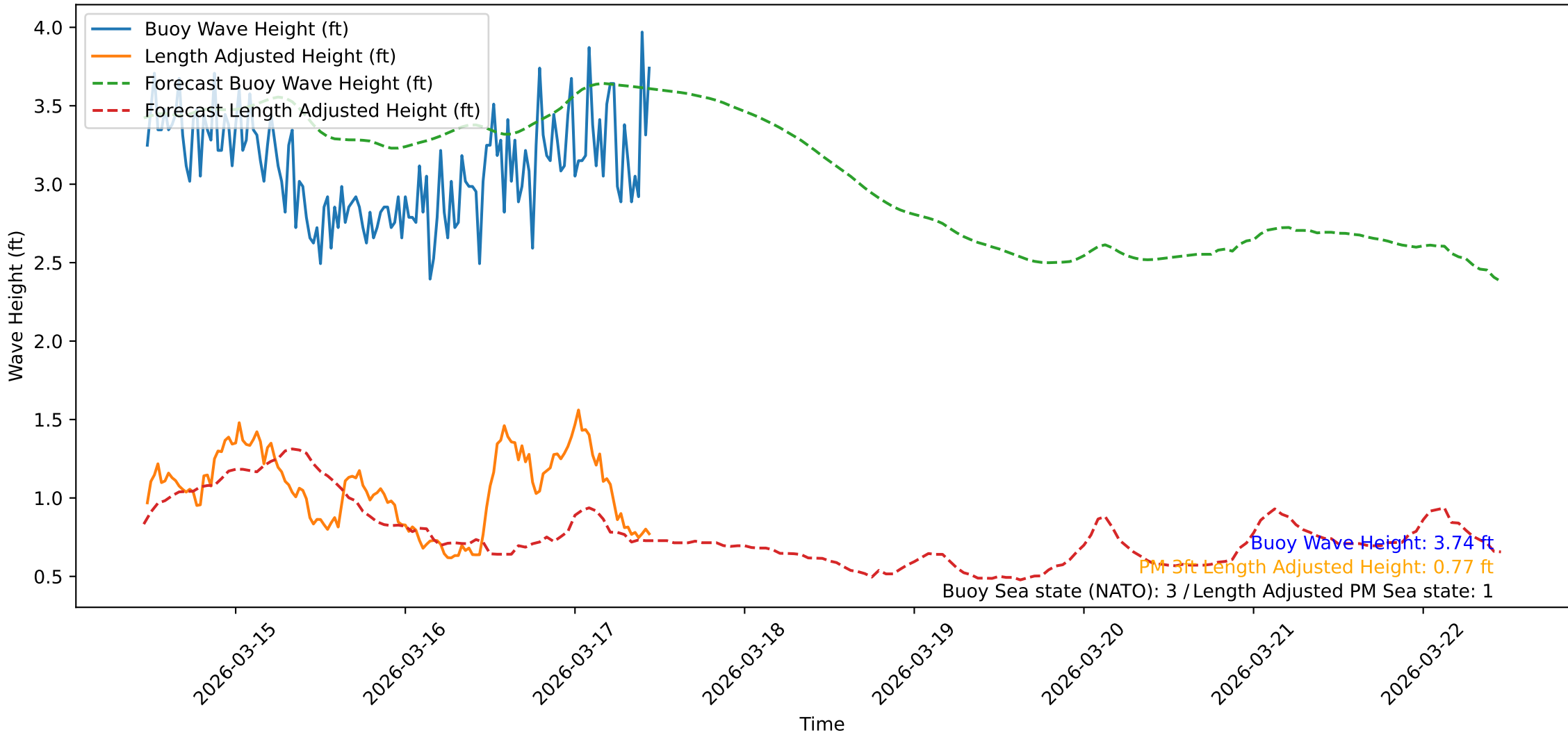
Wave Heights over Time for Oceanside Harbor at 2026-03-17 11:20:42
