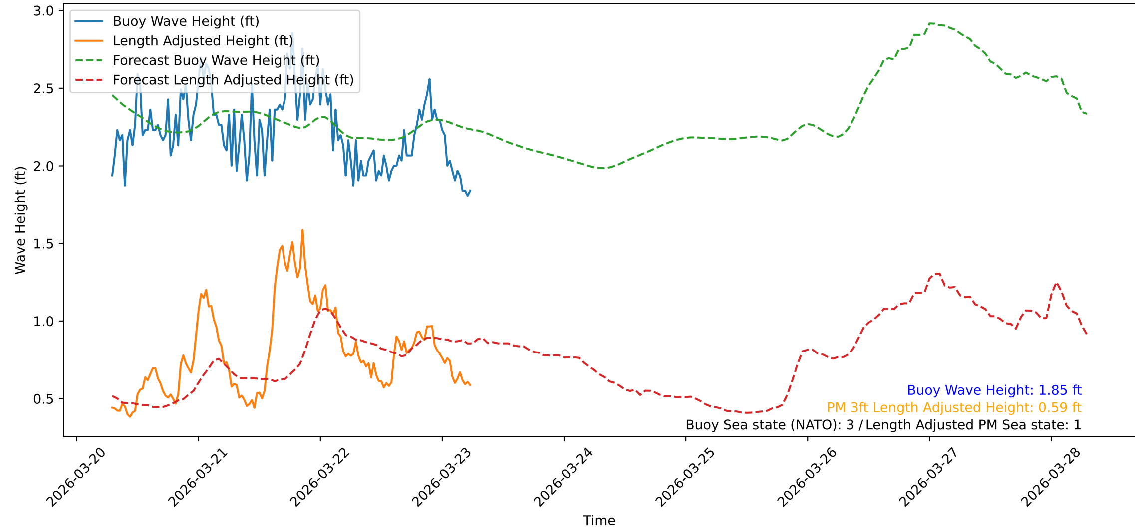
Wave Heights over Time for Red Beach at 2026-03-23 06:30:48
