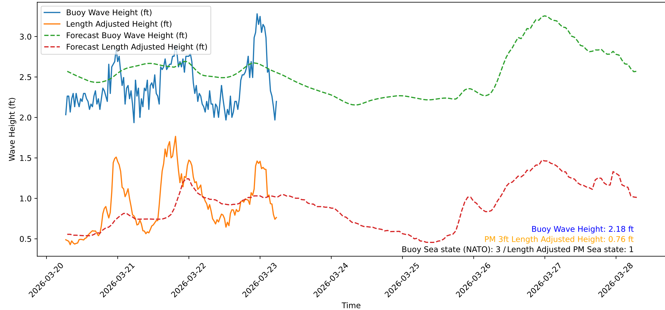
Wave Heights over Time for Green Beach at 2026-03-23 06:31:11
