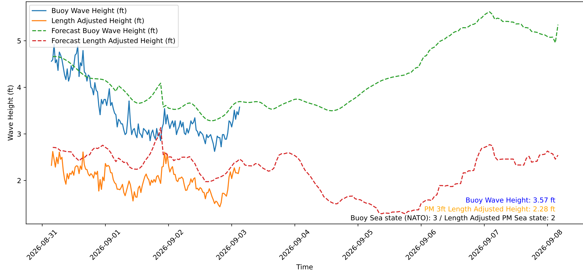
Wave Heights over Time for Oceanside Harbor at 2026-09-03 03:40:29
