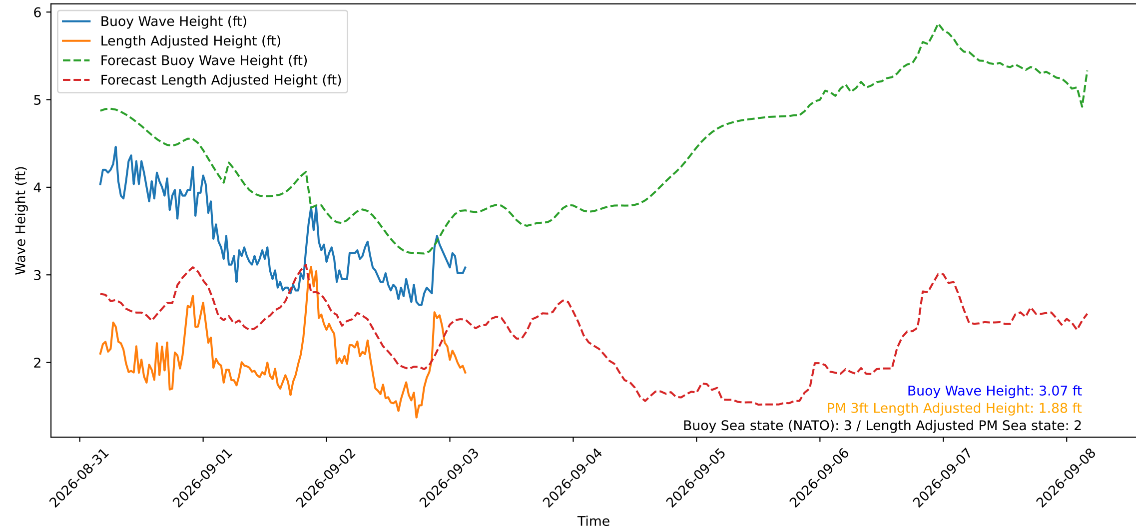
Wave Heights over Time for Green Beach at 2026-09-03 03:41:11
