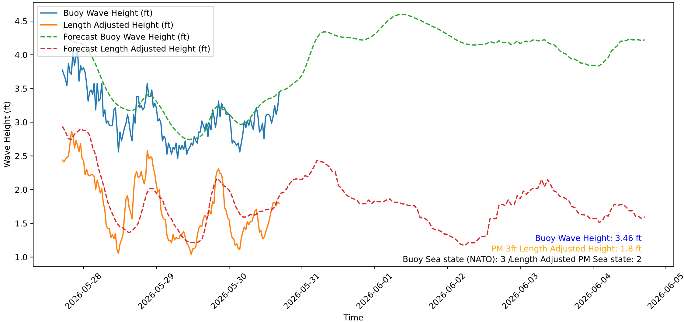
Wave Heights over Time for Green Beach at 2026-05-30 17:11:06
