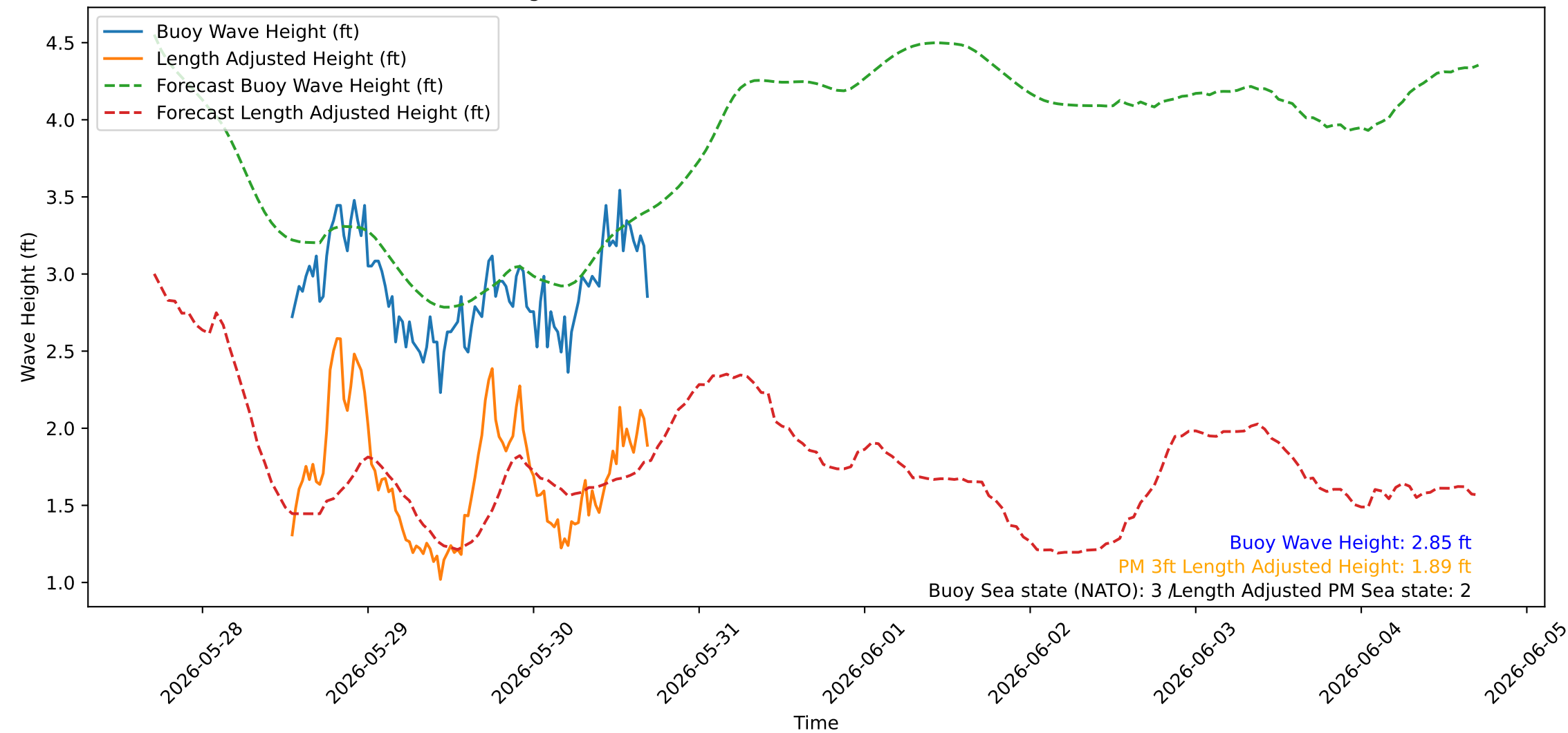
Wave Heights over Time for Oceanside Harbor at 2026-05-30 17:10:23
