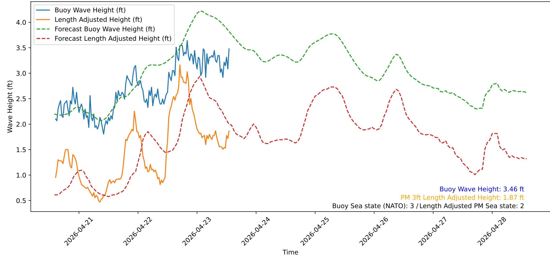
Wave Heights over Time for Red Beach at 2026-04-23 14:00:50
