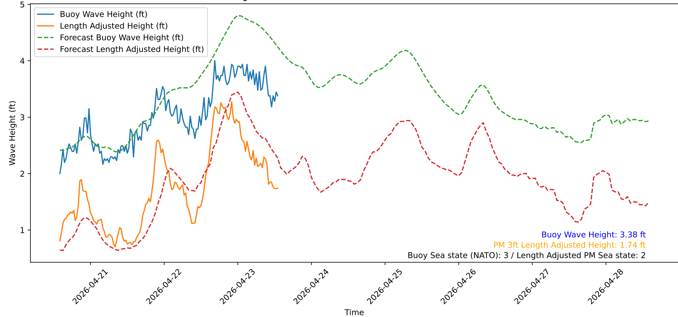
Wave Heights over Time for Green Beach at 2026-04-23 14:01:11
