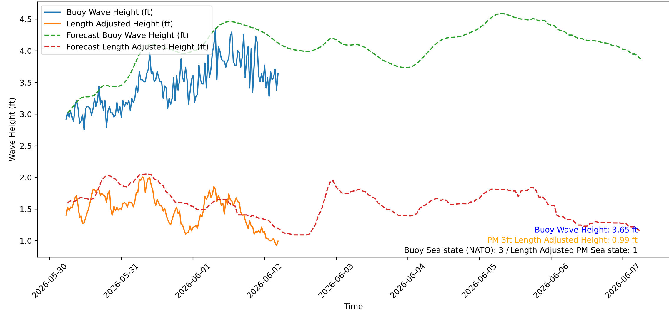
Wave Heights over Time for Green Beach at 2026-06-02 05:41:08
