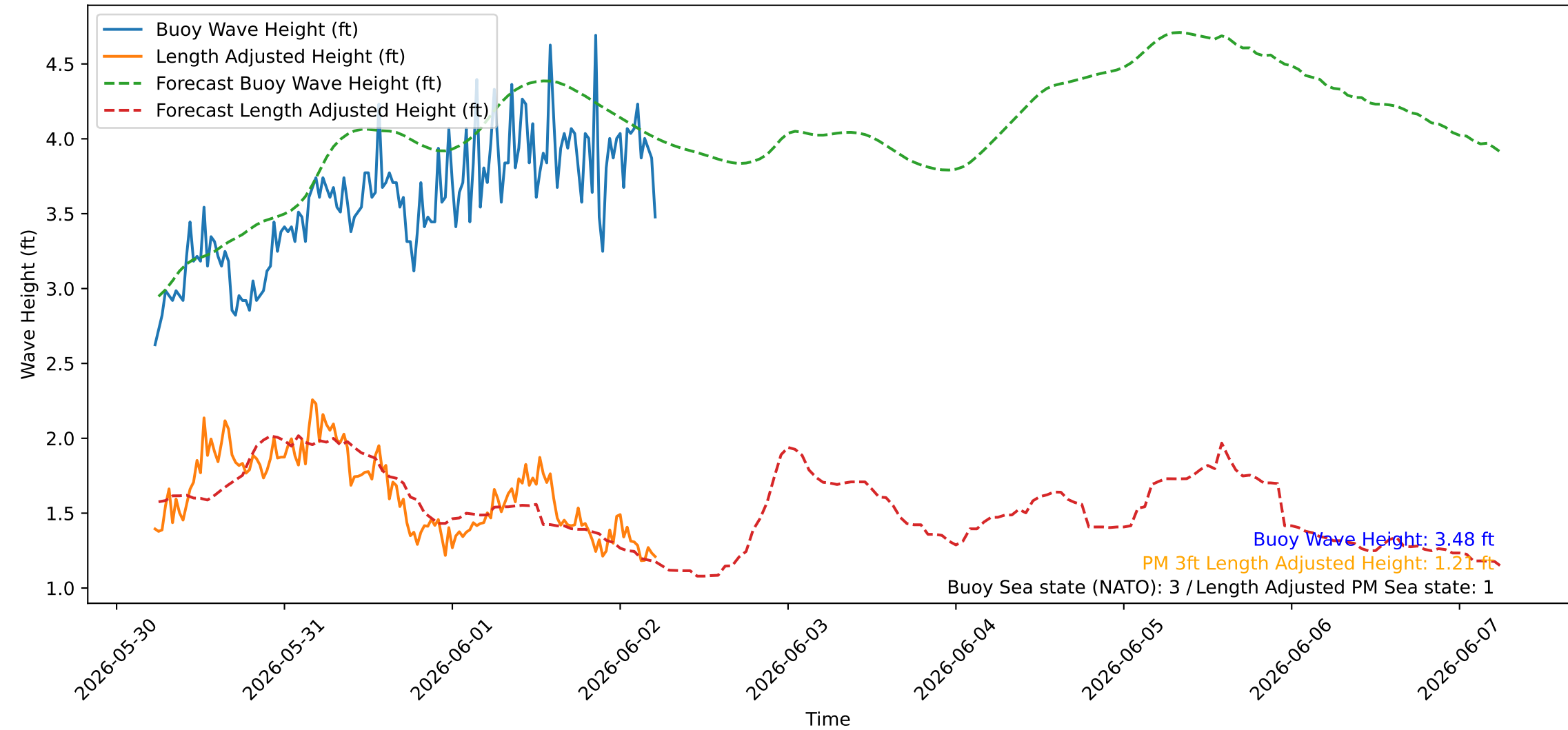
Wave Heights over Time for Oceanside Harbor at 2026-06-02 05:40:26
