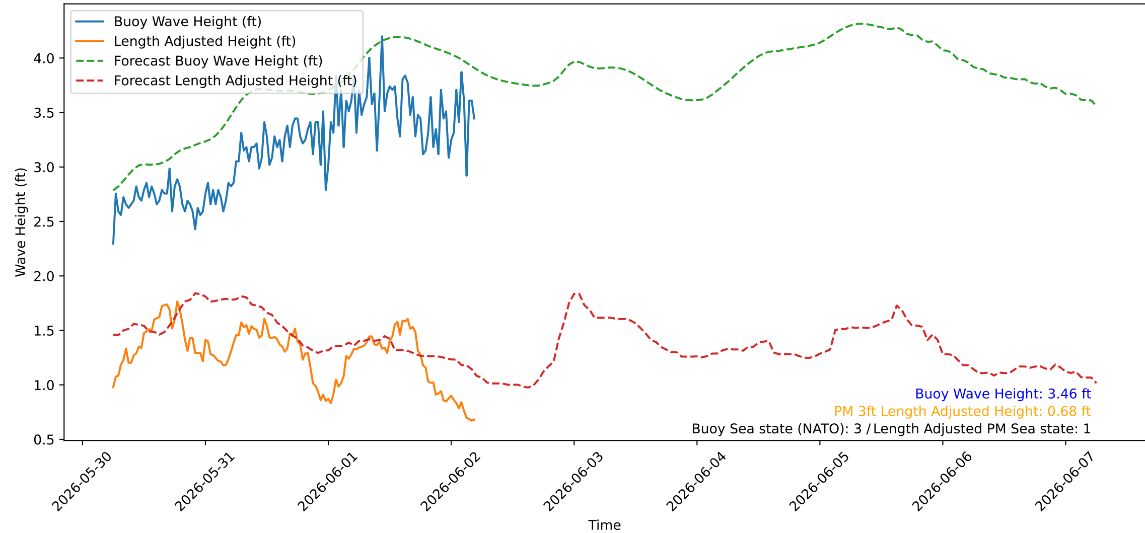
Wave Heights over Time for Red Beach at 2026-06-02 05:40:45
