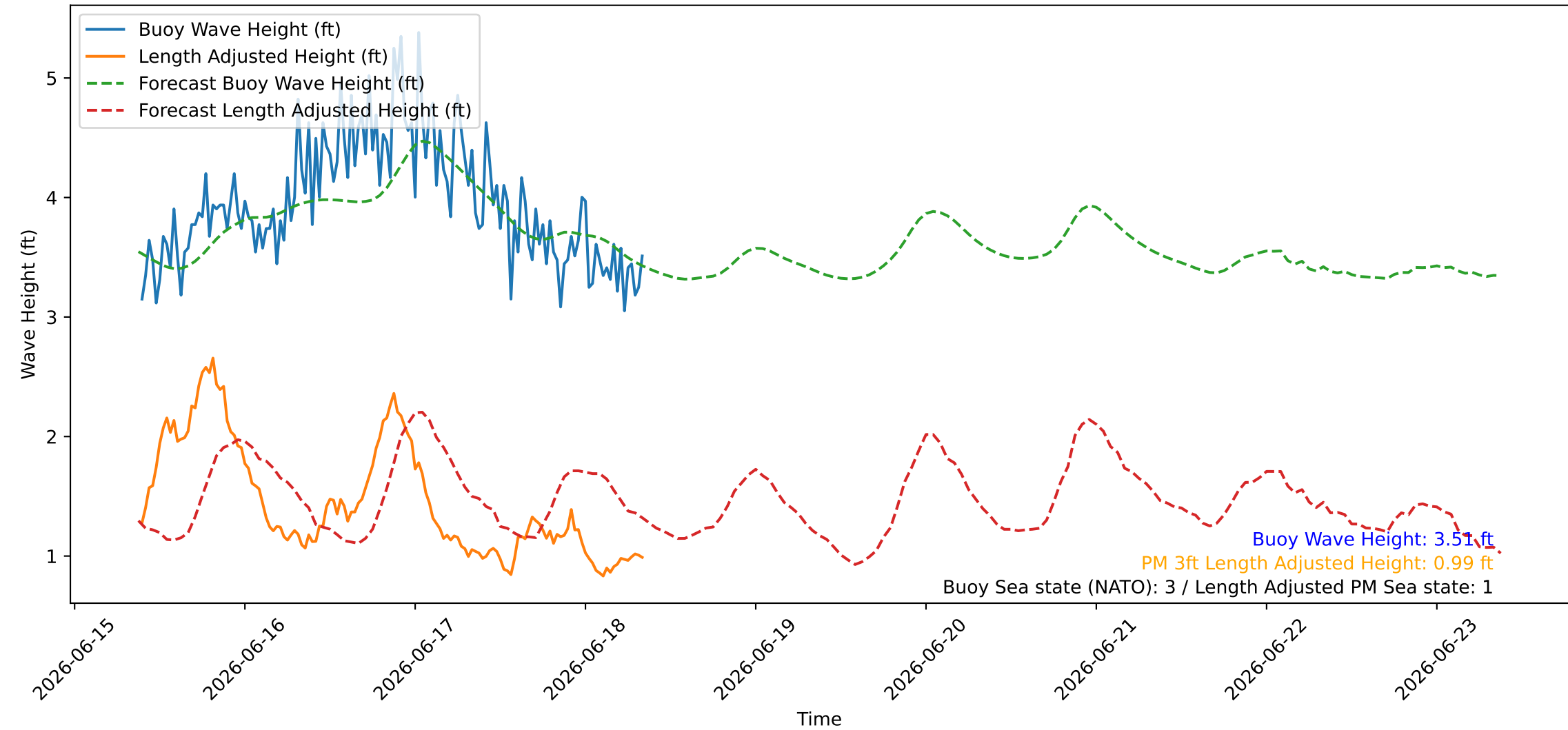
Wave Heights over Time for Red Beach at 2026-06-18 09:10:46
