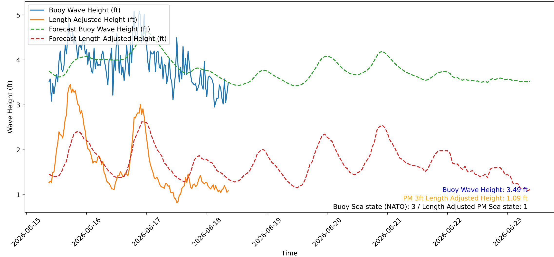
Wave Heights over Time for Green Beach at 2026-06-18 09:11:09
