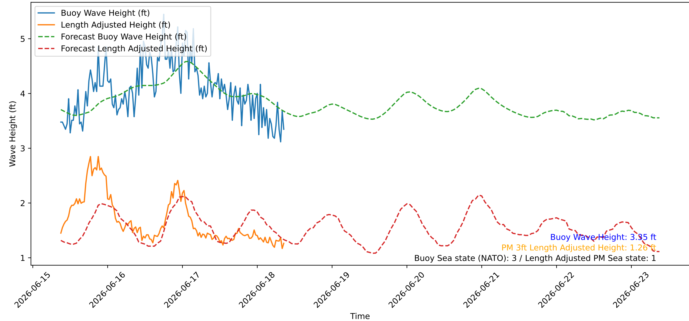
Wave Heights over Time for Oceanside Harbor at 2026-06-18 09:10:27
