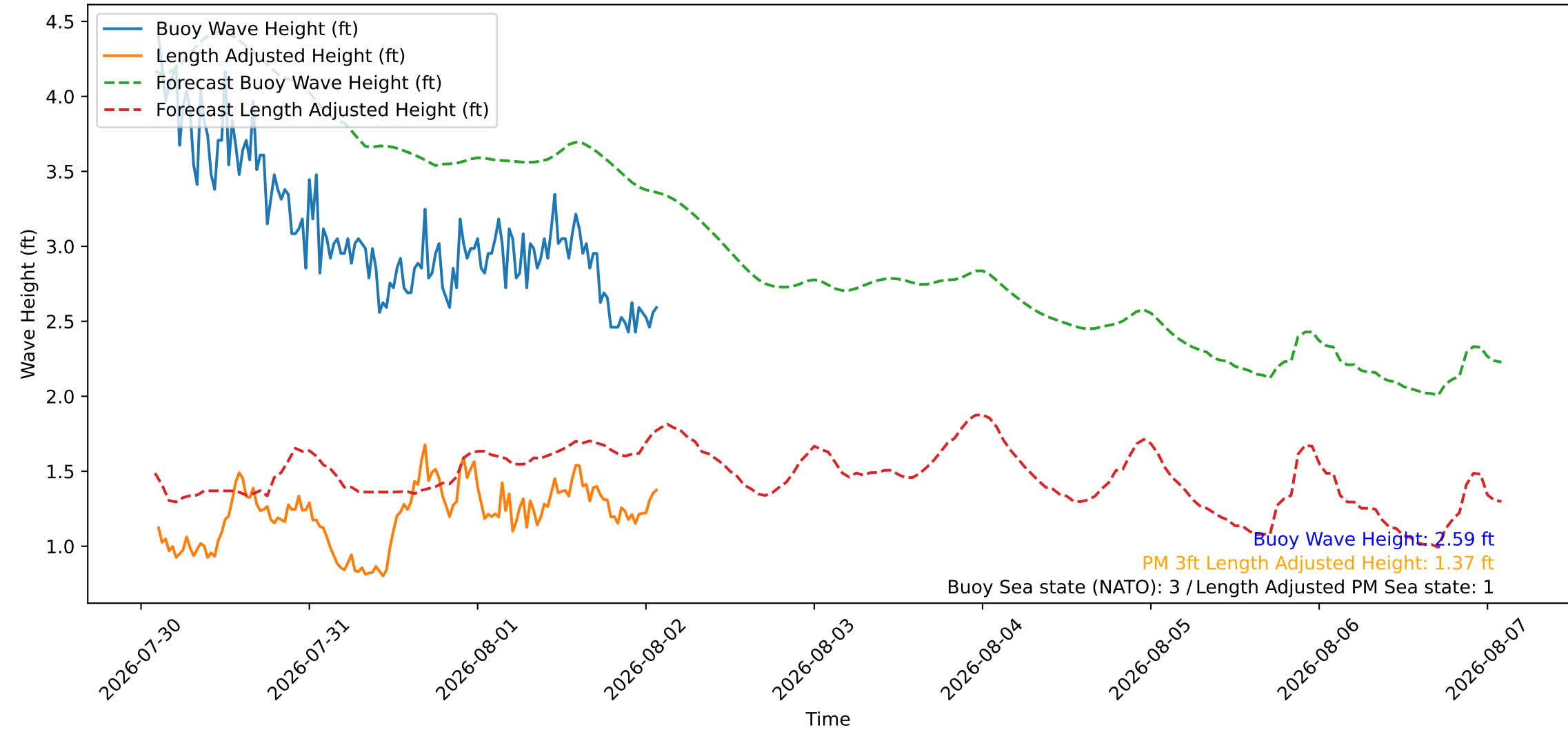
Wave Heights over Time for Red Beach at 2026-08-02 02:20:47
