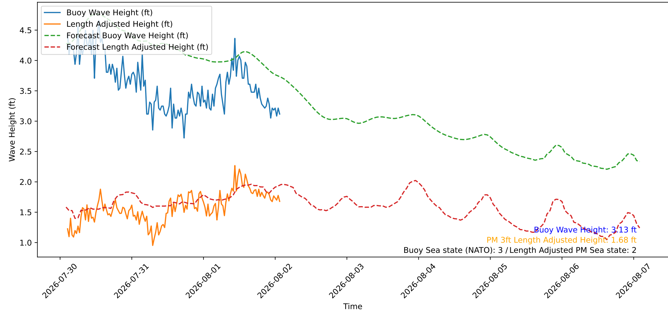
Wave Heights over Time for Oceanside Harbor at 2026-08-02 02:20:26
