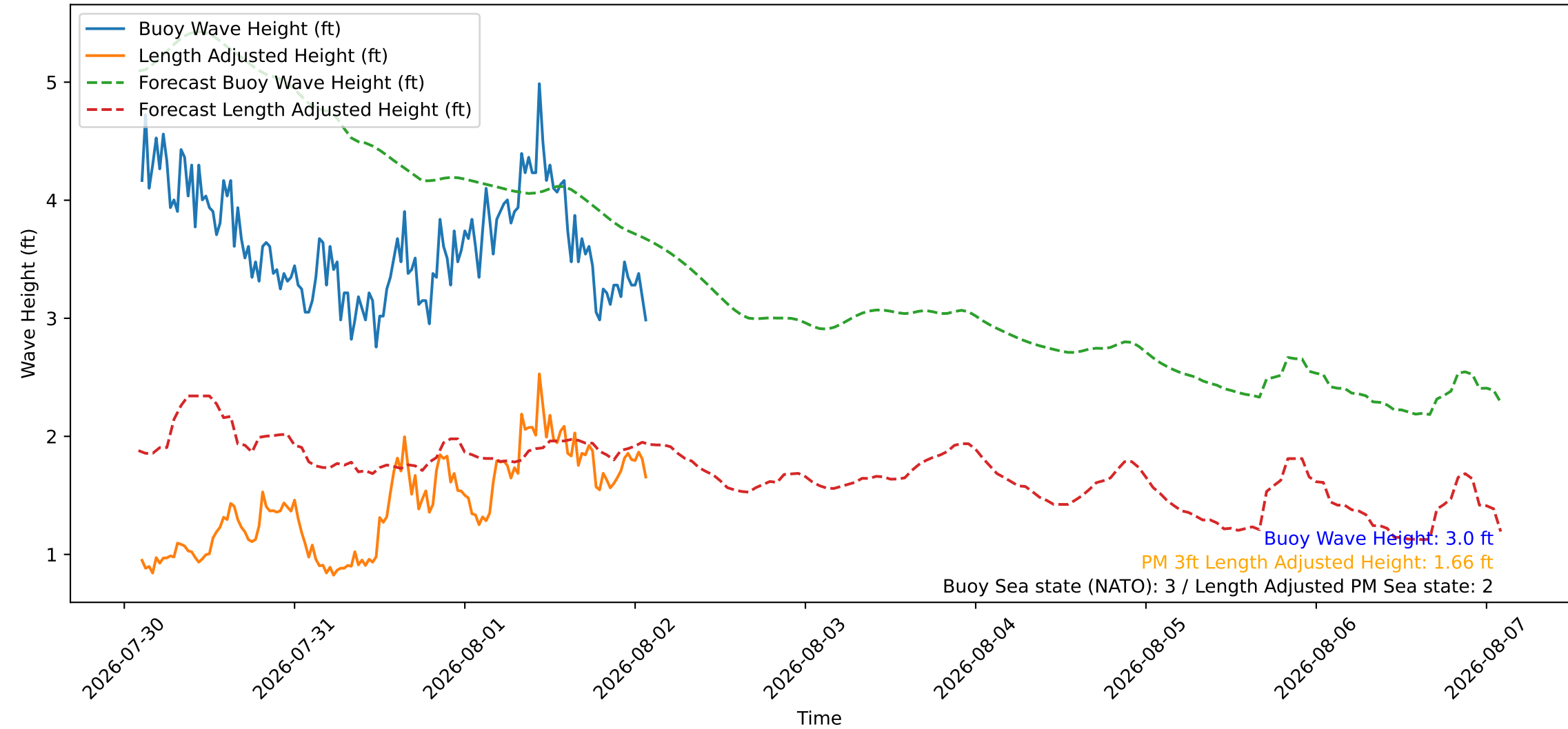
Wave Heights over Time for Green Beach at 2026-08-02 02:21:09
