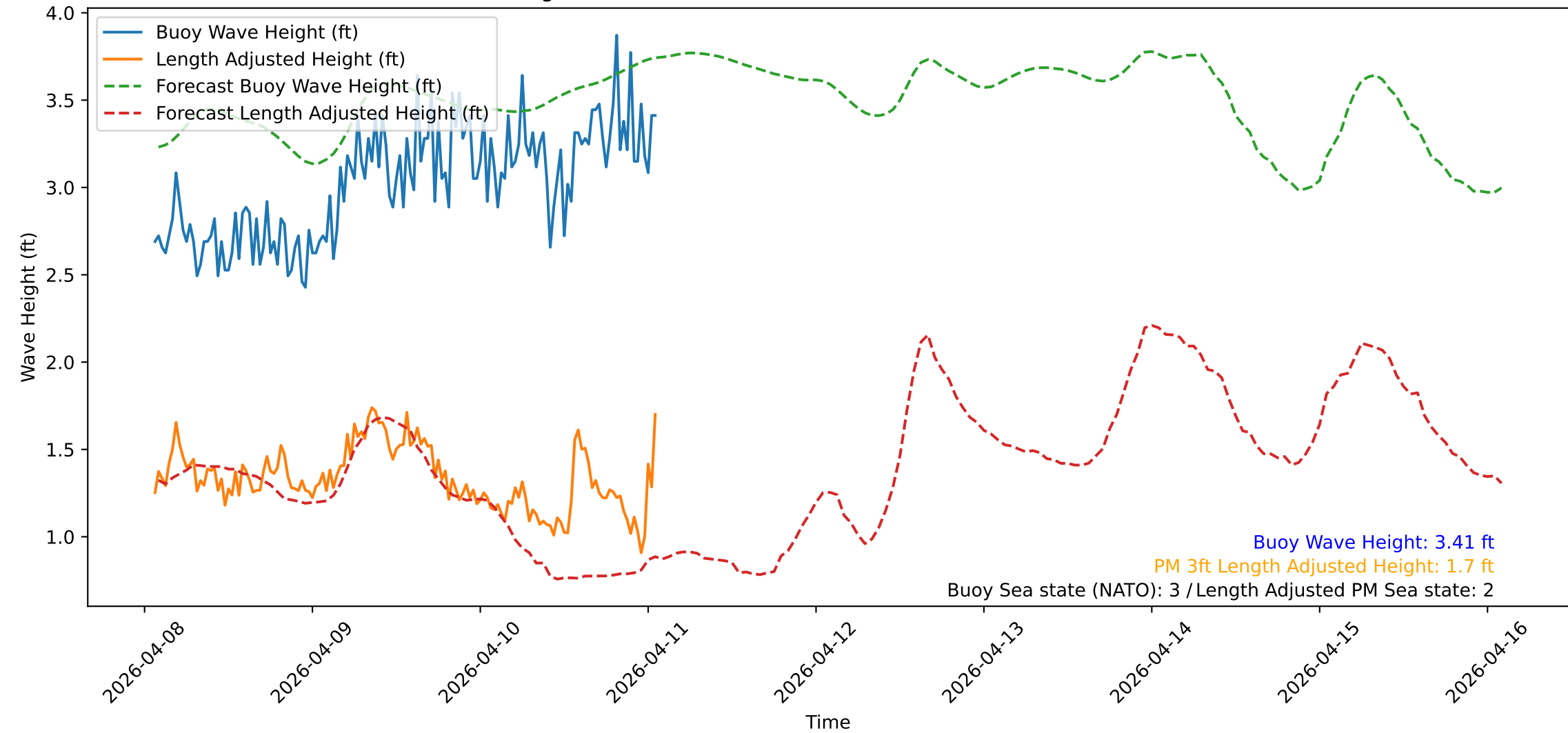
Wave Heights over Time for Oceanside Harbor at 2026-04-11 01:30:32
