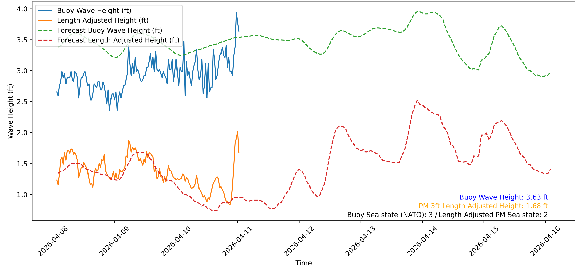
Wave Heights over Time for Green Beach at 2026-04-11 01:31:13
