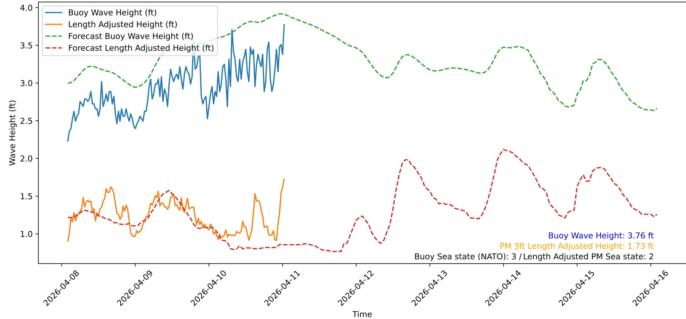
Wave Heights over Time for Red Beach at 2026-04-11 01:30:51
