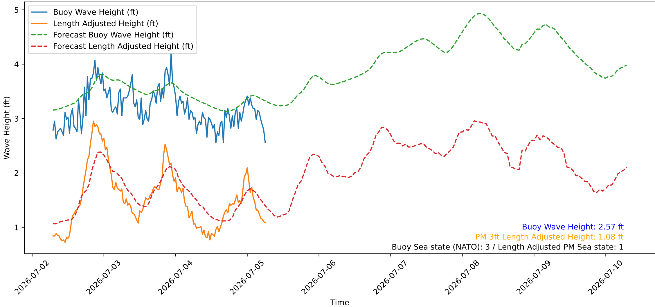
Wave Heights over Time for Green Beach at 2026-07-05 06:51:09
