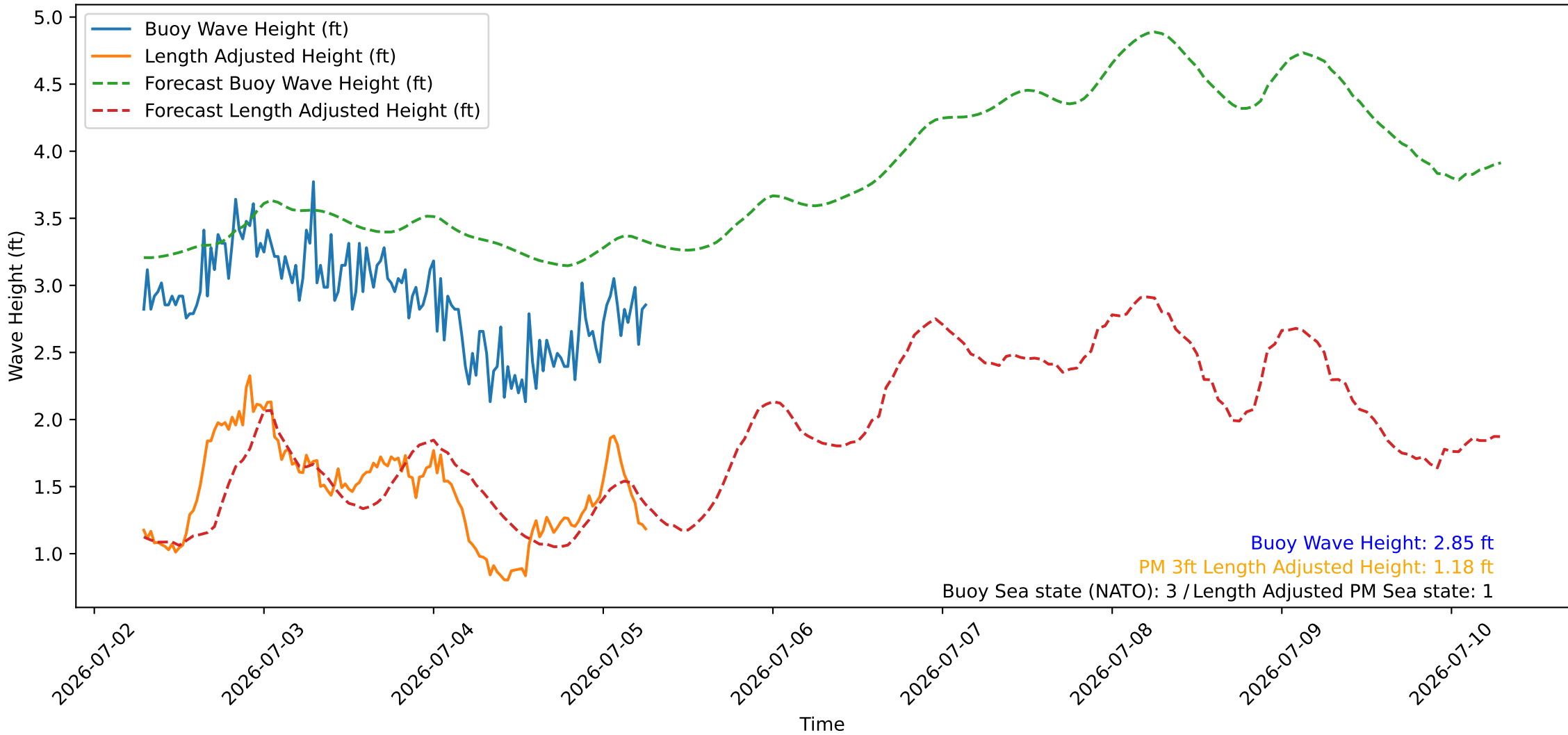
Wave Heights over Time for Oceanside Harbor at 2026-07-05 06:50:26
