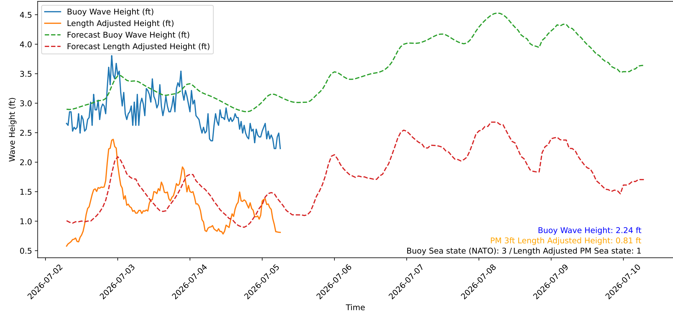
Wave Heights over Time for Red Beach at 2026-07-05 06:50:47
