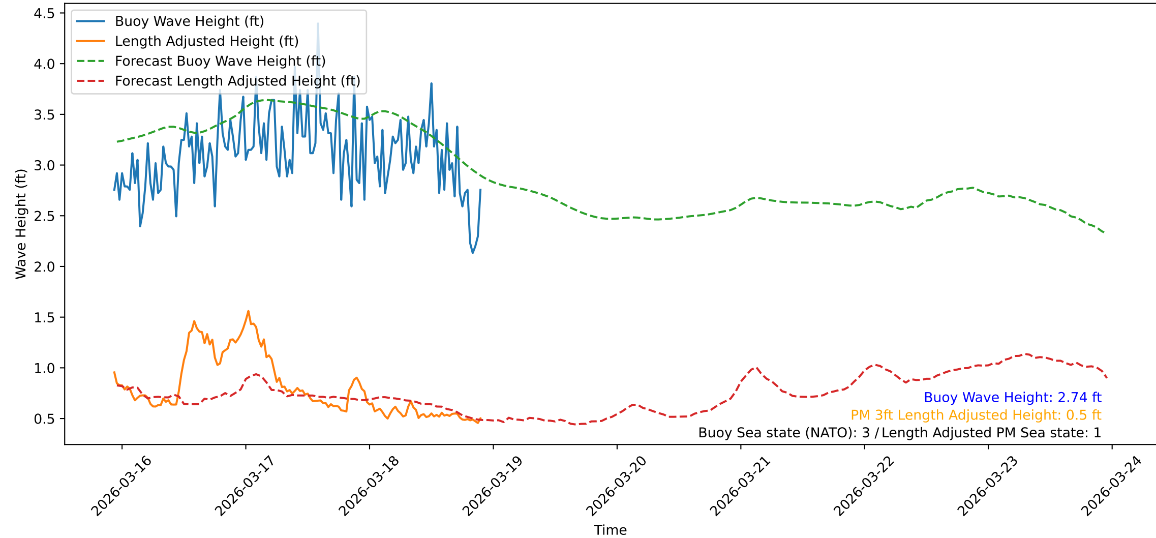
Wave Heights over Time for Oceanside Harbor at 2026-03-18 22:30:31
