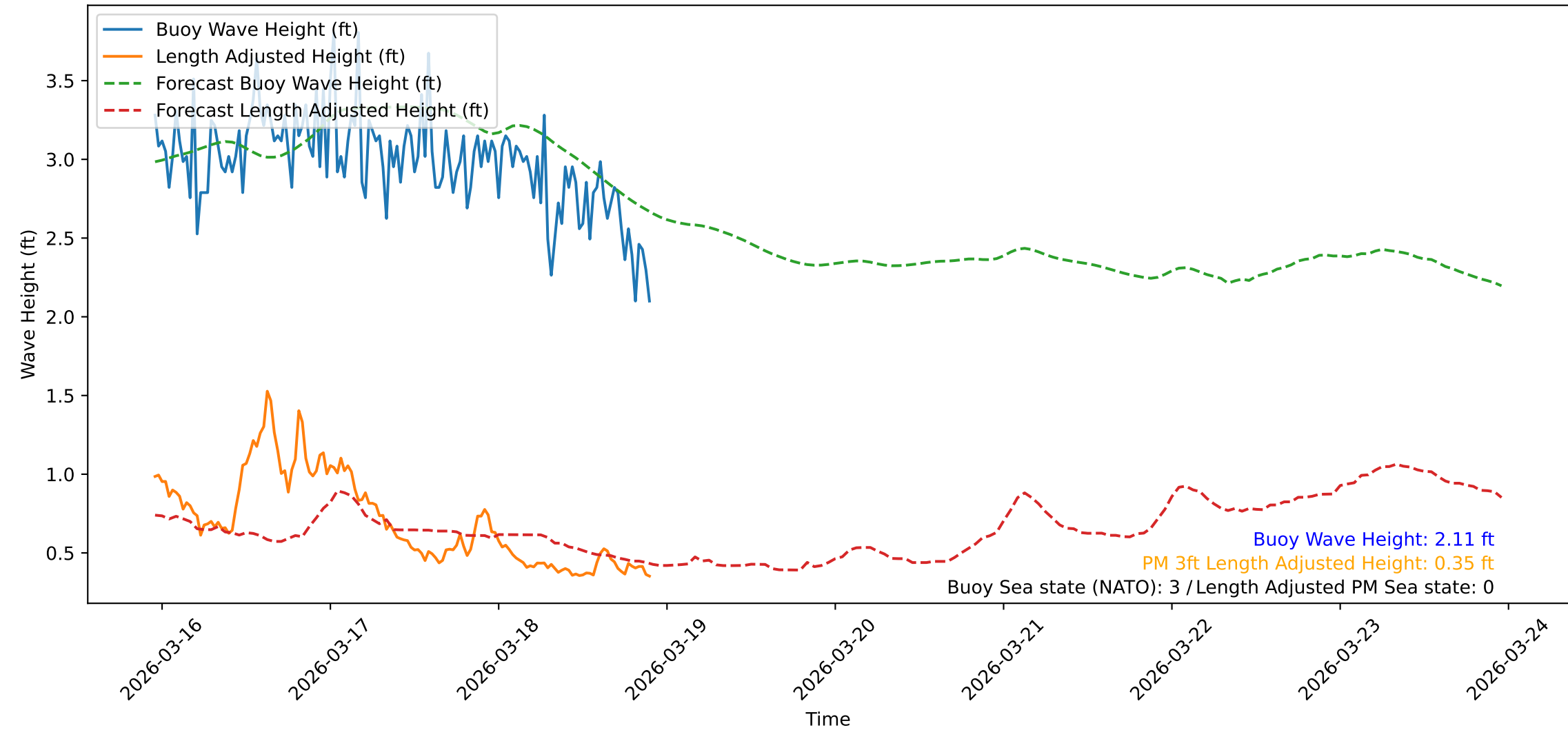
Wave Heights over Time for Red Beach at 2026-03-18 22:30:47
