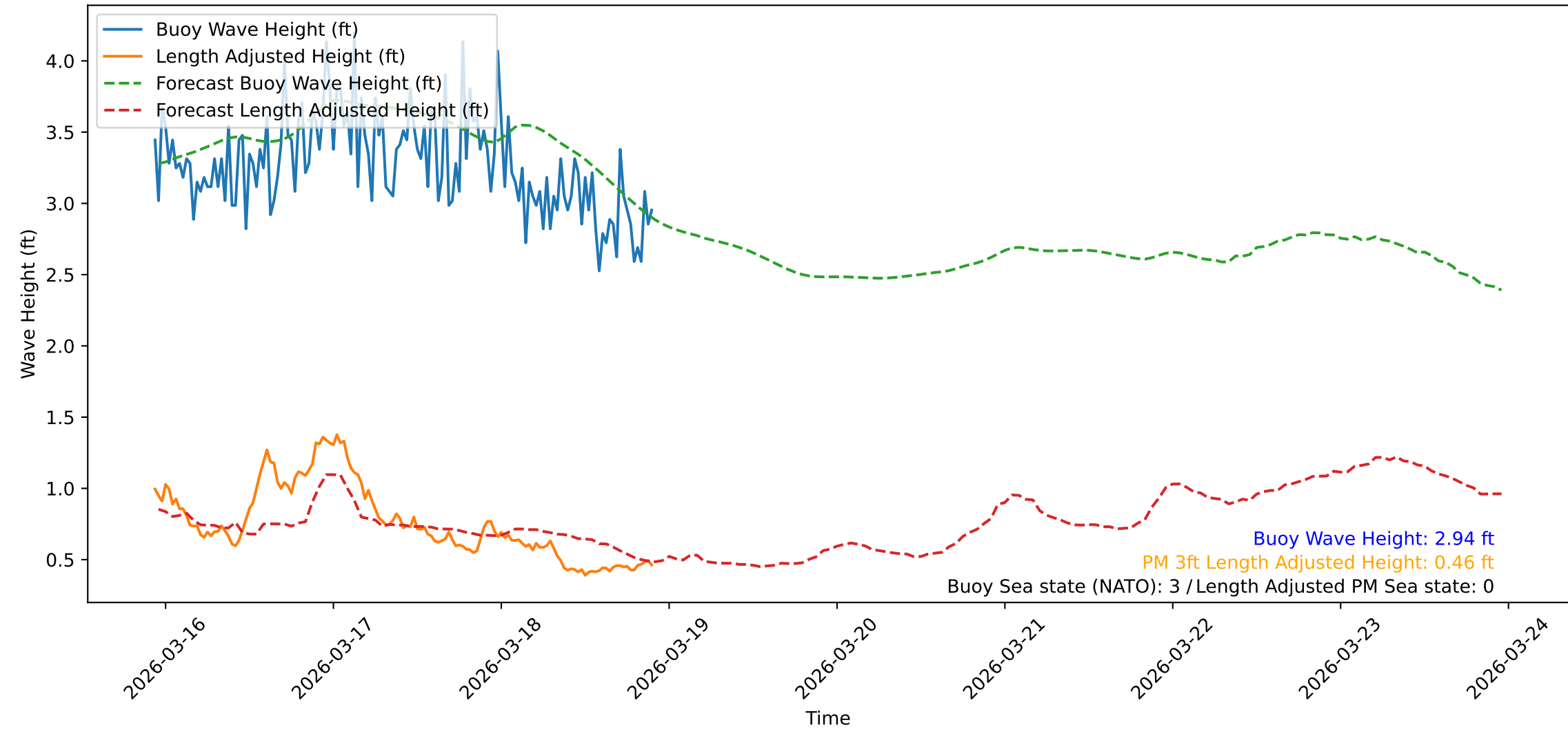
Wave Heights over Time for Green Beach at 2026-03-18 22:31:09
