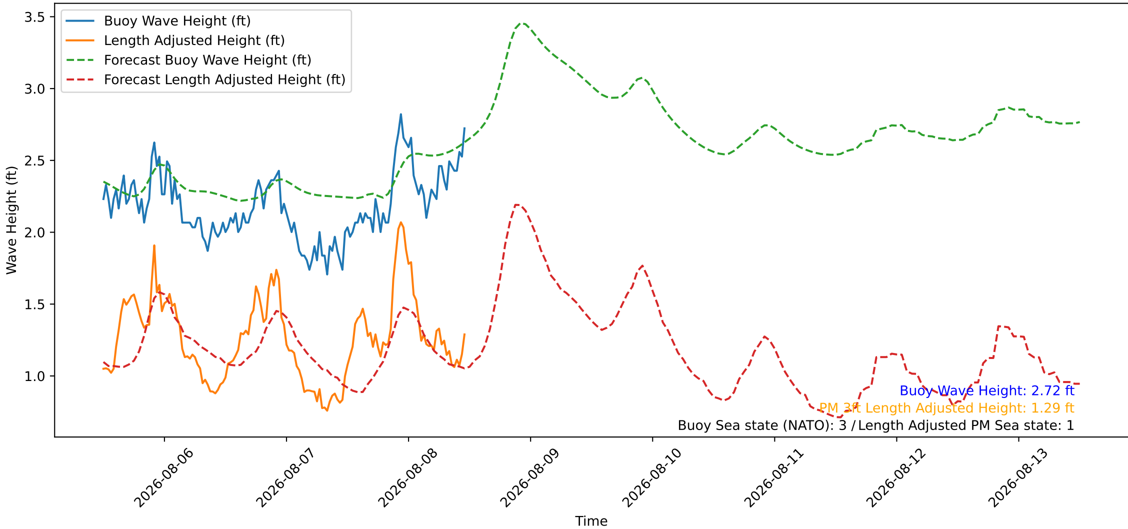
Wave Heights over Time for Green Beach at 2026-08-08 11:51:09
