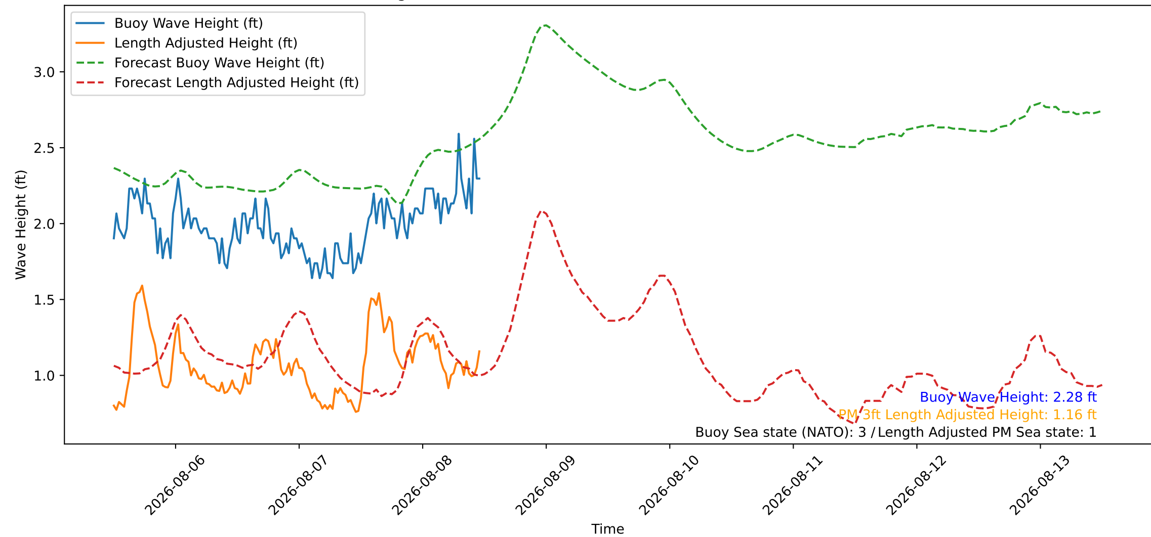
Wave Heights over Time for Oceanside Harbor at 2026-08-08 11:50:26
