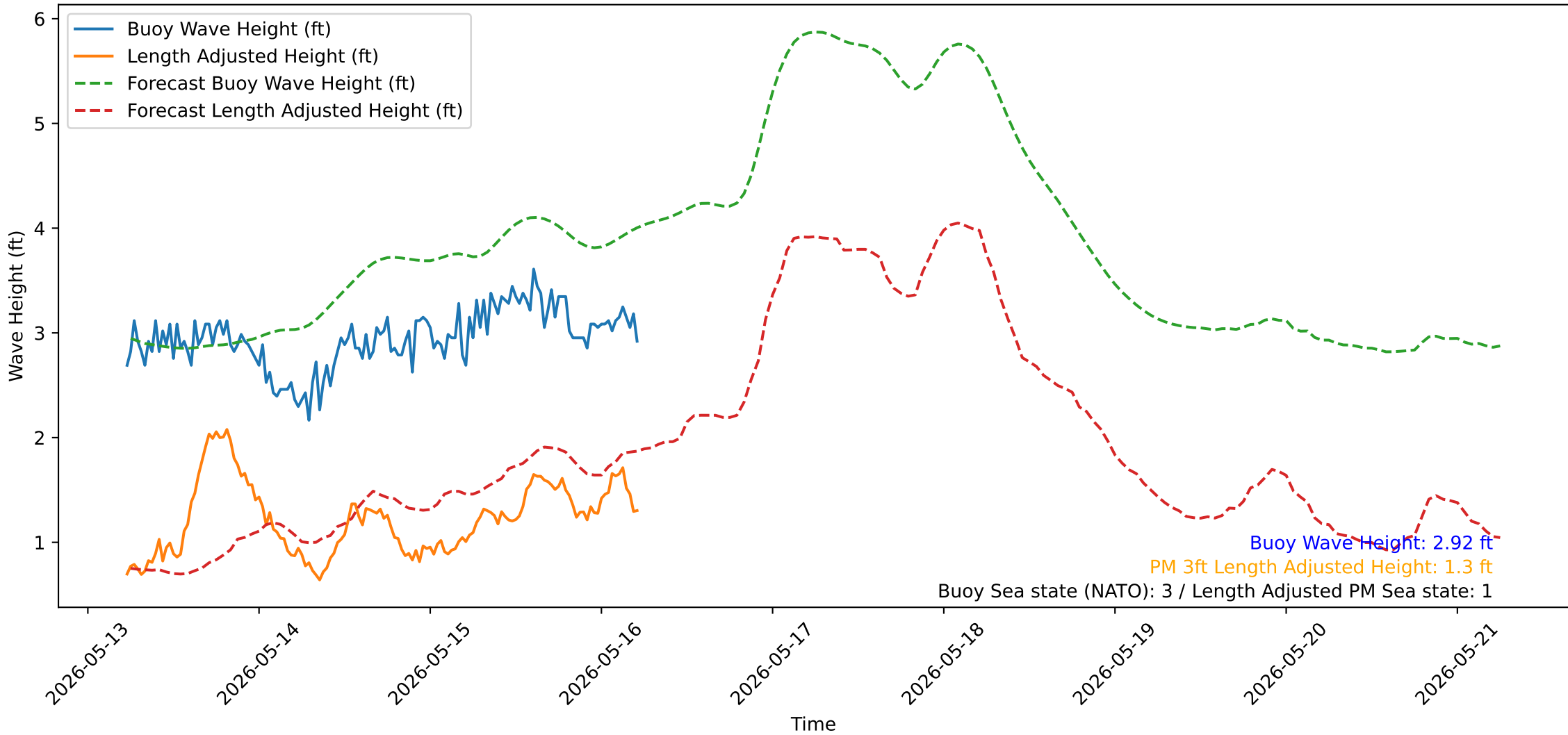
Wave Heights over Time for Oceanside Harbor at 2026-05-16 05:30:32
