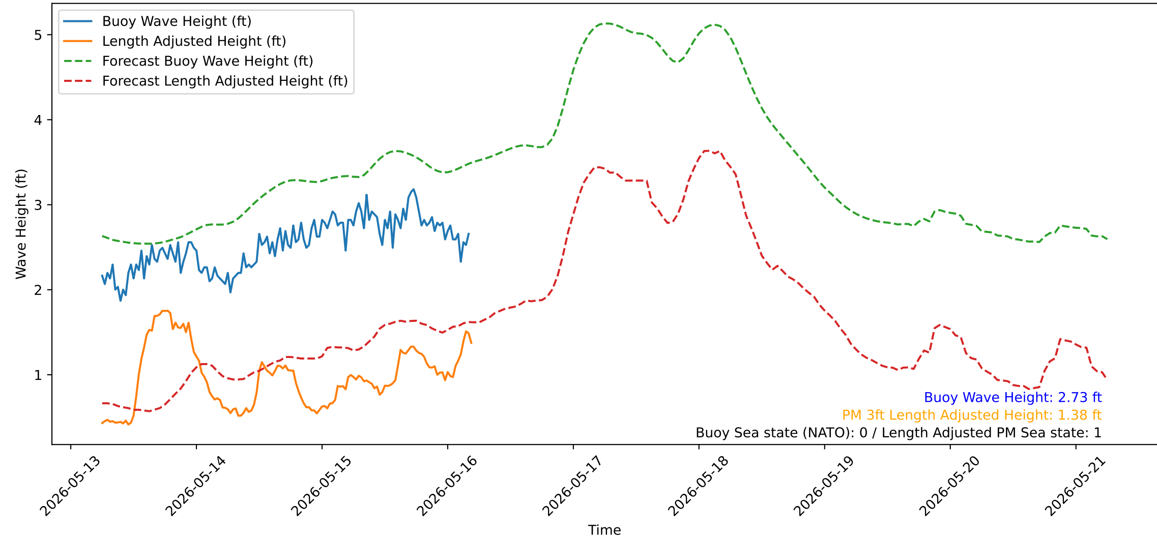
Wave Heights over Time for Red Beach at 2026-05-16 05:30:51
