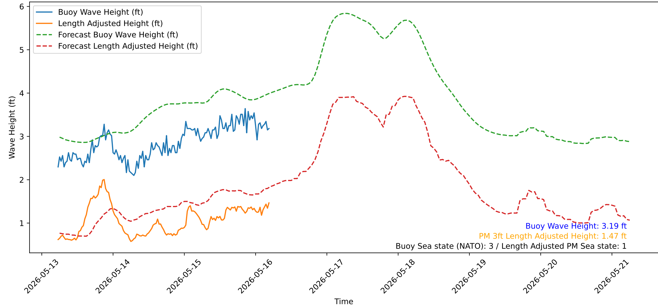
Wave Heights over Time for Green Beach at 2026-05-16 05:31:14
